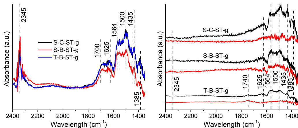
Figure 7. (Left) FTIR spectra at 5 Torr of CO 2 ; (Right) Spectra acquired at 50 °C (black) and 100 °C (red).
