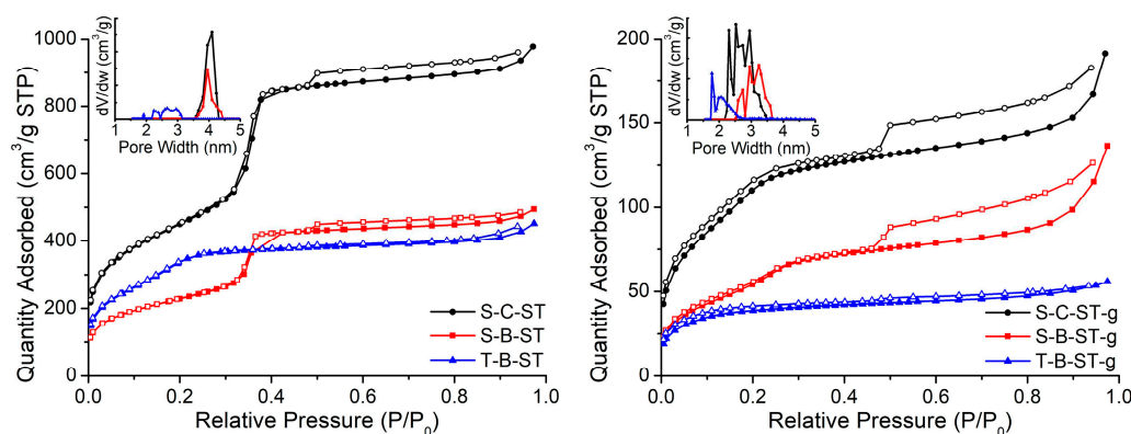
Figure 5. N 2 adsorption (solid symbols) and desorption (open symbols) isotherms of as-made ( left ) and amine-modified ( right ) MCM-41.
