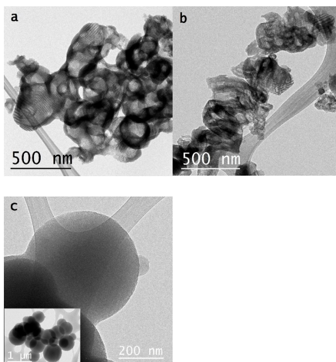
Figure 3. TEM images of samples S-C-ST (a), S-B-ST (b), and T-B-ST (c).
