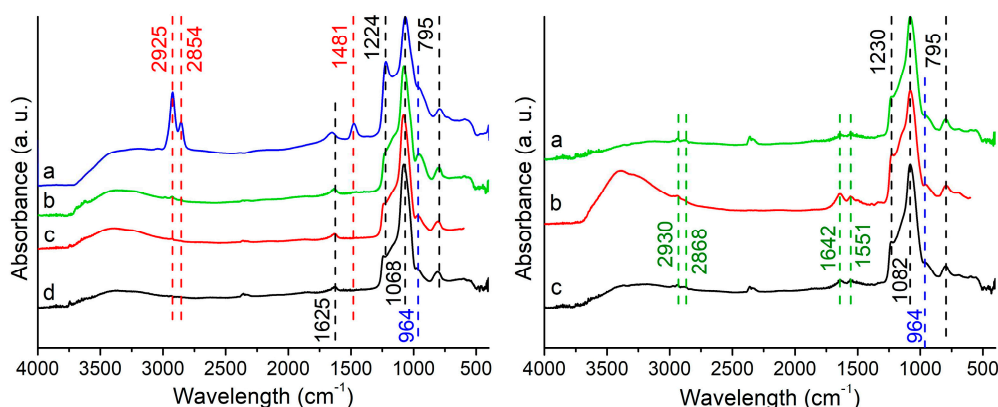
Figure 4. FTIR spectra of S-C samples: (Left) a) as-made, b) S-C-W, c) S-C-ST, and d) S-C-LT; (Right) a) S-C-W-g, b) S-C-ST-g, and c) S-C-LT-g. Bands attributed to surfactant (red lines), silanol groups (blue line), aminopropyl groups (green lines), and Si-O modes (black lines) are indicated.
