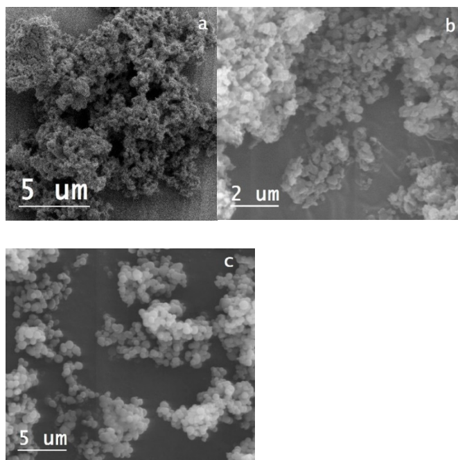
Figure 2. SEM images of samples S-C (a), S-B (b), and T-B (c).
