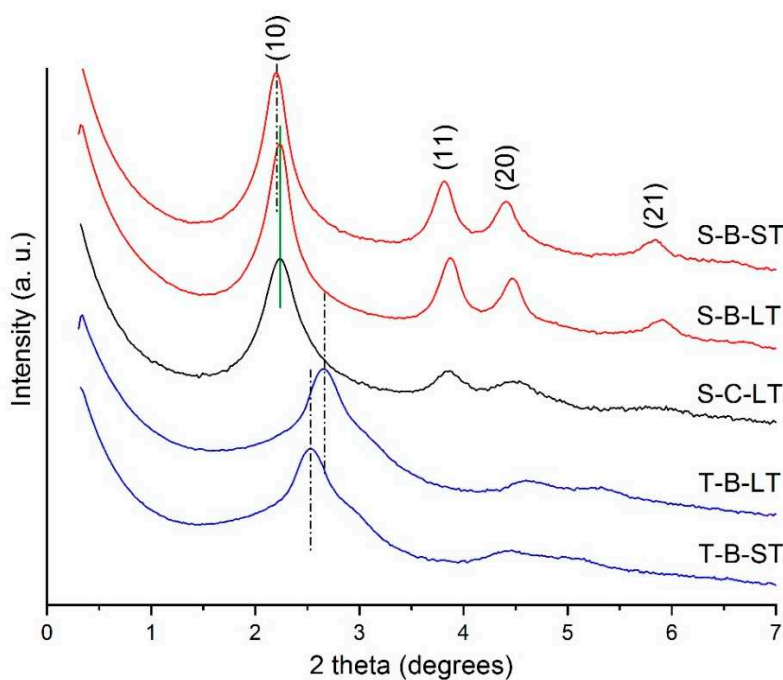
Figure 1. SAXS of MCM-41 samples.
