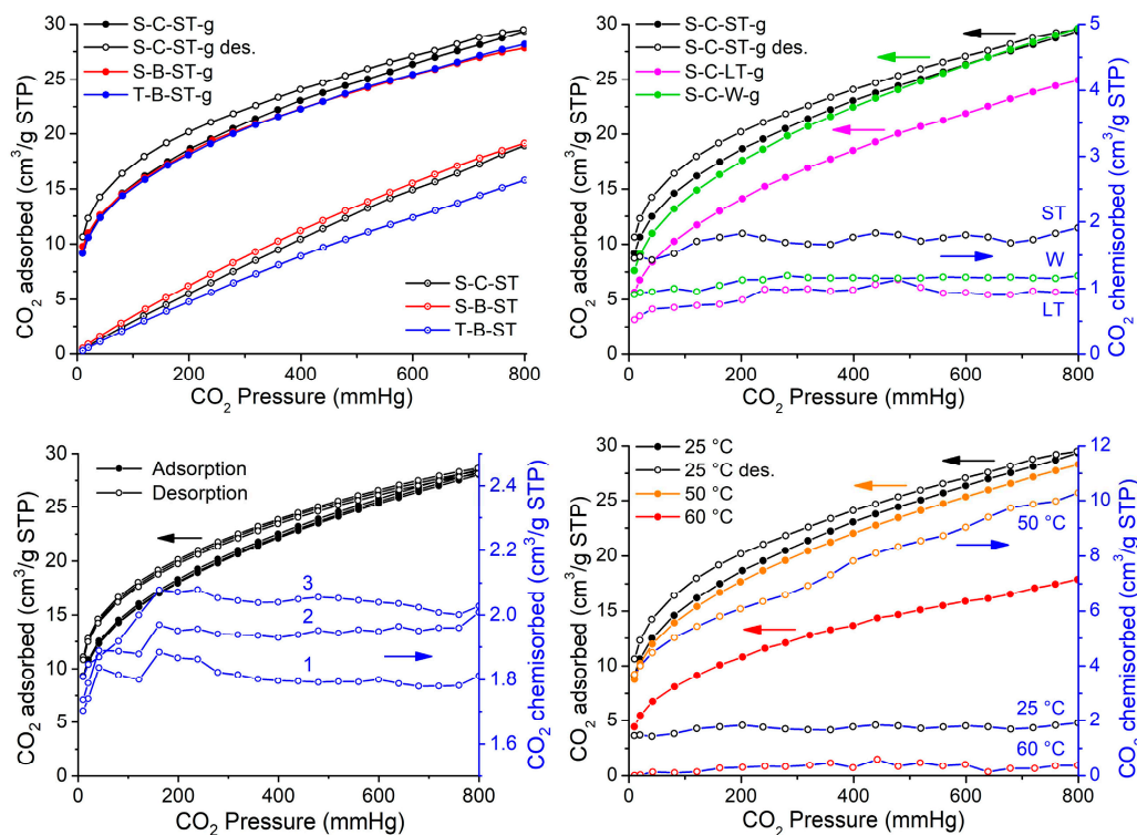
Figure 6. CO 2 total sorption isotherms at 25 °C of as-made and amine-modified MCM-41 (upper panels). Sorption isotherms of three consecutive cycles and adsorption/desorption isotherms at different temperatures for S-C-ST-g sample (lower panels).
