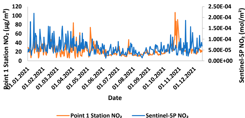
Figure 7. Comparative dynamics of NO 2 daily values for the year 2021 in Fujairah urban area, Point 1 ground-based station measurements are mentioned as orange line in \mu\text{g}/\text{m}^3 , Satellite data (Sentinel-5P) mentioned as blue line in \text{mol}/\text{m}^2 against the dates on horizontal axis.
