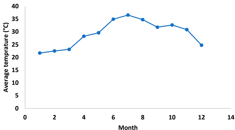
Figure 8. Average temperature in Celsius for each month of 2021 retrieved from Skamkam station data, Average temperatures in Celsius ( ^{\circ}\text{C} ) are shown in vertical axis and the months of 2021 on horizontal axis.
