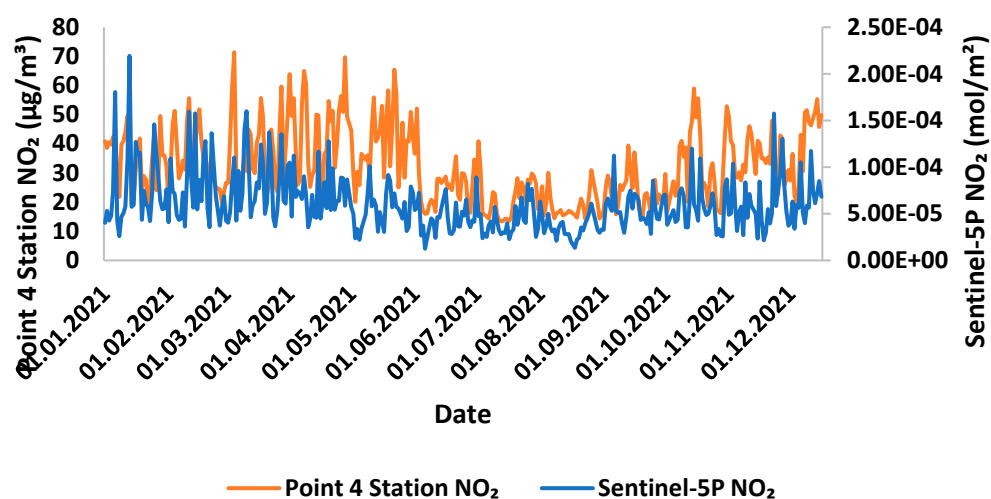
Figure 5. Comparative dynamics of NO 2 daily values for the year 2021 in Fujairah urban area, Point 4 ground-based station measurements are mentioned as orange line in µg/m 3 , Satellite data (Sentinel-5P) mentioned as blue line in mol/m against the dates on horizontal axis.
