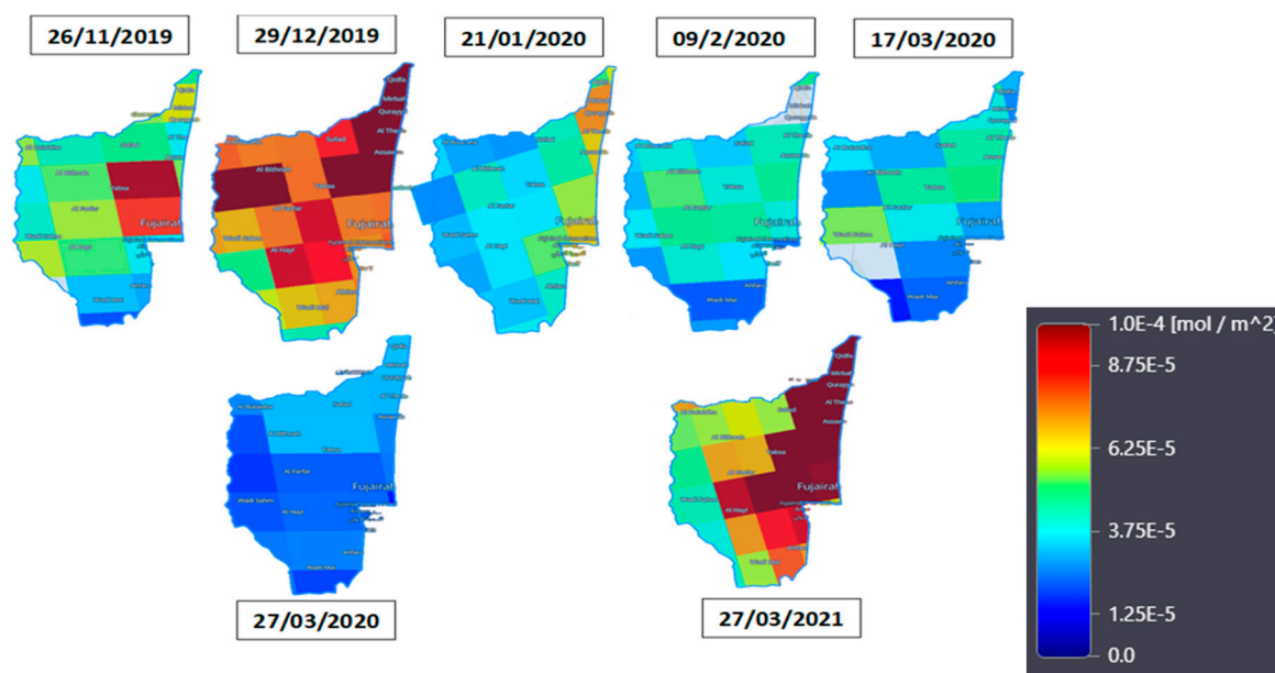
Figure 9. spatial distribution of NO 2 concentrations from Sentinel-5P. comparative maps on selected dates of average tropospheric NO 2 column number density over Fujairah urban area. On the right it shows the average tropospheric NO 2 column number density index.
