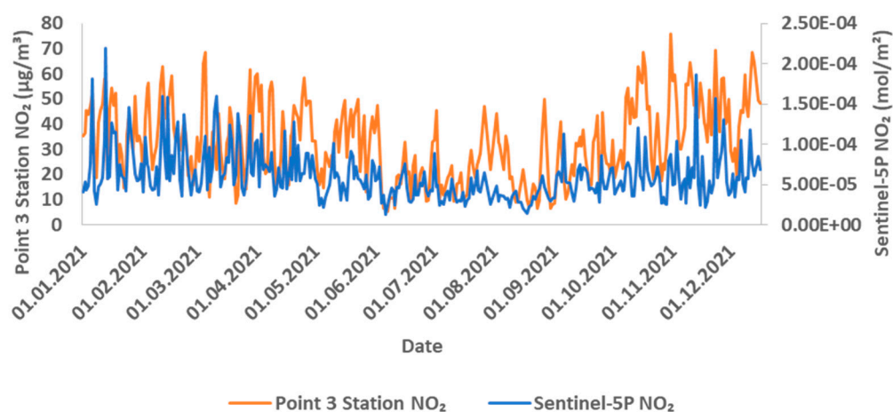
Figure 4. Comparative dynamics of NO 2 daily values for the year 2021 in Fujairah urban area, Point 3 ground-based station measurements are mentioned as orange line in µg/m 3 , Satellite data (Sentinel-5P) mentioned as blue line in mol/m against the dates on horizontal axis.
