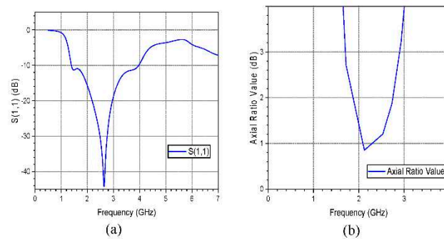
Figure 11. (a) S-parameter ( S_{11} ) plot (b) Axial Ratio plot.
