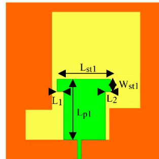
Figure 4. Slot Antenna with with one stub.
