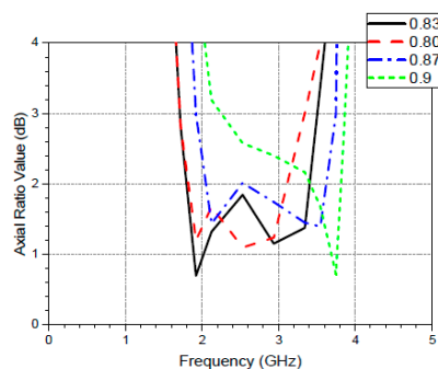
Figure 18. Axial Ratio plot for parametric analysis on the Crescent stub.
