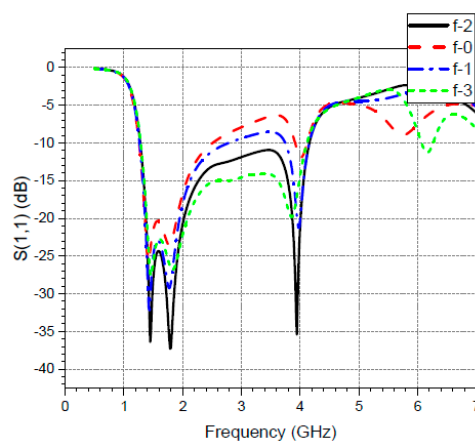
Figure 15. S-parameter (S11) plot for parametric analysis on offset feedline.
