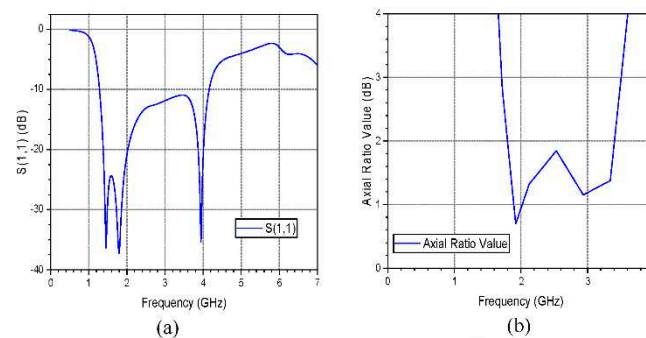
Figure 12. (a) S-parameter ( S_{11} ) plot (b) Axial Ratio plot.
