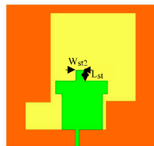
Figure 5. Slot Antenna with with two stub.
