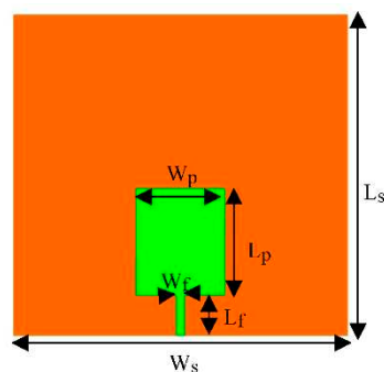
Figure 1. Antenna without slot.
