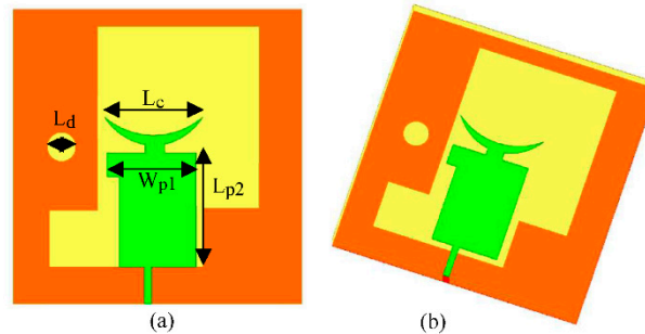
Figure 6. Slot Antenna with compositely-shaped patch (a) Top view (b) Trimetric view.
