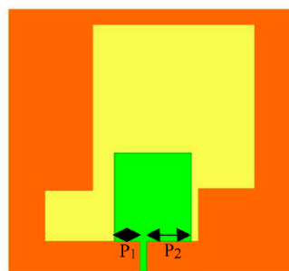
Figure 3. Slot Antenna with offset feeding.
