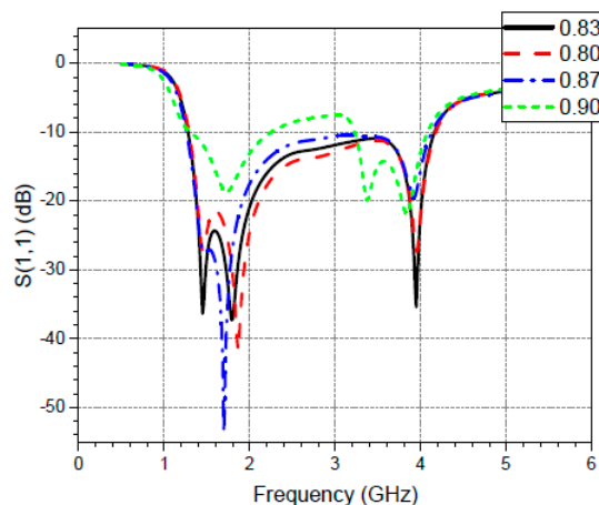
Figure 17. S-parameter (S11) plot for parametric analysis on the Crescent stub.
