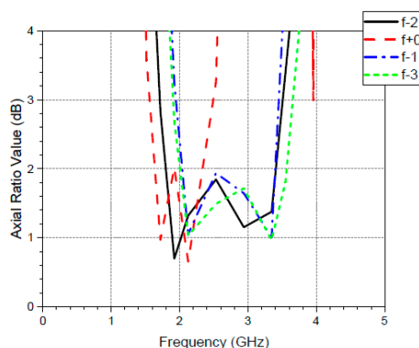
Figure 16. Axial Ratio plot for parametric analysis on offset feedline.
