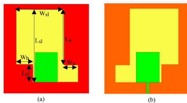
Figure 2. Slot antenna (a) Bottom view (b) Top view.
