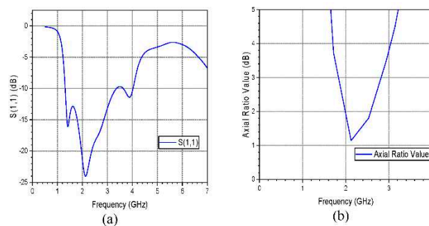
Figure 10. (a) S-parameter ( S_{11} ) plot, (b) Axial Ratio plot.
