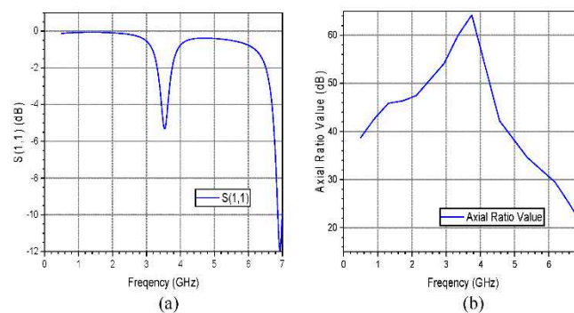
Figure 7. (a) S-parameter ( S_{11} ) plot (b) Axial Ratio plot.
