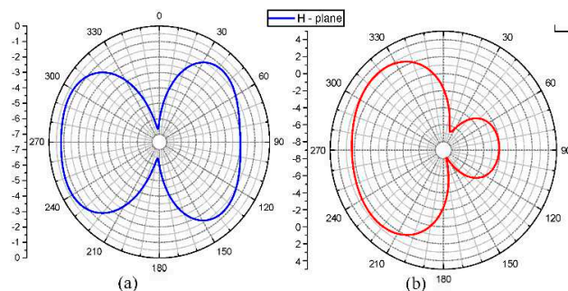
Figure 14. (a) Radiation pattern in H-plane (b) Radiation pattern in E-plan.
