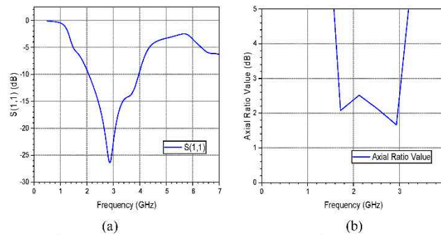
Figure 9. (a) S-parameter ( S_{11} ) plot (b) Axial Ratio plot.
