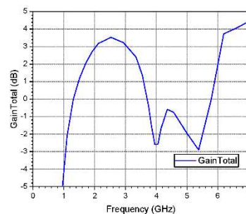
Figure 13. Simulated Gain results in dB plot.
