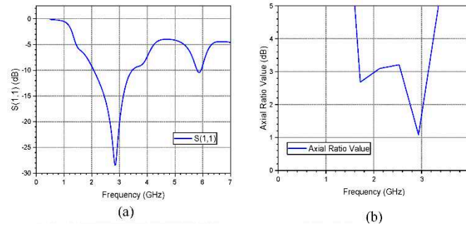
Figure 8. (a) S-parameter ( S_{11} ) plot (b) Axial Ratio plot.
