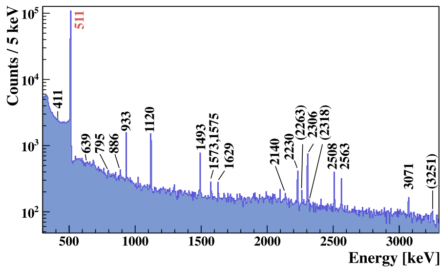
Figure 3. \gamma -ray energy spectrum for decay events correlated with ^{70}\text{Kr} implants.
