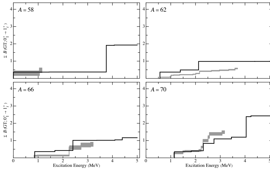
Figure 6. Distributions of the GT strength in the decay from N = Z - 2 to N = Z nuclei for A = 58 , 62, 66 and 70. The experimental B(\text{GT}) distributions and their uncertainties are indicated in grey. Parameters of the Hamiltonian (31) are given in Table 3 and the GT strength is calculated with a quenching factor q^2 = 0.74^2 .
