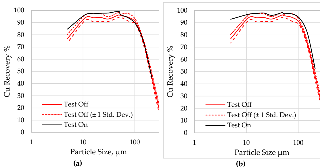
Figure A1. Size-by-size Cu recoveries in the rougher bank A, comparing the air-restricted case with the non-restricted scenario: (a) a low average air-restriction (a decrease in 1.2% in the average gas holdup with respect to the non-restricted case), (b) a moderate average air-restriction (a decrease in 1.9% in the average gas holdup with respect to the non-restricted case).
