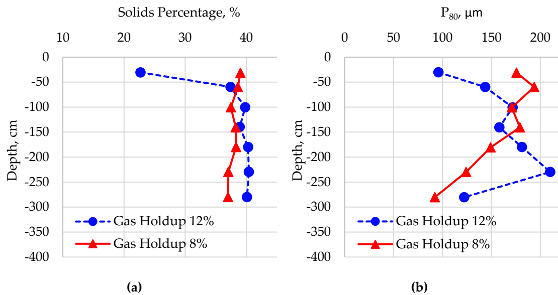
Figure 4. Axial profiles in the second cell of bank A: (a) solid percentage, (b) particle size.
