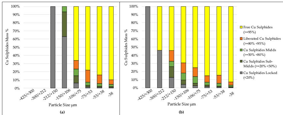
Figure 7. Liberation analysis for concentrate samples in the second cell of bank A: (a) non-restricted condition; (b) air-restricted condition.
