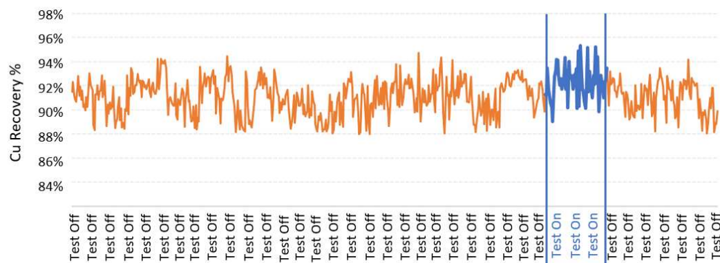
Figure 9. Cu recovery before and after restricting the air-intake, as described in Figure 8.
