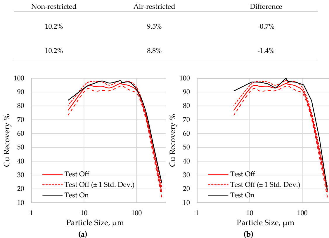
Figure 10. Size-by-size Cu recoveries in the rougher banks C and D, comparing the air-restricted case with the non-restricted case: (a) a low average air-restriction (a decrease in 0.7% in the average gas holdup with respect to the non-restricted case), (b) a moderate average air-restriction (a decrease in 1.4% in the average gas holdup with respect to the non-restricted case).
