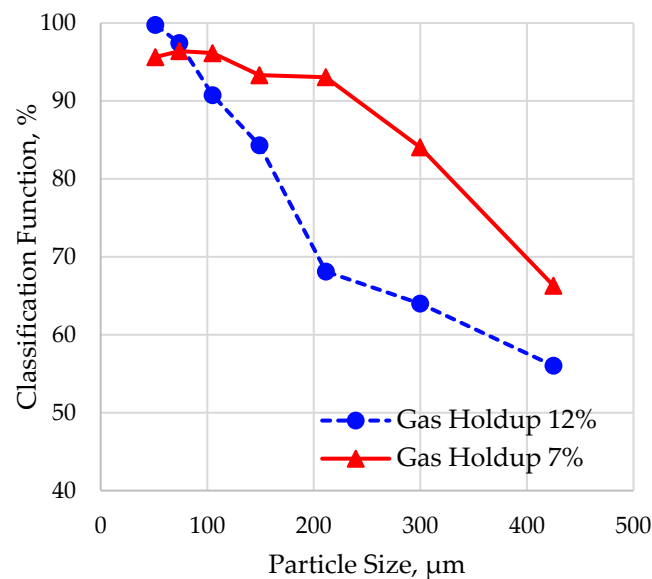
Figure 5. Classification function for the nominal ( \epsilon_G = 12\% ) and air-restricted ( \epsilon_G = 7\% ) conditions.
