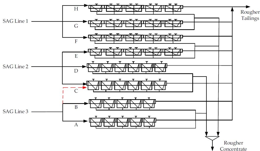
Figure 1. Rougher flotation circuit at Minera Los Pelambres [22].
