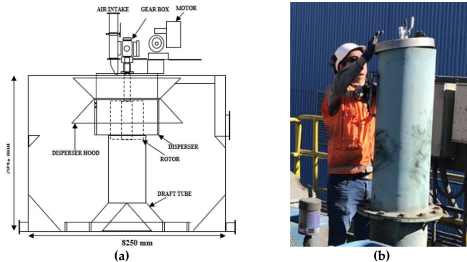
Figure 2. (a) WEMCO cell schematic; (b) a restriction of the air intake by installing a metallic cap with a ball valve.
