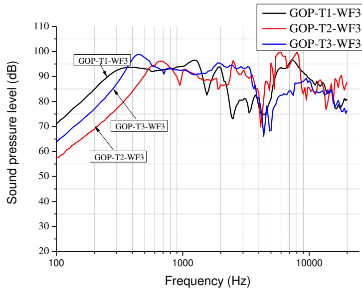
Figure 6. SPL curves for GO paper diaphragm headphones fabricated by various sonication times on suspension.
