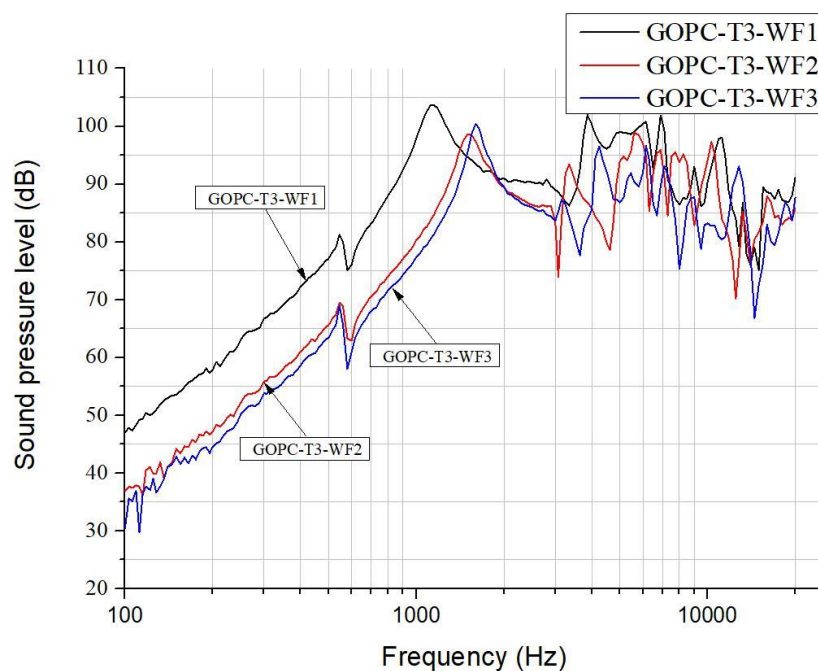
Figure 10. SPL curves for GOP/epoxy diaphragm headphones fabricated by various GO weight fractions in suspension.
