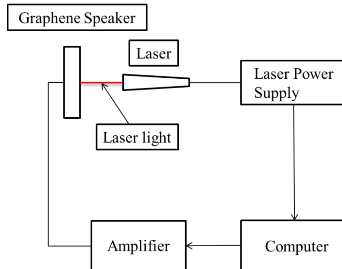
Figure 2. Set-up of the Klippel LPM laser measurement system for compliance of the GOP diaphragm.
