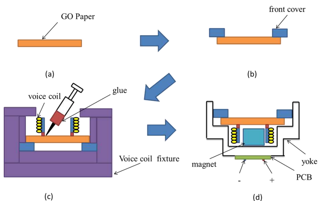
Figure 1. The fabrication procedure for a GOP headphone (a) preparation of GOP, (b) adhesion of GOP on a plastic ring, (c) alignment and adhesion of GOP/voice coil, (d) assemblage of the GOP diaphragm with a headphone unit.
