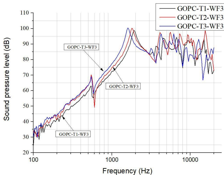
Figure 7. SPL curves for GOP/epoxy diaphragm headphones fabricated by various sonication times on suspension.
