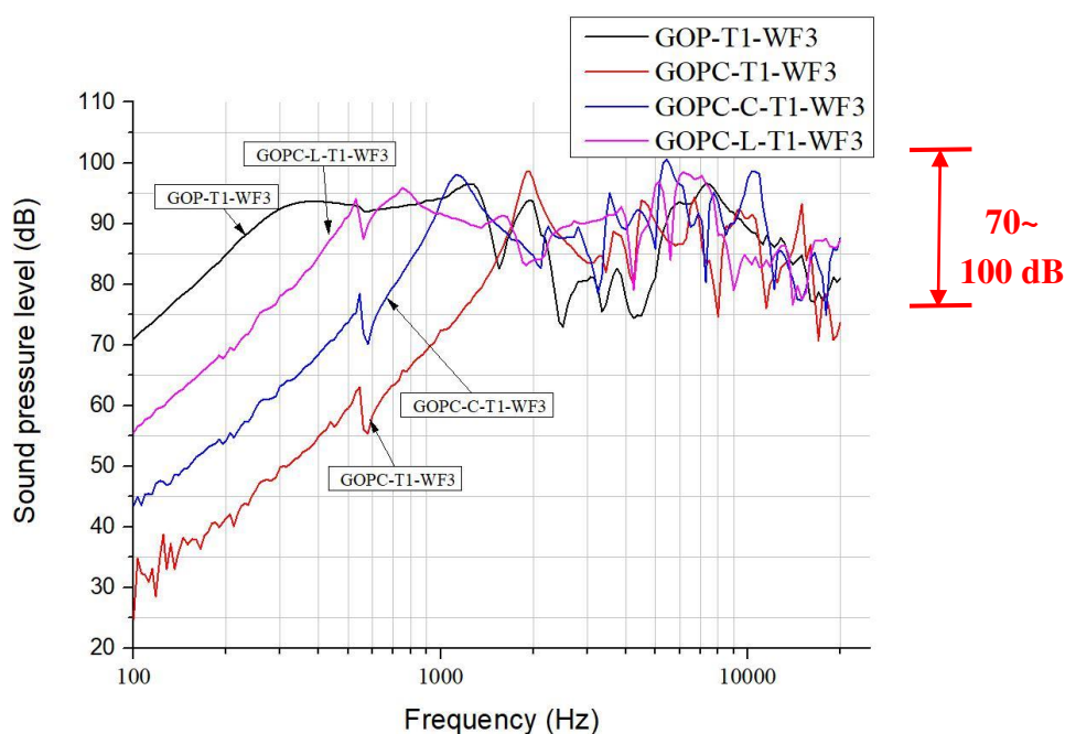
Figure 8. SPL curves for diaphragm headphones fabricated at lowest sonication time of T1 and WF3 by GO papers (GOP), GOP/epoxy nanocomposite without a pattern (GOPC), and with lined (GOPC-L) and curved patterns (GOPC-C).
