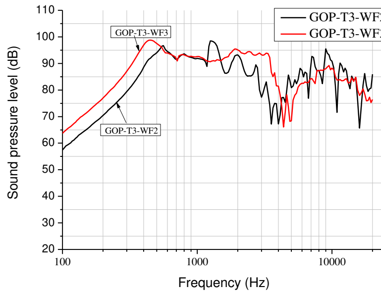
Figure 9. SPL curves for GO paper diaphragm headphones fabricated by various GO weight fractions in suspension.
