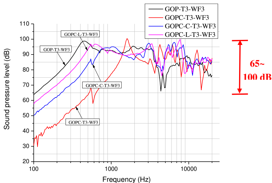
Figure 3. SPL curves for diaphragm headphones fabricated at highest sonication time of T3 and WF3 by GO papers (GOP), GOP/epoxy nanocomposite without a pattern (GOPC), and with lined (GOPC-L) and curved patterns (GOPC-C).
