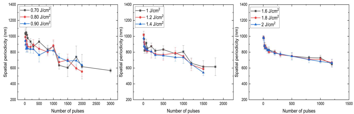
Figure 3. LIPSS spatial period as a function of the laser fluence and number of pulses. The target material is silicon irradiated by fs-laser pulses at 1030 nm in wavelength.
