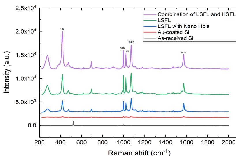
Figure 7. The SERS spectra of thiophenol molecules in ethanol adsorbed on the as-received Si surface, Au-coated as-received Si surface, Au-coated combination of LSFL and HSFL surface, Au-coated LSFL surface and Au-coated LSFL with Nano Hole surface.
