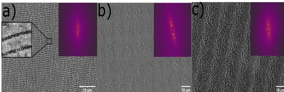
Figure 5. Scanning Electron Microscopy (SEM) Image of Homogeneous Large-Scale LIPSS Structure: (a) Combination of LSFL and HSFL (b) LSFL only, and (c) LSFL with Nano Hole.
