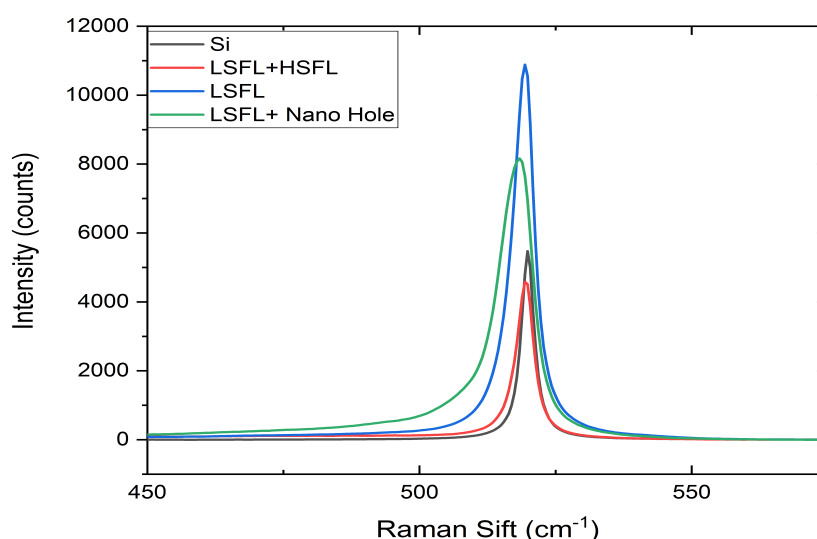
Figure 6. Raman spectra analysis of Crystalline Silicon and different LIPSS Structure.
