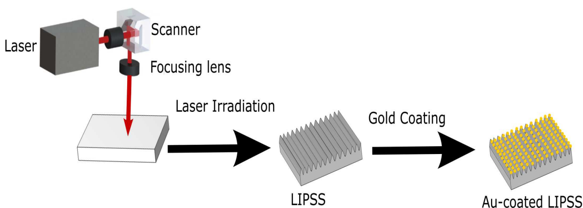
Figure 1. Schematic of the experimental process followed the fabrication of the gold nanoparticles on a silicon substrate.
