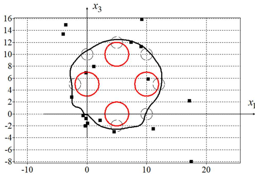
Figure 4. Optimal trajectory for adaptive synthesized control
