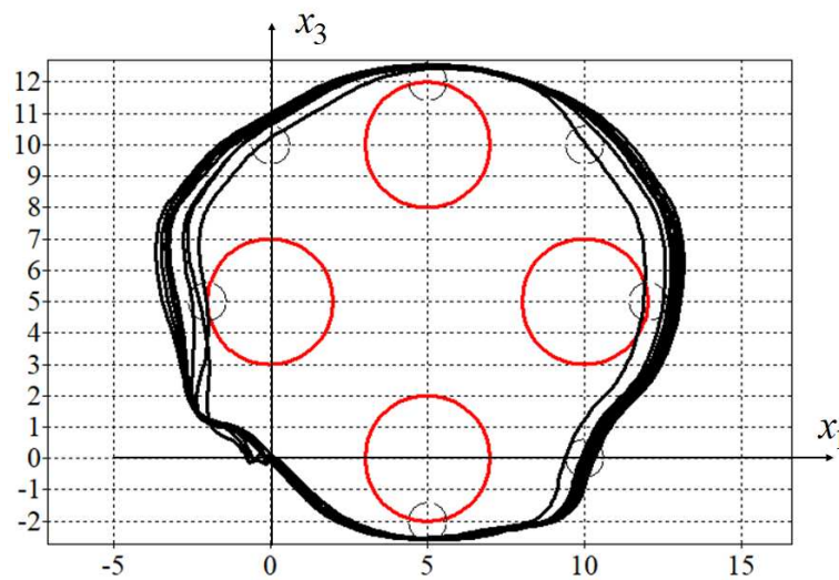
Figure 6. Optimal and eight disturbance trajectories of adaptive synthesized control
