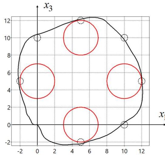
Figure 7. Optimal trajectory of direct control
