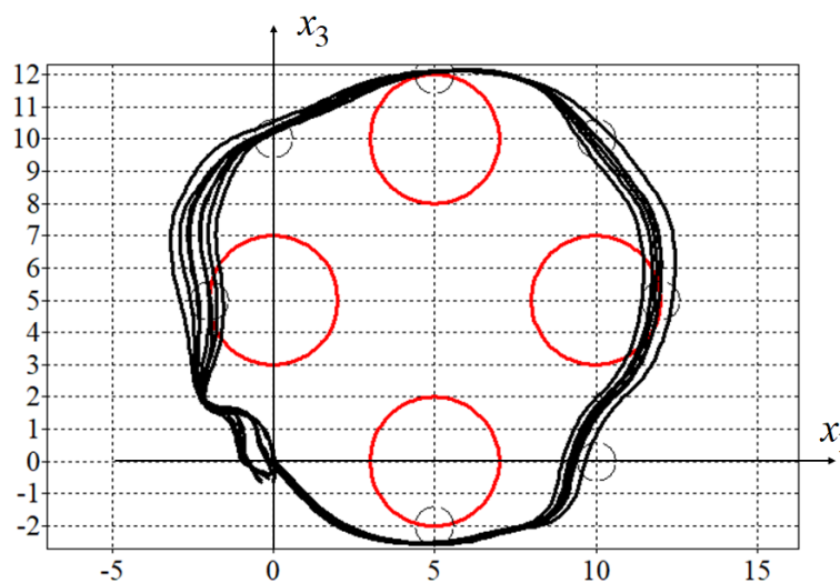
Figure 5. Optimal and eight disturbance trajectories of synthesized control
