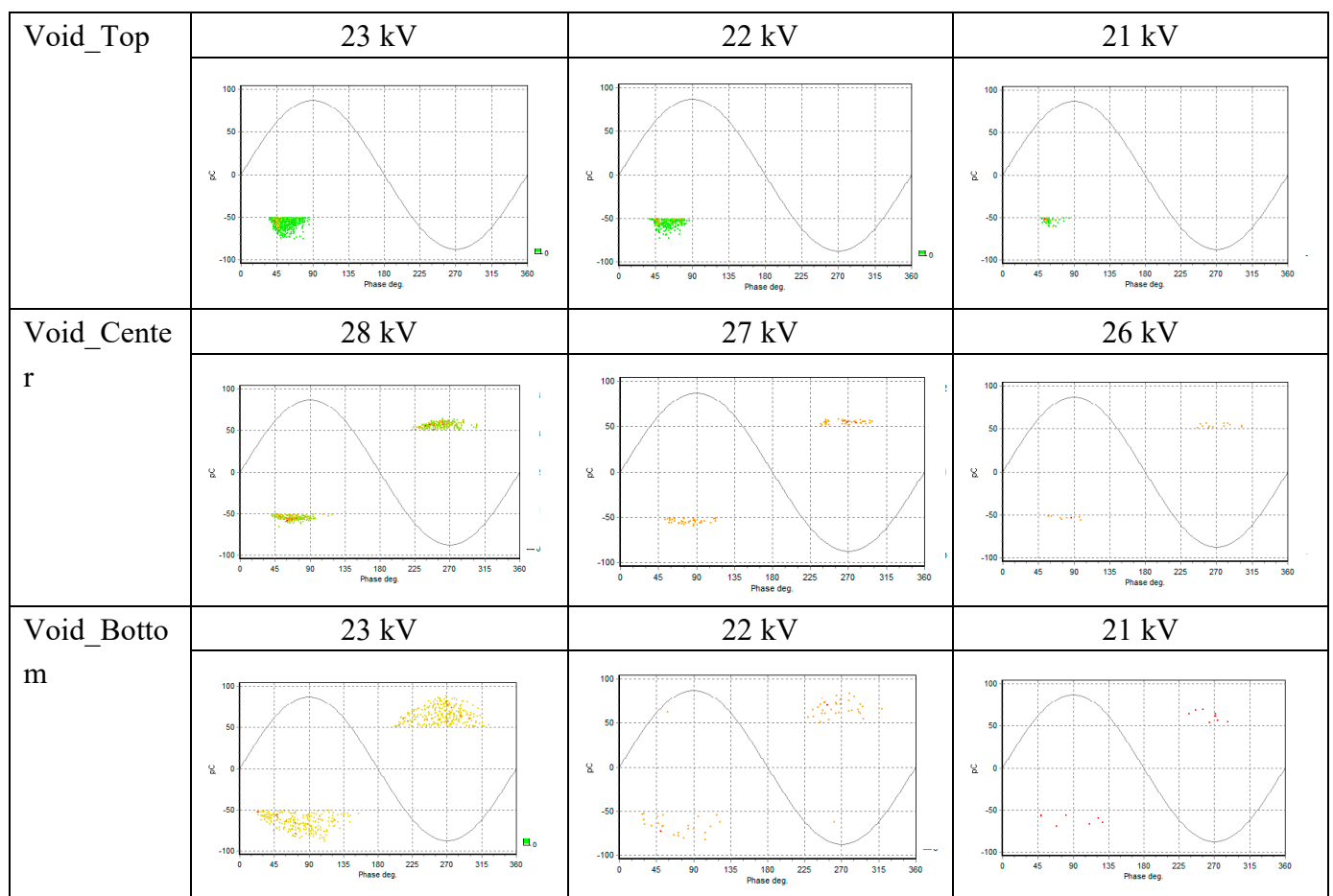
Figure 8. PRPD patterns for one-minute duration at different void positions.
