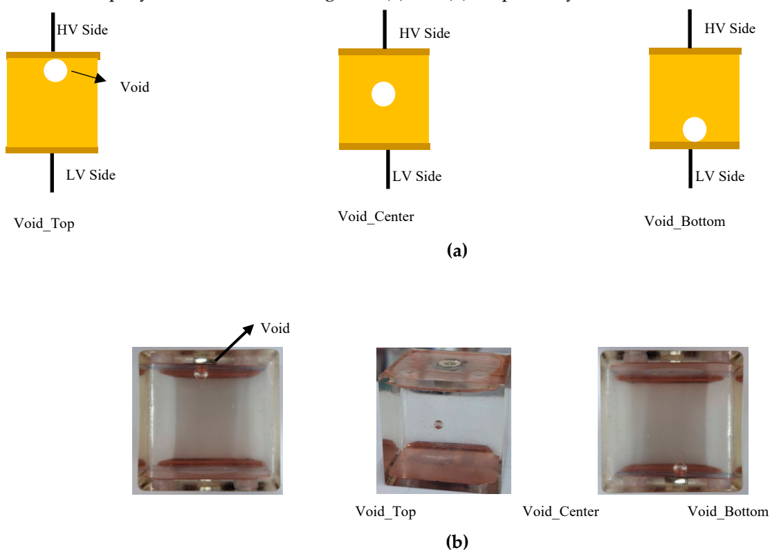
Figure 2. (a) Schematic diagram and; (b) experimental pictures of epoxy resins with voids at different positions.
