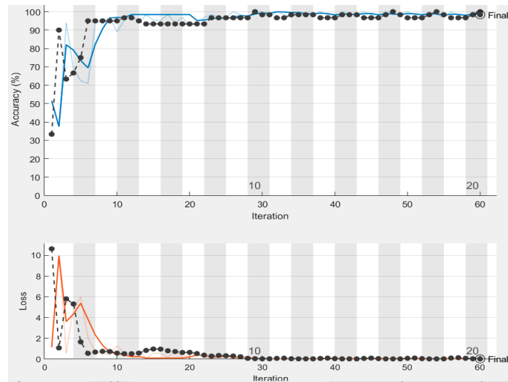
Figure 6. Learning curve of a CNN trained with PD data recorded at the PDIV.
