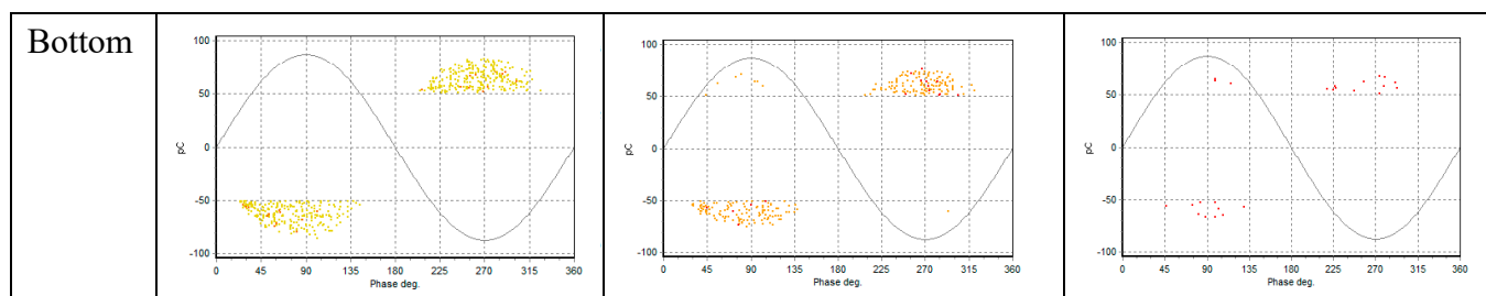
Figure 10. PRPD patterns for one-hour duration at different void positions.
