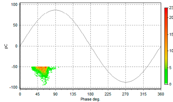
Figure 3. PRPD pattern with Void_Top in epoxy resin.
