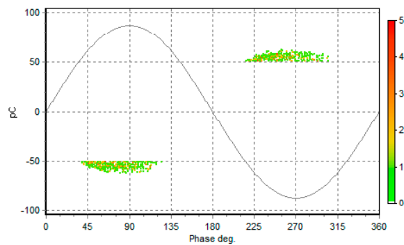
Figure 4. PRPD pattern with Void_Center in epoxy resin.
