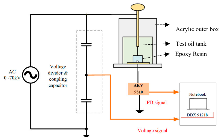
Figure 1. PD experimental setup of an epoxy resin with a void bottom.
