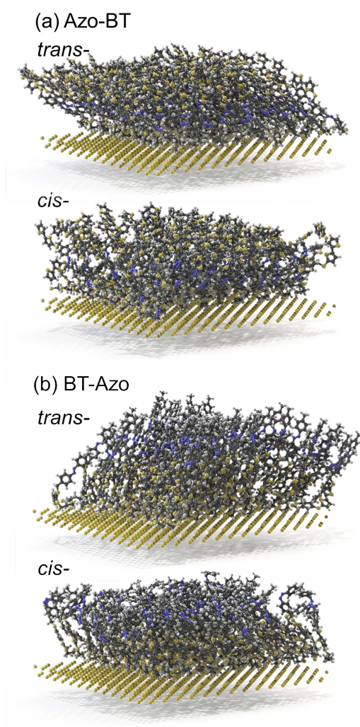
Figure 3. Chemisorbed monolayers of trans- and cis-Azo-BT (a) and trans- and cis-BT-Azo (b) as received in MD simulations. The gyration radius of the anchored molecules is 3.37 \pm 0.20 \text{ \AA} (trans-Azo-BT), 2.38 \pm 0.43 \text{ \AA} (cis-Azo-BT), 3.72 \pm 0.33 \text{ \AA} (trans-BT-Azo), and 2.84 \pm 0.40 \text{ \AA} (cis-BT-Azo).
