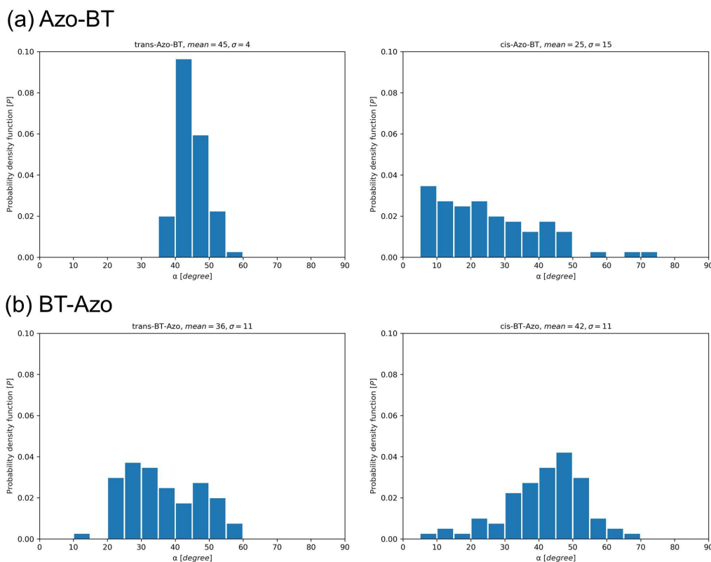
Figure 5. Probability density function P showing populations of angles between a normal to the gold surface and a vector connecting thiol sulfur and a middle of the thiophene-thiophene bond in Azo-BT (a) or a middle of the N=N bond in BT-Azo (b).
