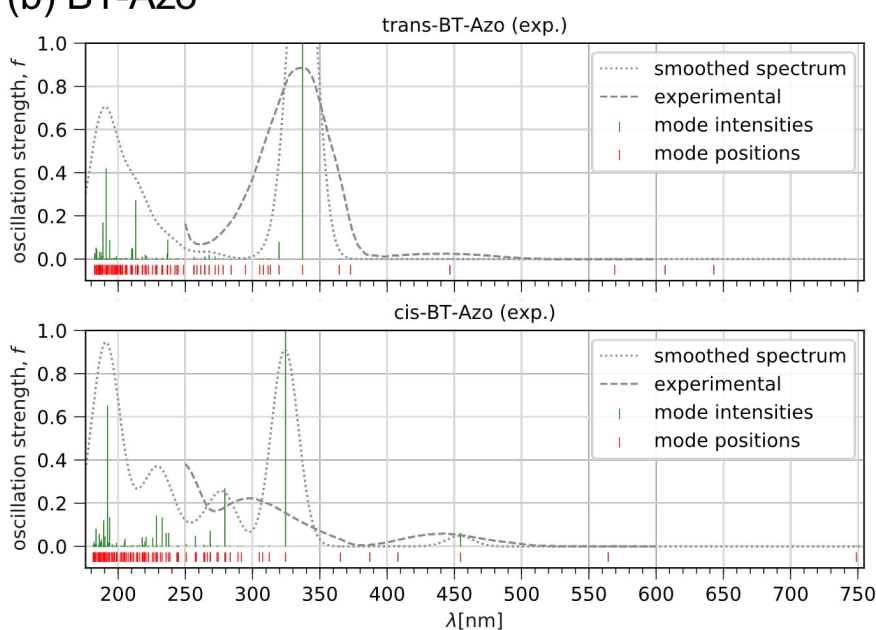
Figure 2. Absorption spectra (dotted lines) of trans-, cis-Azo-BT (a) and trans-, cis-BT-Azo (b) as received in TD-DFT calculations. The dashed lines on panel (b) are the experimental spectra from Ref. [10] with \lambda_{max} = 341 nm ( \pi - \pi^* ) and 435 nm ( n - \pi^* ).
