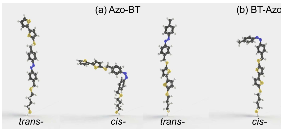
Figure 1. The optimized geometries of Azo-BT (a) and BT-Azo (b) in trans- and cis-state with a common formula C_{26}H_{26}N_2S_5 . The abbreviations Azo and BT stand for azobenzene and bithiophene, respectively. The molecules (a) and (b) differ in the sequence of Azo and BT blocks counting from the spacer with thiol group, i.e. they are structural isomers. For example, this group anchors BT-Azo (b) molecules to the surface of an electrode [10,11,47] or a nanoparticle [23,45,46]. We use Azo-BT and BT-Azo nomenclature for the sake of convenience only. The carbon, nitrogen, sulfur, and hydrogen atoms are colored in gray, blue, yellow, and white. This color scheme is used throughout the paper. The static dipole moments are 1.67 and 3.52D for (a) trans- and cis-isomers, and 1.34 and 3.22 D for (b) trans- and cis-states, respectively, as obtained in our recent publication [30].
