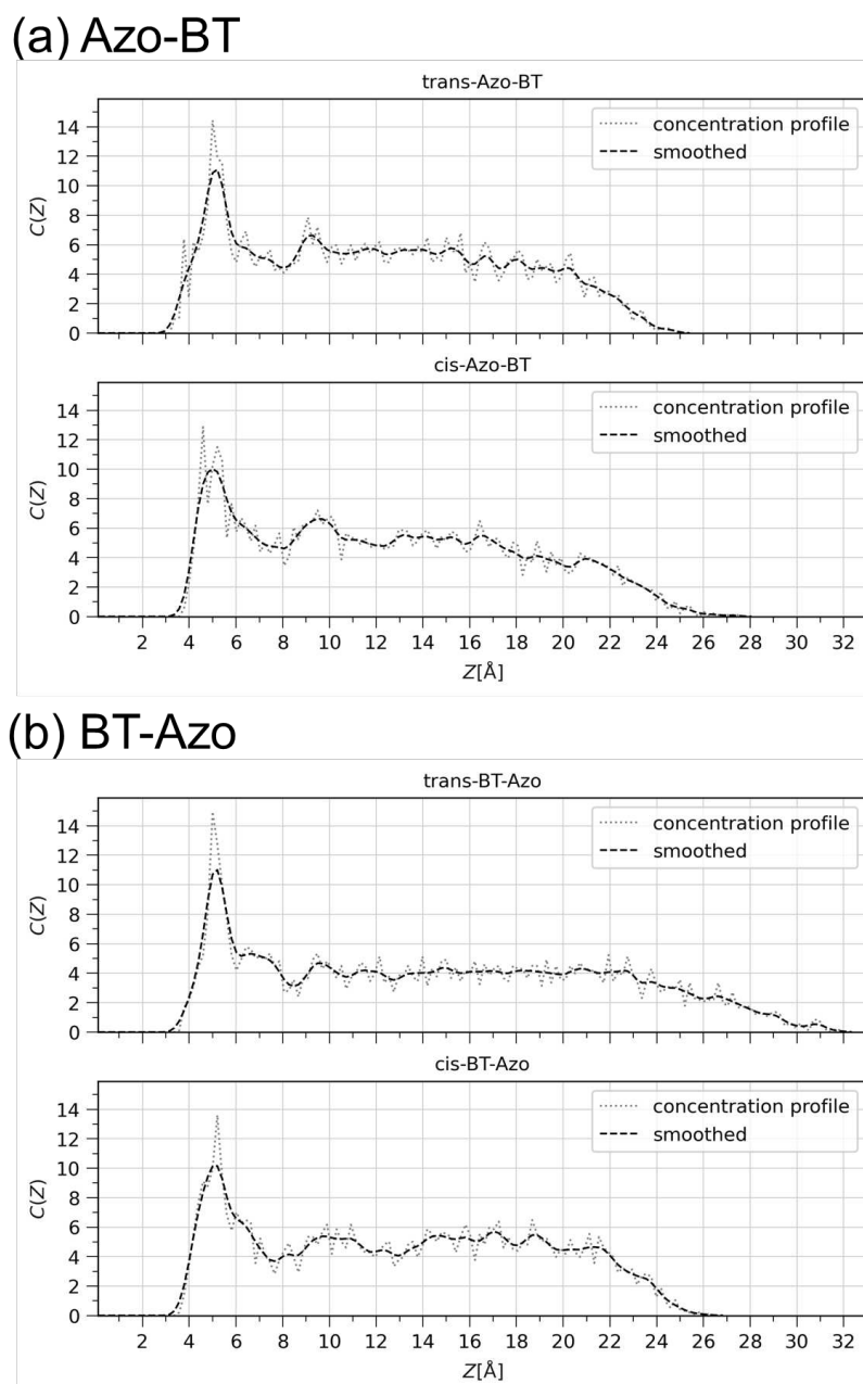
Figure 4. Concentration profiles of trans- and cis-Azo-BT (a) and trans- and cis-BT-Azo (b). The concentration profile C(Z) calculates the concentration of particles in a given layer away from the gold surface located at Z=0 . The reported values of C(Z) are relative to a random distribution and are therefore unit-less. The values range from 0 (no atoms in the layer), to a maximum value corresponding to the total number of bins if all atoms reside in the same layer. The sum over all layers or stripes is equal to the total number of bins.
