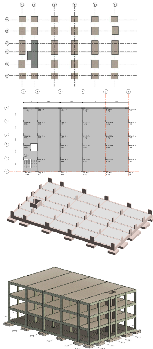
Figure 7. Sequence of the modelling process of the structural model made in Revit.
