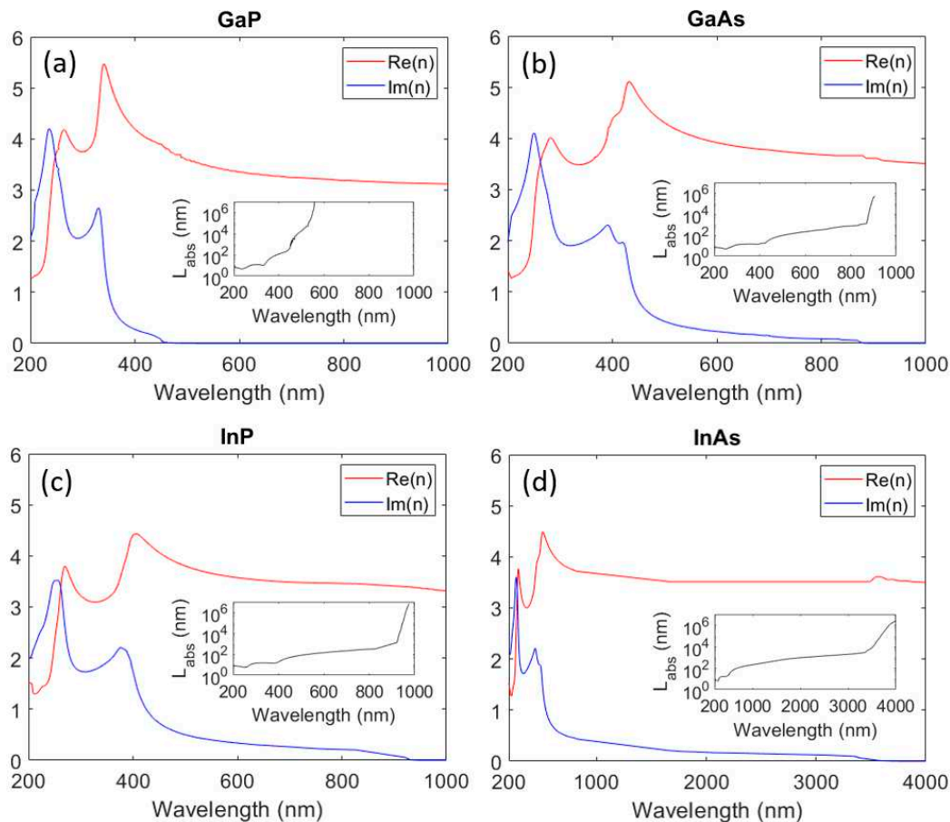
Figure 3. Refractive index of the III-V semiconductors GaP, GaAs, InP, and InAs, with tabulated data from Refs. [26–29], respectively. The insets show the corresponding absorption length L_{\text{abs}} on a logarithmic scale. We show here InAs with an extended wavelength range due to its lower bandgap, see Table 1.
