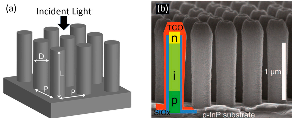
Figure 1. (a) Schematic of a nanowire array with nanowires of diameter D and length L in a square array of period P . (b) Scanning electron microscopy image of an InP nanowire array solar cell with n, i, and p indicating the regions of the InP diode; and TCO indicates the transparent conductive oxide used for the top side electrical contacting. Reproduced with permission from Wallentin et al. Science 339, 1057 (2013). Copyright 2013 the American Association for the Advancement of Science.
