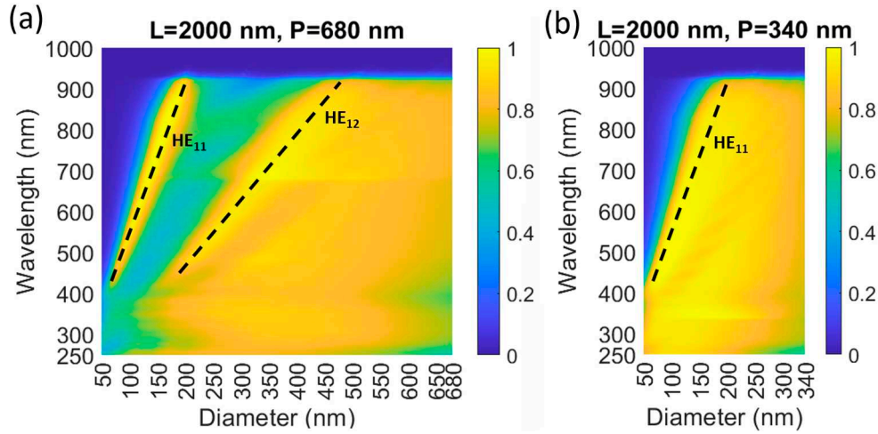
Figure 4. Modelled absorptance of normally incident light in InP nanowires on InP substrate, that is, the same system as studied in Ref. [2], recalculated for this Review in the same way as in Ref. [2] to allow this replotting. (a) L = 2000 nm and P = 680 nm. For this L , P = 680 nm and D = 441 nm gives, a peak of j_{sc} = 27.6 mA/cm 2 , which occurs when the HE 12 absorption peak is placed to the vicinity of the bandgap wavelength. This P and D is the optimum choice if using this HE 12 for this L . (b) L = 2000 nm and P = 340 nm. For this L , P = 340 nm and D = 184 nm gives, for any value of D and P , the maximum absorption corresponding to j_{sc} = 29.0 mA/cm 2 . These values are calculated for the AM1.5D spectrum (see Figure 2) for which the maximum values for InP with E_g = 1.34 eV is 31.1 mA/cm 2 , which occurs when all above bandgap light is absorbed (see inset in Figure 2). The horizontal scaling in (a) and (b) is set equal to allow easier comparison. Here, to guide the eye, we indicate the absorption peak due to the HE 11 and HE 12 waveguide modes (dashed lines). The region of low absorptance for small D/\lambda to the left of the dashed line indicating the HE 11 peak originates from the electrostatic screening [24]. For InP, \lambda_g = 925 nm, and for \lambda > \lambda_g , the absorption drops rapidly to negligible values.
