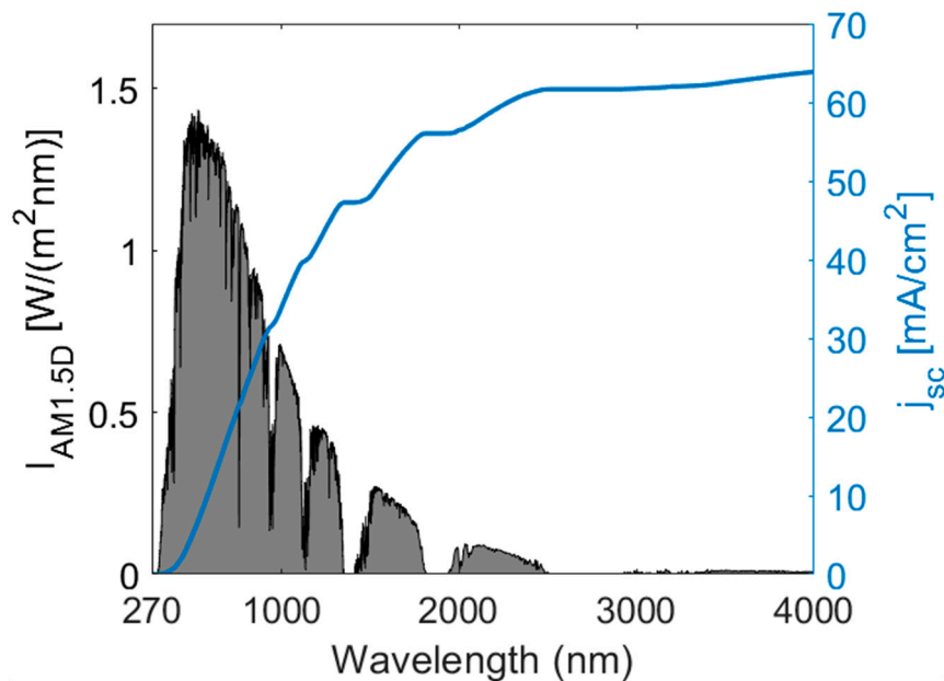
Figure 2. The direct and circumsolar 900 W/m 2 I_{AM1.5D} spectrum (grey patched area) is shown with values on the left axis [18]. Here, also the corresponding maximum short-circuit current j_{sc} as a function of bandgap wavelength (blue line) is shown with values on the right axis, under the assumption that all incident above bandgap photons are absorbed, that is, that A_{inc}(\lambda) = 1 for \lambda < \lambda_g .
