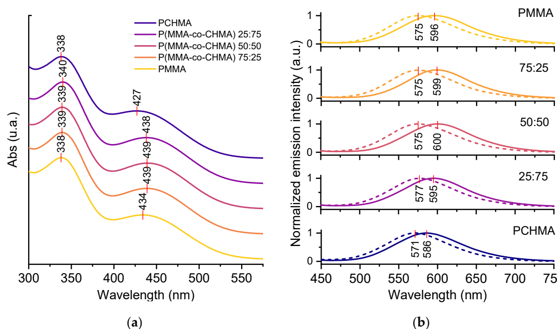
Figure 7. (a) Absorption spectra of TPE-BPAN in the five polymeric matrices under study at 2.0 wt.% concentration. Peak positions are marked with red vertical dashes. (b) Emission spectra of TPE-BPAN
