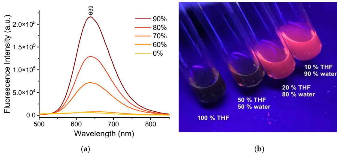
Figure 2. (a) Emission spectra of TPE-BPAN dissolved in THF/H 2 O mixtures at different compositions; (b) Picture showing solutions of TPE-BPAN in various THF/H 2 O mixtures under UV irradiation (366 nm).
