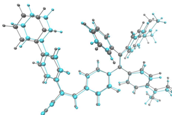
Figure 4. Superposition of the optimized ground state ( S_0 , gray) and first excited state ( S_1 , cyan) structures computed for TPE-BPAN .
