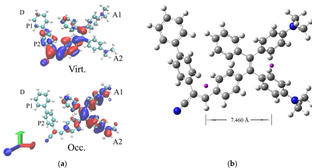
Figure 3. (a) NTO orbital associated to the S_0 - S_1 transition of TPE-BPAN . (isodensity = 0.025 a.u.). (b) Graphical representation of the D_{\text{CT}} : barycenters of hole and electron charge distribution are in violet.
