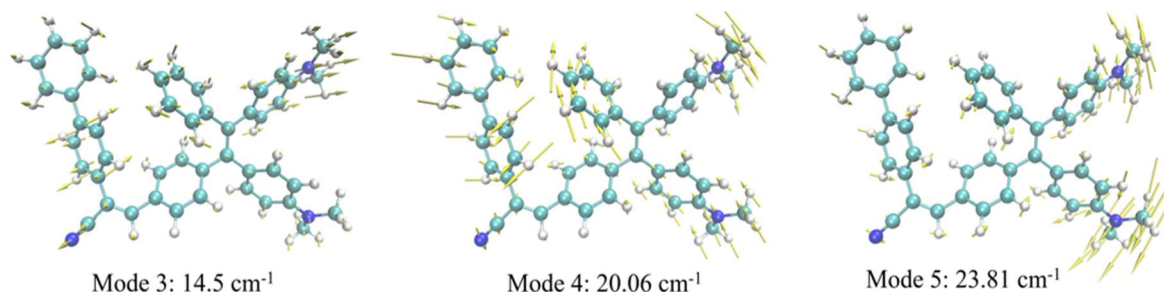
Figure 5. Schematic representation of the normal modes related to the largest HR factors of TPE-BPAN.
