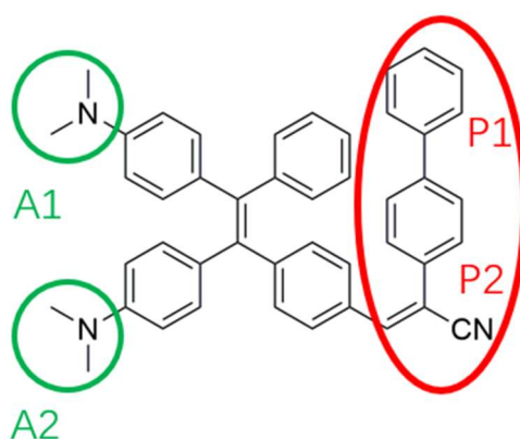
Figure 1. Schematic structure of TPE-BPAN highlighting the donor (green) and acceptor (red) substituent groups introduced in the TPE core.
