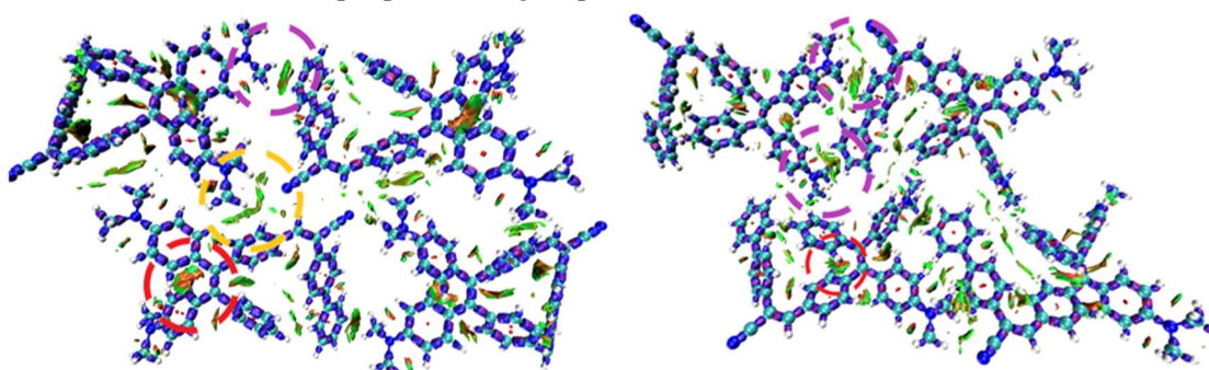
Figure 6. Interaction Region Indicator analysis computed for TPE_BPAN in the Pol_2 and Pol_3 phases. Refer to text for further explanation.
