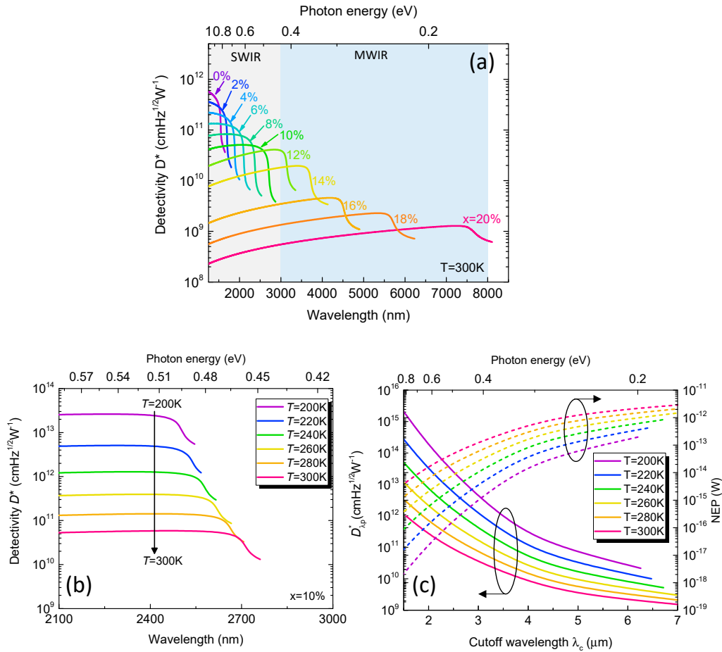
Figure 6. (a) Calculated specific detectivity spectra of GeSn PDs with various Sn contents at T=300 K. (b) Calculated specific detectivity spectra for \text{Ge}_{0.9}\text{Sn}_{0.1} PD in the temperature range of T=200\text{-}300 K. (c) Calculated peak detectivity and NEP as a function of cutoff wavelength in the temperature range of T=200\text{-}300 K.
