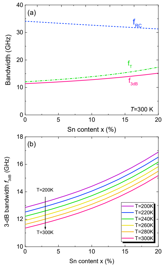
Figure 8. (a) Calculated transit-time-delay-limited bandwidth, RC-delay-limited bandwidth and 3-dB bandwidth of GeSn PDs as a function of Sn content at T=300\text{ K} . (b) Calculated 3-dB bandwidth as a function of Sn content at various temperatures.
