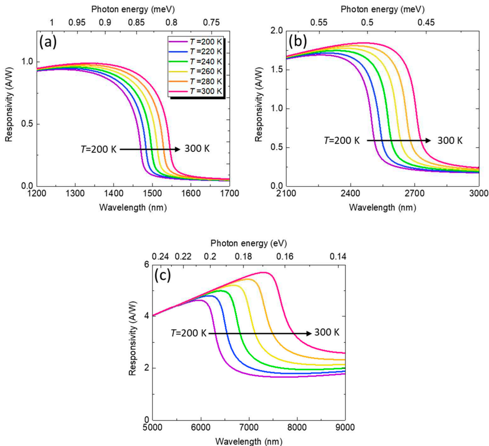
Figure 5. Calculated responsivity spectra of GeSn PDs with Sn contents of (a) x=0\% , (b) x=10\% , and (c) x=20\% in the temperature range of T=200-300 K.
