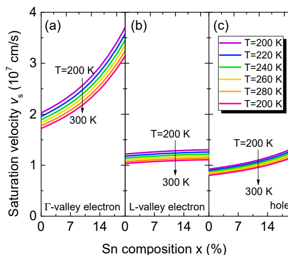
Figure 7. Calculated electron and hole saturation velocities as a function of Sn content in the temperature range of T=200 - 300 K.
