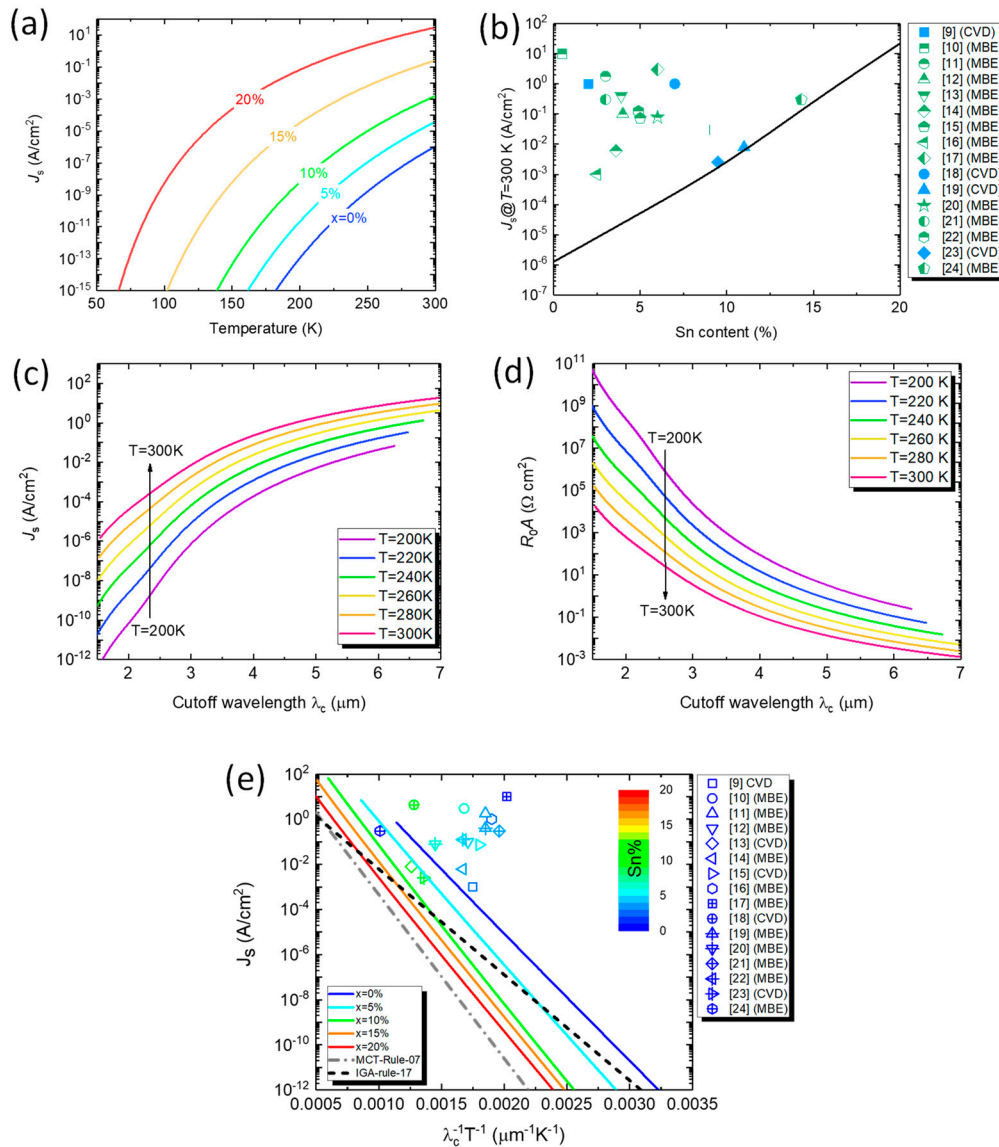
Figure 3. Calculated GeSn-rule-23 performance for GeSn PDs. (a) Calculated dark current density as a function of temperature. (b) Calculated dark current density at T=300 K for GeSn PDs as a function of Sn content. Experimental dark current densities taken from Refs. [9–24] are also shown for comparison. Calculated (c) dark current density, and (d) R_0A product of the GeSn PDs as a function of cutoff wavelength in the temperature range of T=200 – 300 K. (e) Calculated GeSn-rule-23 performance by means of dark current density as a function reciprocal of the product cutoff wavelength and temperature (solid lines) compared with reported experimental data (scatters) in the literature [9–24]. MCT rule-07 (dashed-dotted line) [26] and IGA-rule-17 (dashed line) [27] and are also depicted for comparison.
