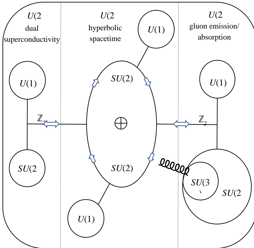
Figure 4. Decomposition of symmetry groups to establish common U(2) scale- and gauge-invariance. This model of invariance provides a mechanism through which the pressure-induced ‘rolling’ critical response results in PV work that is either positive or negative. The complex reorganization of water ice cages produces variable inertia which, through the conservation of angular momentum, is responsible for either an acceleration or deceleration of quarks. In the case of acceleration, this leads to the emission of physical gluons that are absorbed into the QCD vacuum manifold. A corresponding tendency to reduce local ‘space density’ and effective magnetic permeability \mu_0 manifests as increased hyperbolic curvature K .
