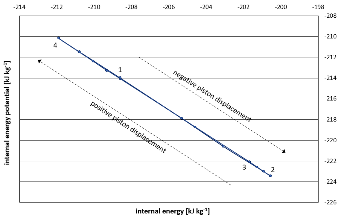
Figure 2: Excess internal energy potential resulting from excess thermodynamic potentials. All values for energy and thermodynamic potentials are derived from the pressure and temperature measurements by the NIST REFPROP program/database. The calculations are in accordance with GERG-2008 modified by the Kunz and Wagner Model 0 (KW0). The piston expander is completely immersed in a heat bath with a temperature of 270K, approx.
