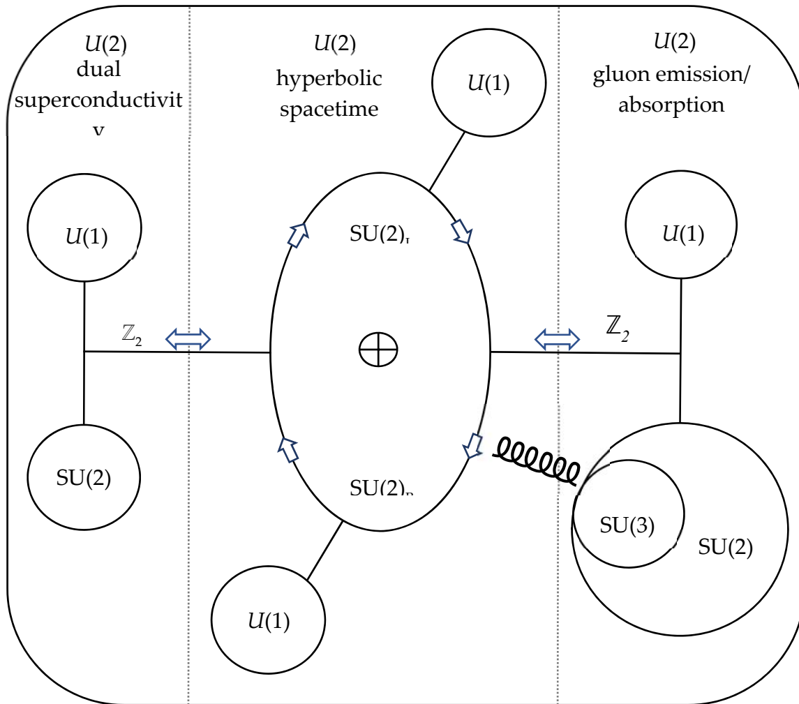
Figure 4: Decomposition of symmetry groups to establish a common U(2) gauge-invariance. This model of gauge-invariance provides a mechanism through which the pressure-induced ‘rolling’ critical response results in PV work that is either positive or negative. The complex reorganization of water ice cages produces variable inertia which, through the conservation of angular momentum, is responsible for either an acceleration or deceleration of quarks. In the case of acceleration, this leads to the emission of physical gluons that are absorbed into the embedding manifold. A corresponding tendency to reduce local ‘space density’ and effective magnetic permeability \mu_0 manifests as reduced hyperbolic curvature and negative PV work. Conservation of magnetic charge imposes a superconducting phase transition on the crystal-fluid material.
