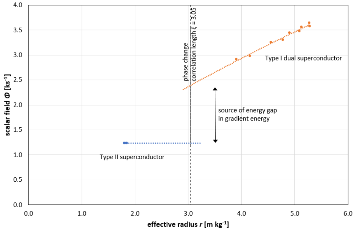
Figure 3: Effect of inertia and critical correlation length on the magnitude of the scalar field. A gradient energy term, as derived from the Lagrangian function, describes the dynamical system. This, in turn, reveals scalar field \Phi values associated with the critical response and a field coupling constant of 1. Energy conservation requires that non-extensive PV work be balanced through an equal-and-opposite electromagnetic coupling to the scalar field. The gradient energy term of the Lagrangian corresponds to the hyperbolic geometry and topology of the system, as well as its inertial potential. In considering the variable effective radius r of the system (ie. its 'hidden' inertia), the corresponding Euclidean volume \sim e^{3r} .
