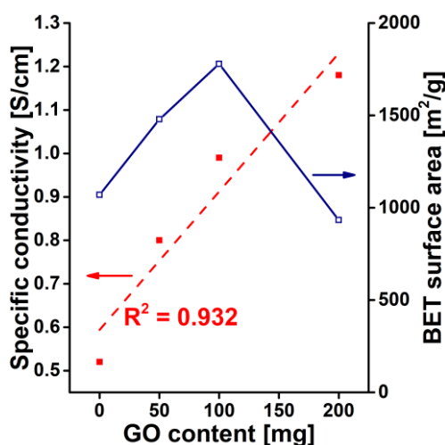
Figure S5 Influence of GO on the specific conductivity and apparent surface area
