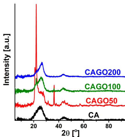
Figure S7 XRD diffractograms of CA and GO doped carbon samples. Normalized to peak at 2\theta \approx 25-26 position
