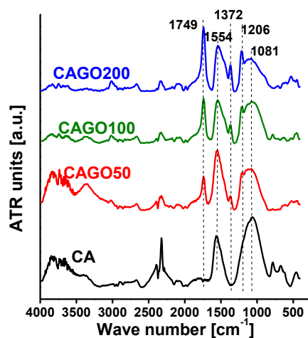
Figure S4 FTIR spectra of the carbon samples. See also Table S3
