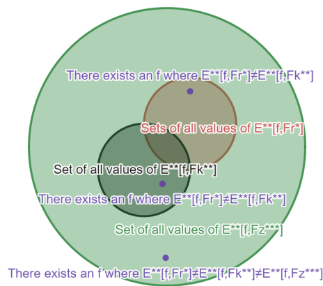
Figure 1. Below F_r^* , F_k^{**} , F_z^{***} are non-equivalent starred sequences of sets, where V' is all circles and E^{**} is the generalized expected value of f w.r.t either \star -sequence of sets (def. 8)
