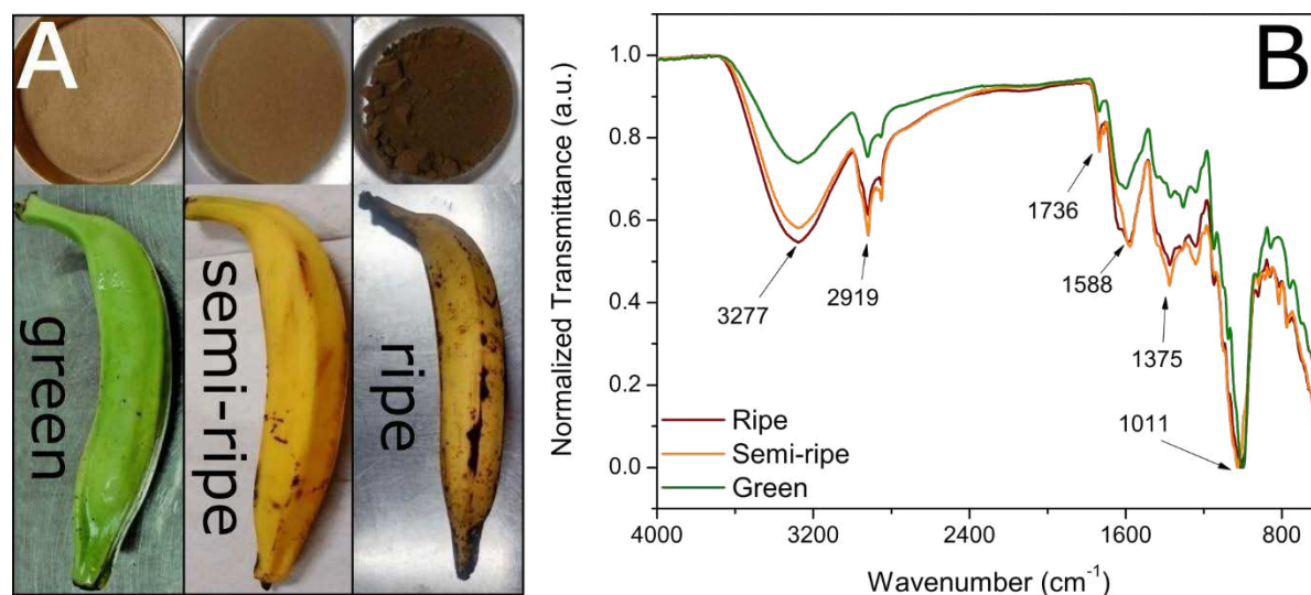
Figure 1. Optical images of the banana fruits and the obtained BPP at the different ripeness stages (A) and FTIR spectra of the BPP samples (B).
