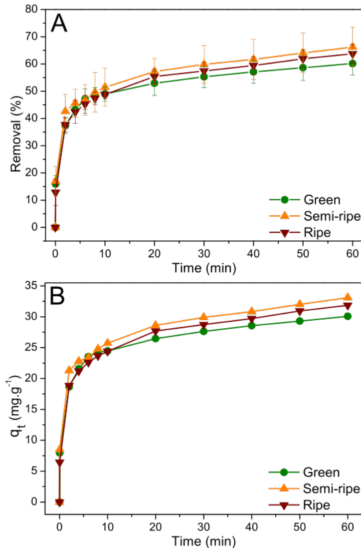
Figure 4. Removal (%) of methylene blue dye (a) and adsorption capacity of the BPP biosorbents obtained at different ripening stages (b). Conditions: 50 mg of BPP; 50 mL MB dye solution at C_0 = 50 mg L -1 .
