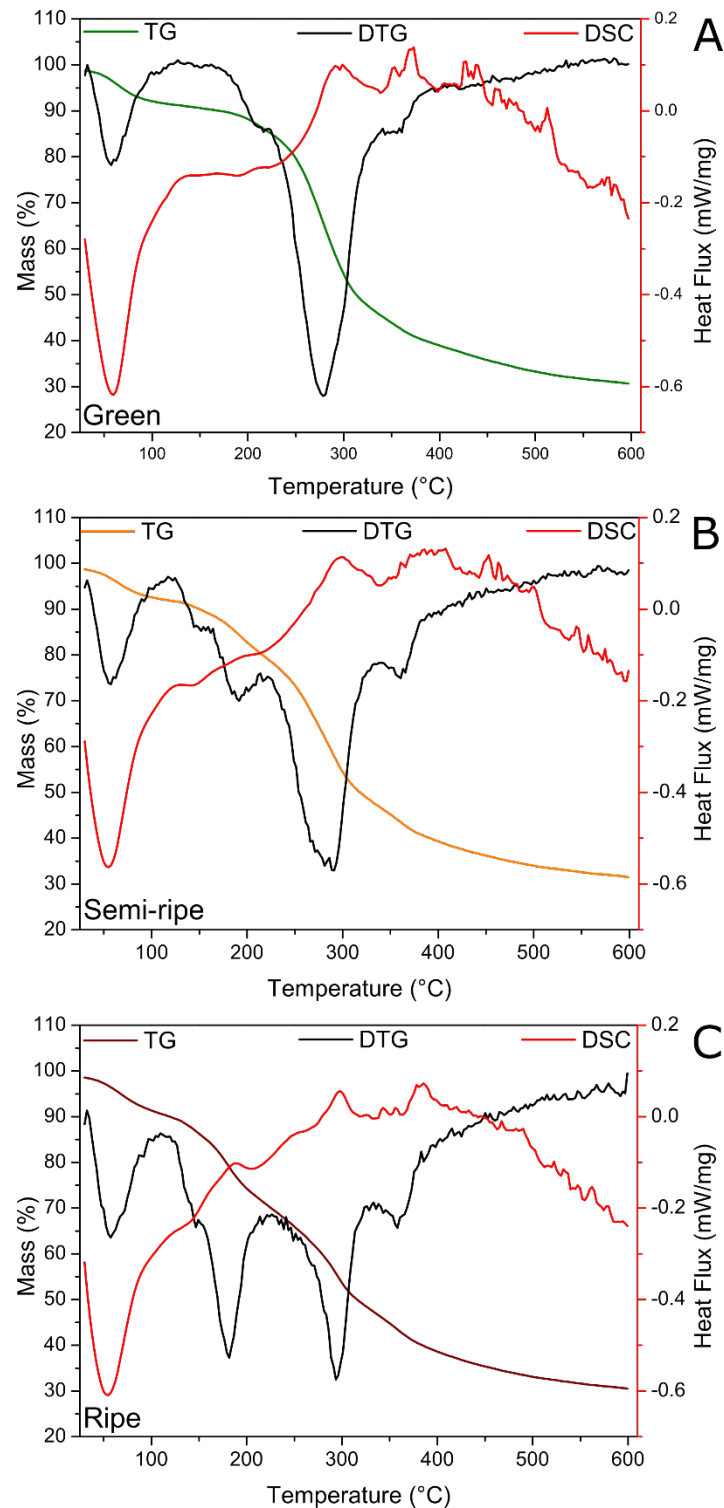
Figure 3. TG, DTG, and DSC curves of the green (a), semi-ripe (b), and ripe (c) BPP biosorbents. The measurements were performed under an N 2 atmosphere with a 5 °C/min heating rate. The DTG scale was normalized and omitted for easy visualization of the superposed graphs.
