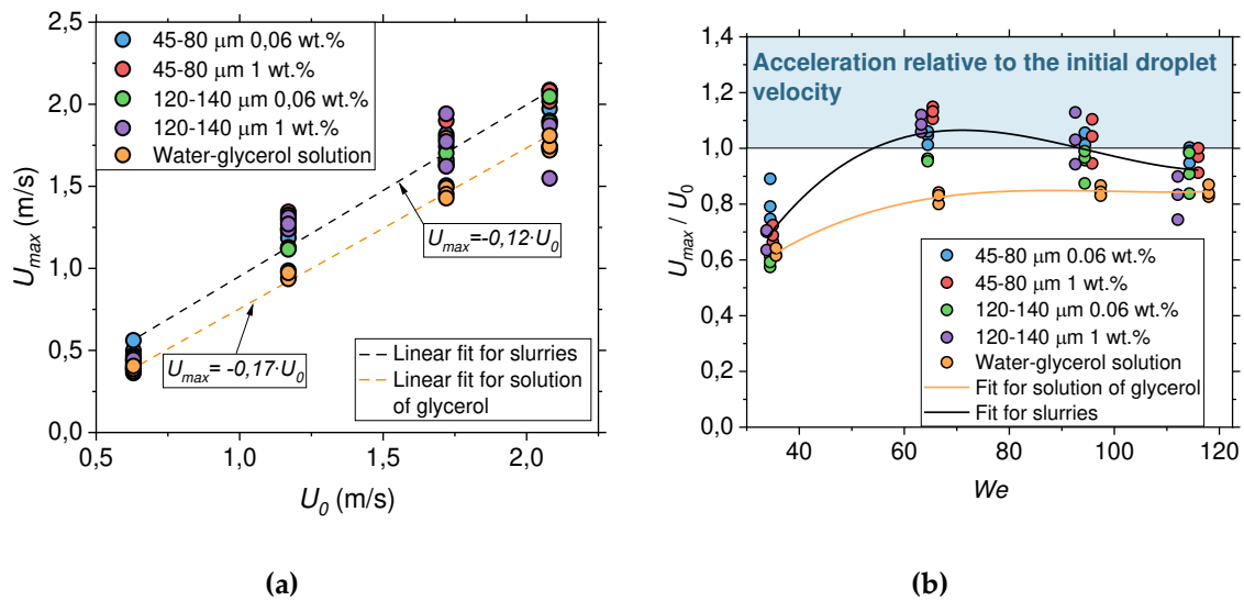
Figure 7. Maximum absolute velocities of internal flows in a drop U_{max} as a function of the initial velocity of the drop before impact U_0 (a), parameter U_{max} / U_0 as a function of We (b).
