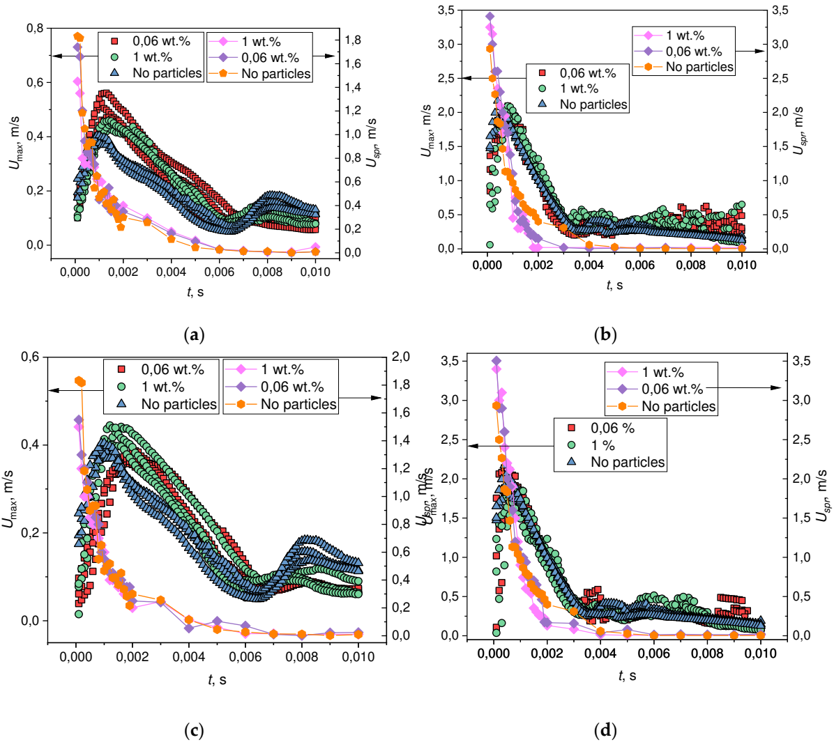
Figure 5. Effect of the Weber number and the concentration of coal particles on the distributions of the instantaneous maximum velocity of fluorescent microparticles in a drop over the spreading time: (a) – grinding fineness of coal particles 45-80 \mu m , We = 30 ; (b) – 45-80 \mu m , We = 120 ; (c) – 120-140 \mu m , We = 30 ; (d) – 120-140 \mu m , We = 120 . The confidence intervals for the experimental data were no more than 3.3%.
