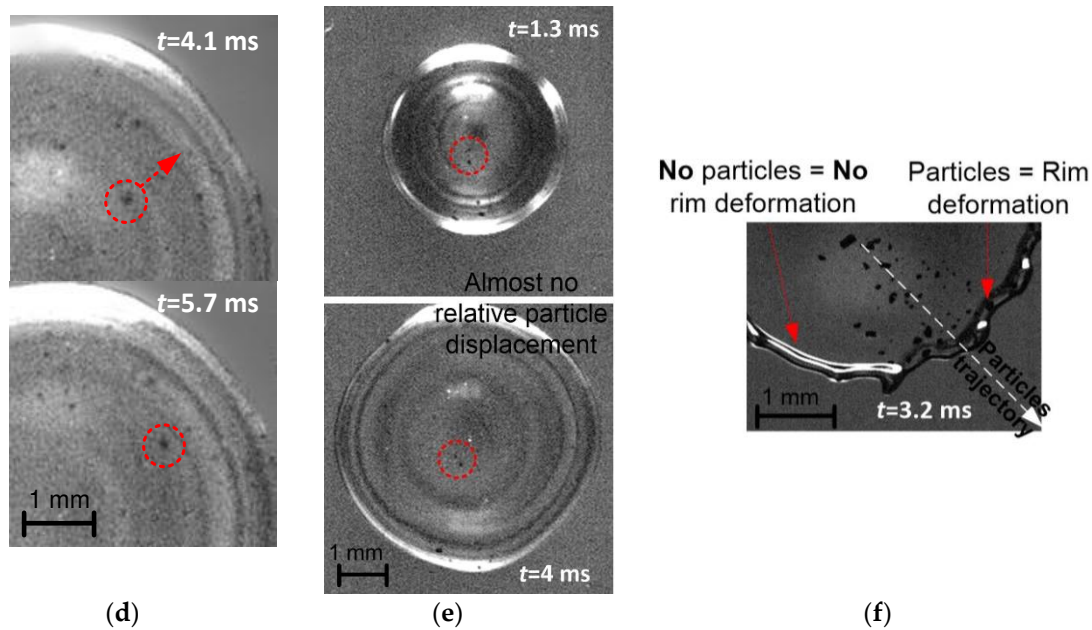
Figure 6. Frames of the forming rim during the Slurry 4 drop spreading with a particle concentration of 1 wt.% and a grinding fineness of 120-140 \mu\text{m} at We=120 and t=1.3 ms (a), We=30 and t=3 ms (b); frame illustrating the appearance of a Slurry 2 drop with a particle concentration of 1 wt.% and a grinding fineness of 45-80 \mu\text{m} at We=120 and t=0.6 ms (c); frames illustrating the relative acceleration of a single coal particle in a drop of Slurry 1 (d); frames illustrating coal particles deposited at the liquid-substrate interface during most of the Slurry 3 drop spreading (e); frame of the mechanical deformation of the Slurry 4 drop rim due to perturbation by coal particles (f).
