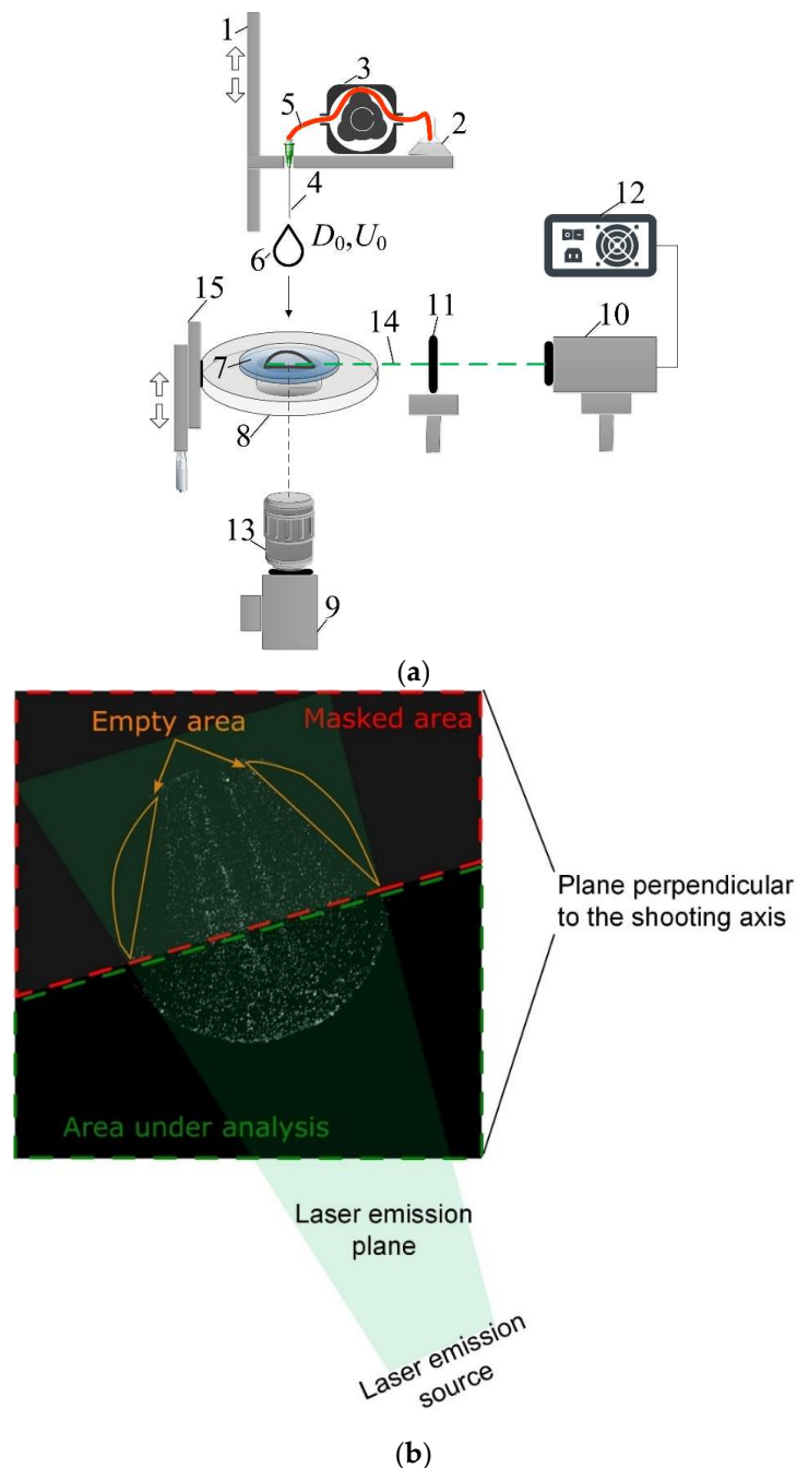
Figure 1. (a) Scheme of the experimental set-up for the implementation of the PIV method: 1 – linear displacement module; 2 – test tube with a liquid; 3 – peristaltic pump; 4 – hollow needle-nozzle; 5 – silicone feed tube; 6 – liquid drop; 7 – optically transparent substrate; 8 – a platform with a through hole for placing the substrate. 9 – high-speed CMOS video camera; 10 – continuous DPSS laser; 11 –
