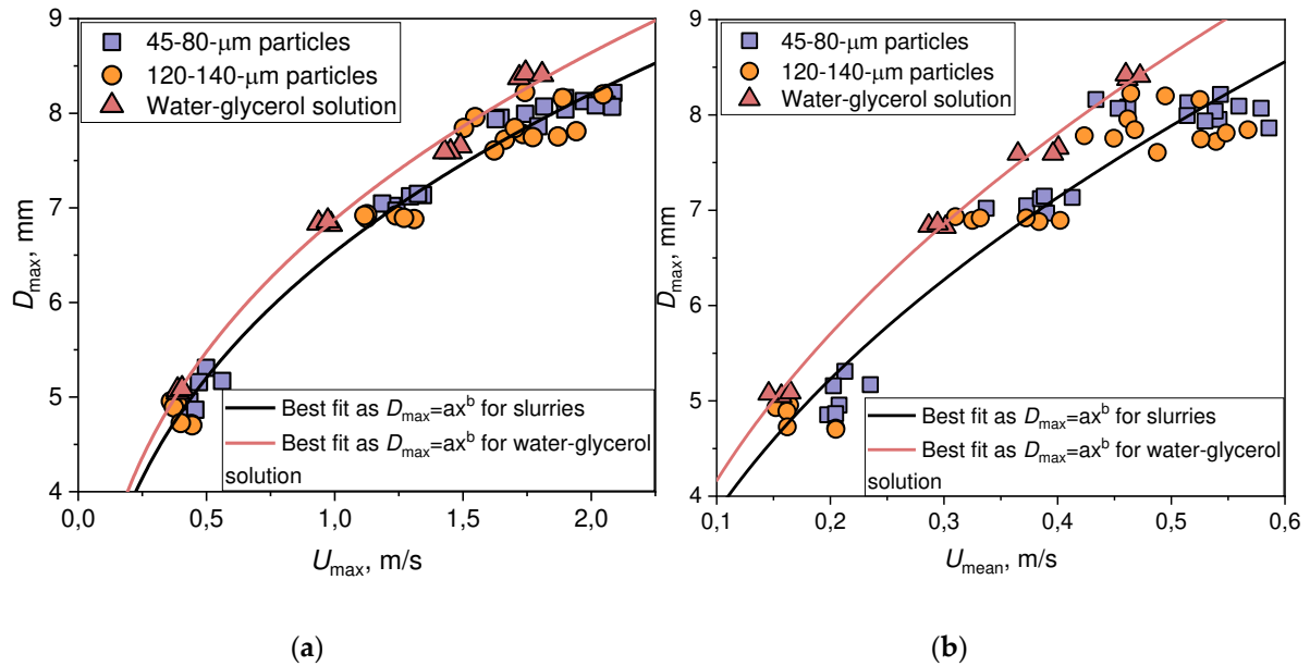
Figure 9. Effect of U_{max} (a) and U_{mean} (b) on the maximum spreading diameter at different grinding fineness of coal particles.
