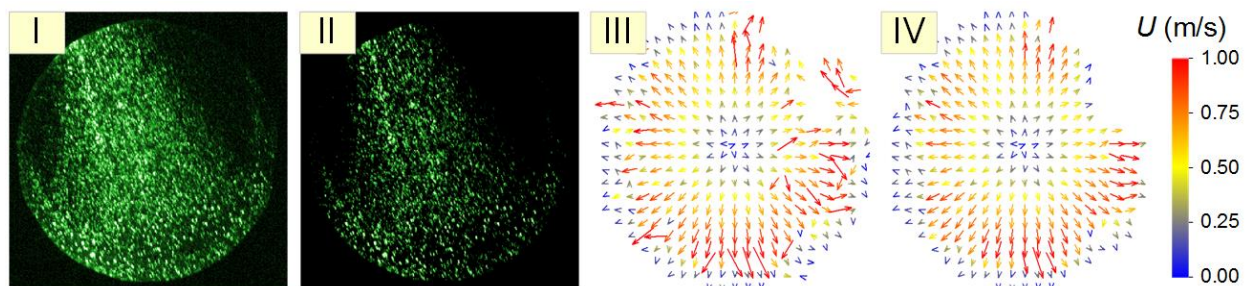
Figure 2. Illustration of the image processing and construction of convective flow velocity fields: I – primary image; II – image after subtracting the background intensity; III – instantaneous velocity field; IV – instantaneous velocity field after the vector interpolation procedure.
