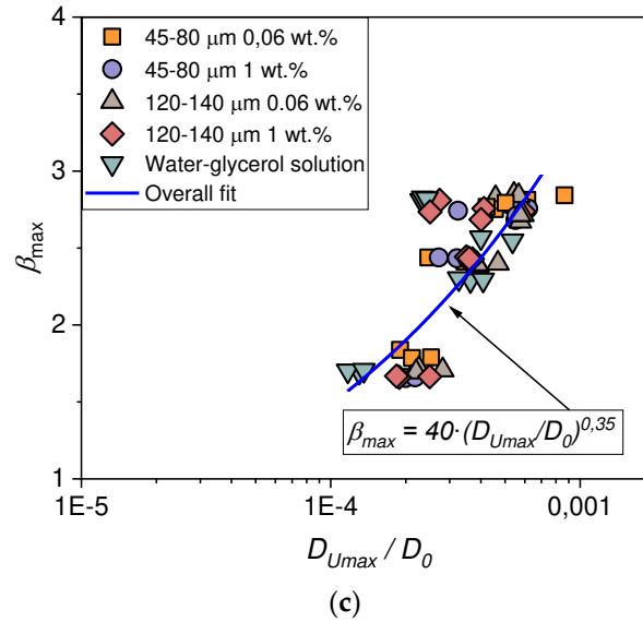
Figure 8. Maximum spreading factor \beta_{max} and time to reach the maximum spreading diameter t_{max} for the considered liquids at We=30, 60, 90, and 120 (a); values of \beta_{max} as a function of We (b); values of \beta_{max} as a function of the dimensionless diameter of the spreading drop at the maximum velocity of internal flows D_{Umax} / D_0 .
