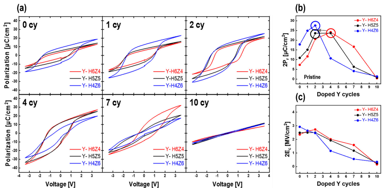
Figure 4. Polarization-voltage ( P-V ) hysteresis curves of as-deposited Y-HZO thin films according to Y-doping cycle. (b) Variation of remanent polarization ( 2P_r ) values of as-deposited Y-HZO thin films according to Y-doping cycle. (c) Variation of coercive field ( 2E_c ) values of as-deposited Y-HZO thin films according to Y-doping cycle.
