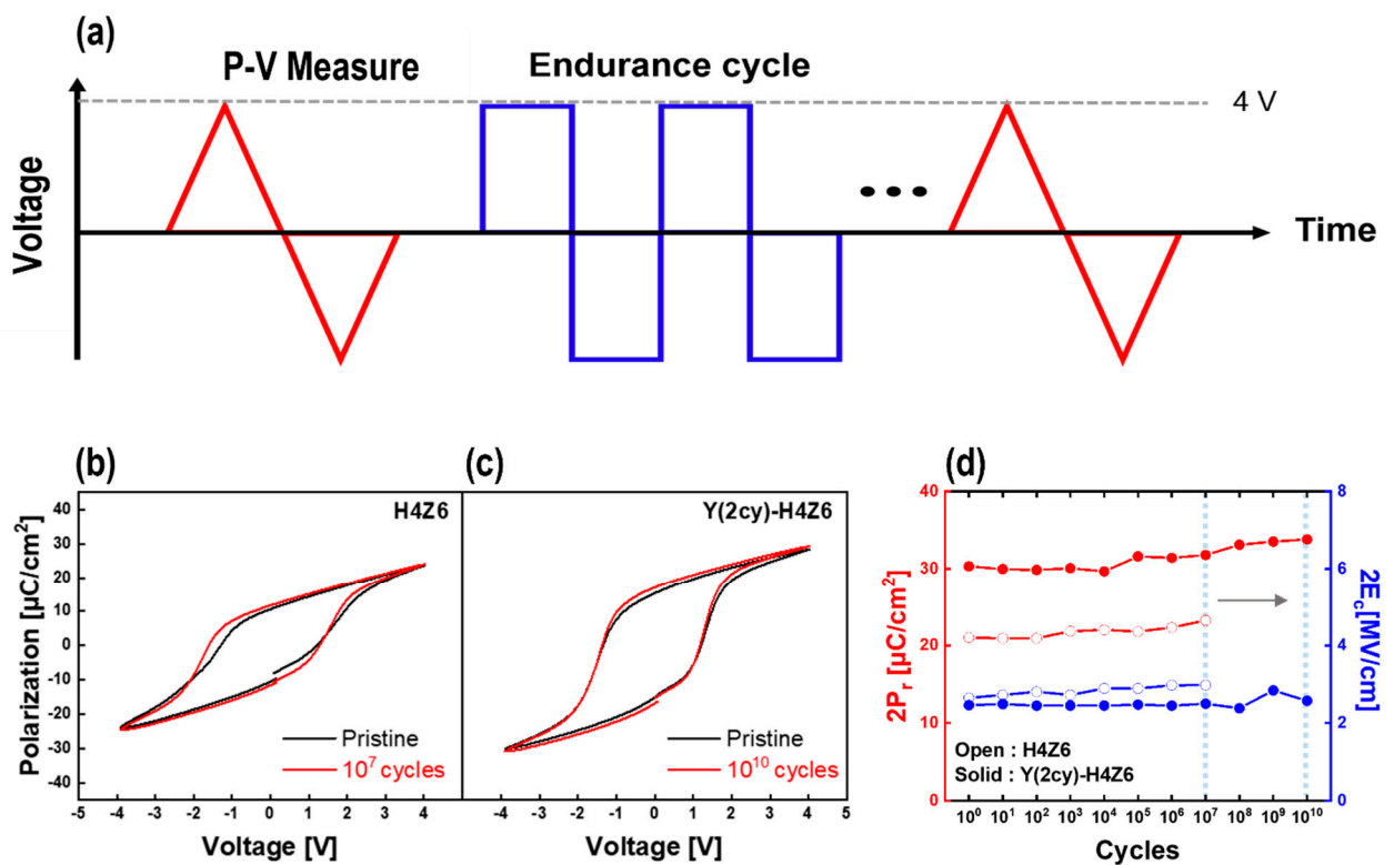
Figure 6. Schematic of the pulse for the endurance test. Polarization-voltage (P-V) hysteresis curves of (b) as-deposited H4Z6 thin films for the pristine state and the state after 10^7 cycles and (c) as-deposited Y(2cy)-H4Z6 thin films for the pristine state and the state after 10^{10} cycles (d) Variation of remanent polarization ( 2P_r ) and coercive field ( 2E_c ) values according to endurance cycles.
