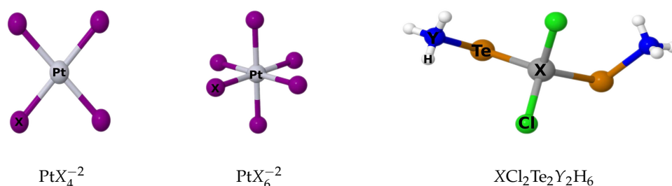
Figure 1. Representation of the molecular structures for \text{PtX}_4^{-2} , \text{PtX}_6^{-2} ( X = \text{Cl}, \text{Br}, \text{I} ), and \text{XCl}_2\text{Te}_2\text{Y}_2\text{H}_6 ( X = \text{Cd}, \text{Hg}; Y = \text{N}, \text{P} ) systems.
