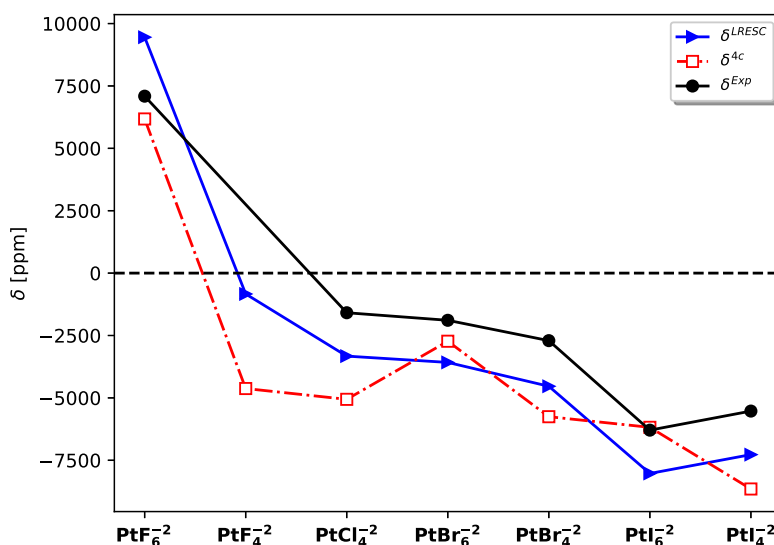
Figure 2. Chemical shift results for platinum, \delta(\text{Pt}) , calculated at LRESC and 4c-RPA levels. Experimental values are also included. All values are given in ppm.
