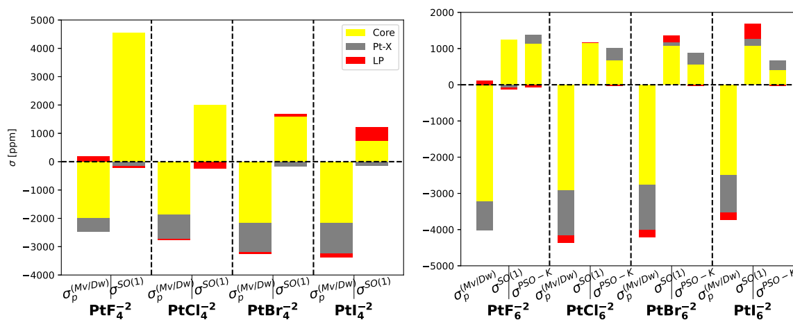
Figure 3. Contributions of core orbitals, bond orbitals, and lone-pair orbitals to the \sigma_p^{(Mv/Dw)} and \sigma^{SO(1)} mechanisms on Pt in PtX_4^{-2} (left) and PtX_6^{-2} (right) molecules. The \sigma^{PSO-K} mechanism is also displayed for PtX_6^{-2} .
