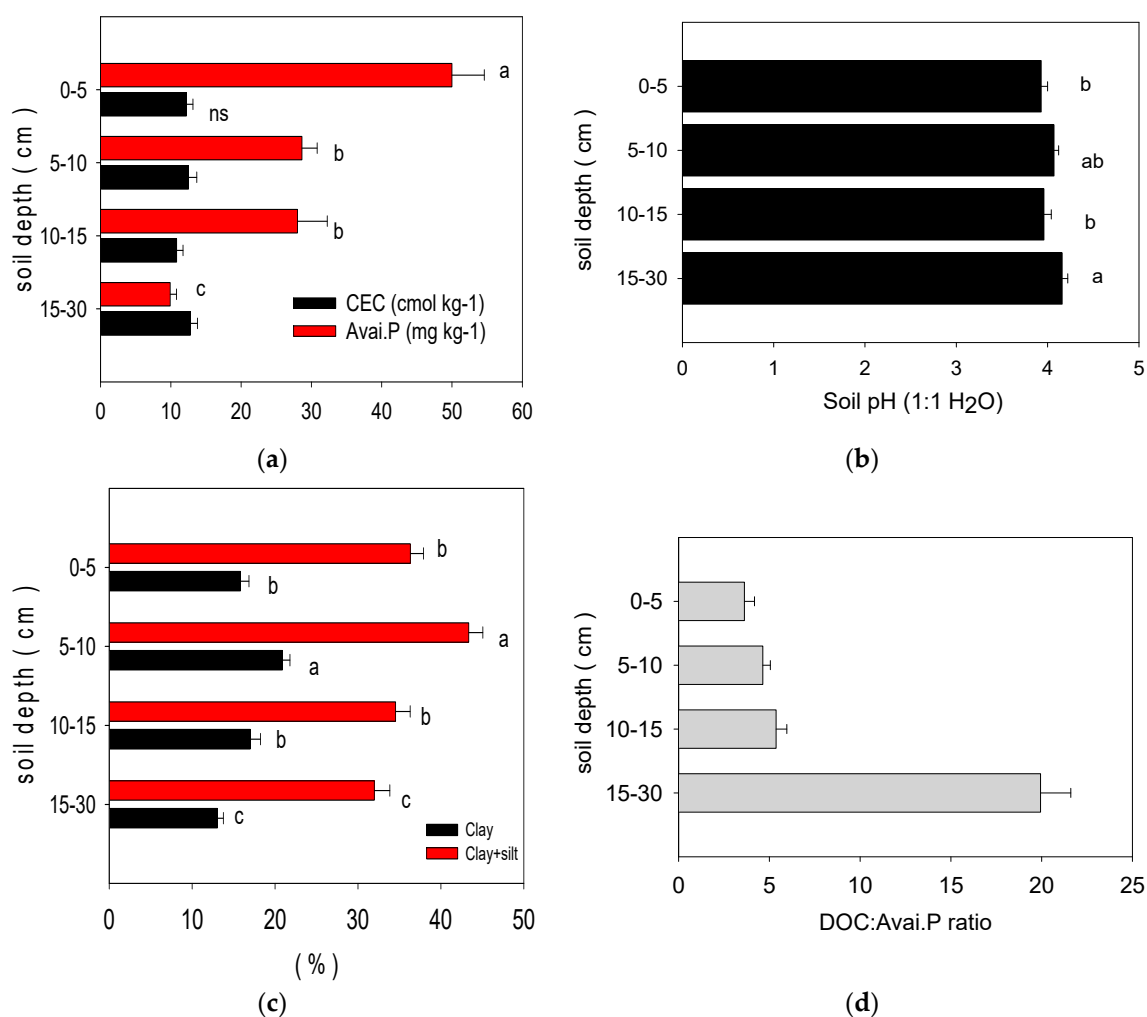
Figure 4. Physiochemical properties of paddy soil at various soil depths: CEC and Avai. P (a), Soil pH (b), Clay and silt (c), and DOC/Avai. P ratio. Note: There were substantial differences between the selected soil depths (0–5 and 10–15 cm), as shown by the differences in the latter ( P<0.05 ). The lines above the bars represent the standard error. CEC = cation exchange capacity (1 N \text{NH}_4\text{OAC} pH =7), where P is available phosphorus assessed using the Bray II method, pH = soil pH (1:1 \text{H}_2\text{O} ), clay and silt are percentages of clay and silt content, and DOC/P is the ratio of DOC to P.
