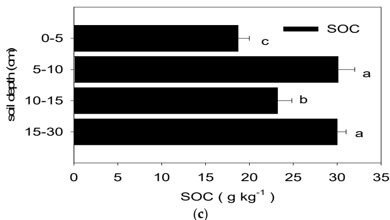
Figure 2. The WSC, HWSC, and DOC (a), POXC (b), and SOC (c) at different soil depths. Note: Differences in soil depth across the latter means are significant ( P < 0.05 ). The lines above the bars represent the standard error. SOC = soil organic carbon, POXC = permanganate oxidizable carbon, HWSC = hot water-soluble carbon, DOC = dissolved organic carbon.
