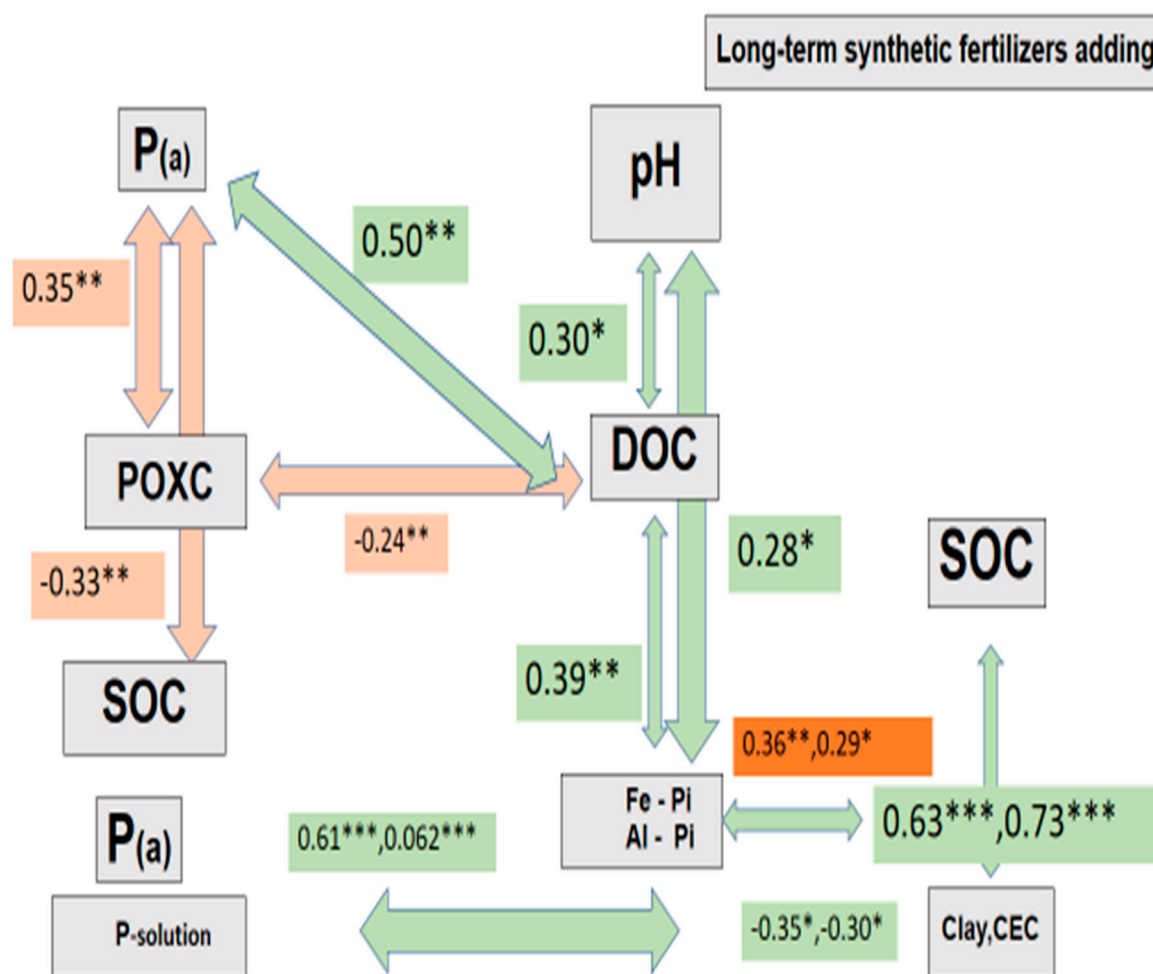
Figure 8. The effect of long-term synthetic fertilization on the changes in SOC and C dynamics in the paddy soil. Note: The numbers in the boxes indicate the relationships between the correlation coefficients of the indicators. Solution-P was extracted using 0.1 M \text{NH}_4\text{Cl} , Al-P was extracted using 0.5 M \text{NH}_4\text{F} , and Fe-P was extracted using 0.1 M \text{NaOH} . Re.So.P = Reductant soluble P was extracted using a mixture of \text{Na}_3\text{C}_3\text{H}_6\text{O}_7 , \text{NaHCO}_3 , and \text{Na}_2\text{S}_2\text{O}_4 , and Ca-P was extracted using 0.25 M \text{H}_2\text{SO}_4 . SOC, soil organic carbon; WSC, water soluble carbon; HWSC, hot water-soluble carbon; DOC, dissolved organic carbon; POXC, permanganate oxidizable carbon; Avai. P, available phosphorus; pH, soil pH; CEC, cation exchange capacity; clay and silt, percentages of clay and silt. The numbers in the green boxes varied between the datasets 0–5 and 10–15 cm, while the numbers in the orange boxes came from a 0–30 cm soil depth dataset.
