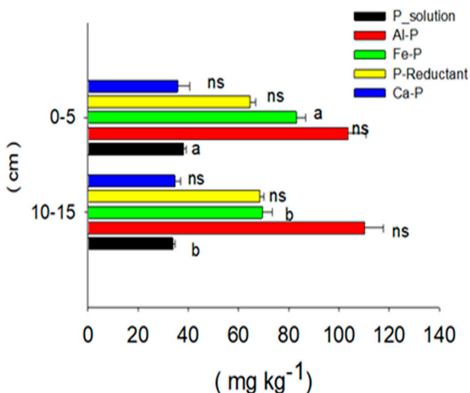
Figure 3. The fractionation of inorganic phosphorus in conventional paddy soil at specific soil depths between 0–5 and 10–15 cm. Note: There were substantial differences between the selected soil depths (0–5 and 10–15 cm) between the small case and bar ( P < 0.05 ). The lines above the bars represent the standard error. P-solution was extracted using 0.1 M \text{NH}_4\text{Cl} , Al-P was extracted using 0.5 M \text{NH}_4\text{F} , and Fe-P was extracted using 0.1 M \text{NaOH} . Red-So-P = Reductant soluble P was extracted using a mixture of \text{Na}_2\text{C}_2\text{O}_4 , \text{NaHCO}_3 , and \text{Na}_2\text{S}_2\text{O}_4 . and Ca-P was extracted using 0.25 M \text{H}_2\text{SO}_4 .
