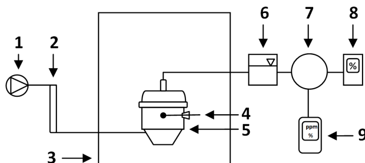
Figure 2. Laboratory scale composting system (based on [16]): 1 – air supply, 2 – flowmeter, 3 – climate chamber, 4 – thermocouple, 5 – bioreactor, 6 – cooling system, 7 – puffer bag, 8 – IR gas analyzer (CO 2 , % v/v), 9 – gas concentration analyzer (CO, ppm; O 2 , % v/v).
