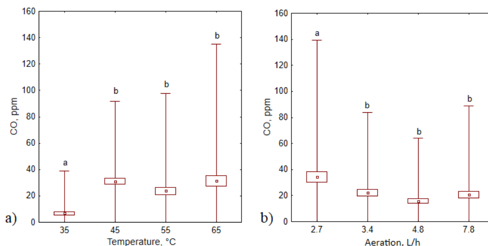
Figure 6. Average CO concentration ( \pm standard deviation) during 14 days of composting process in (a) different temperature variants, and (b) different aeration variants; letters (a, b) indicate homogeneity group according to Tukey's test at the significance level p < 0.05 .
