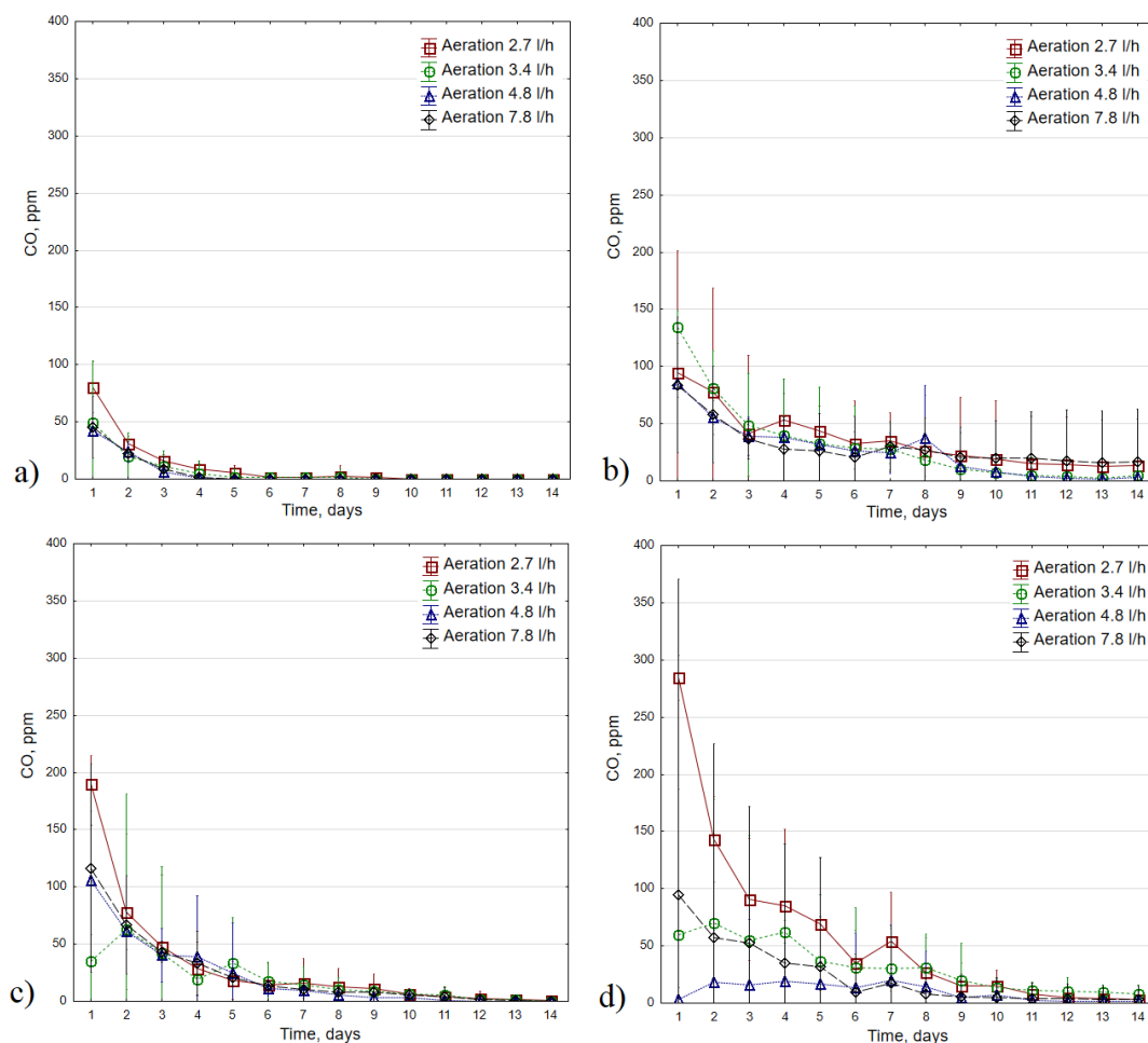
Figure 5. CO concentration average values ( \pm standard deviation) during 14 days of composting process in different temperature variants: (a) 35°C; (b) 45°C; (c) 55°C; (d) 65°C.
