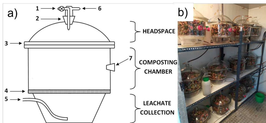
Figure 1. Bioreactors for laboratory scale composting: (a) scheme of the bioreactor (based on [16]), 1 – closed valve, 2 – covers screw cup, 3 – cover edge, 4 – perforated plastic screen, 5 – aeration hose, 6 – exhaust air outlet, 7 – screw cup for temperature measurements; (b) bioreactors in the climate chamber.
