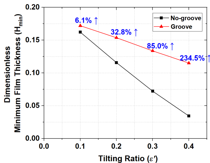
Figure 8. Dimensionless minimum film thickness with shaft tilting ratio ( L = 3.0 , A = 0.4 , L_f = 1/3 , W = 4.4 , \gamma = 1.0 ).
