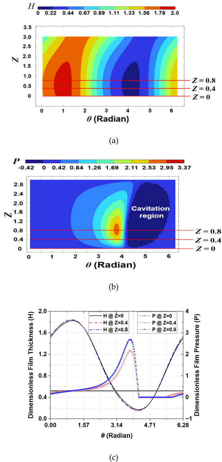
Figure 7. Dimensionless results for journal bearing with flexible structure ( L = 3.0 , A = 0.4 , W = 4.4 , \gamma = 1.0 , \varepsilon' = 0.2 ) (a) film thickness; (b) pressure distribution; (c) circumferential distribution of film thickness and pressure.
