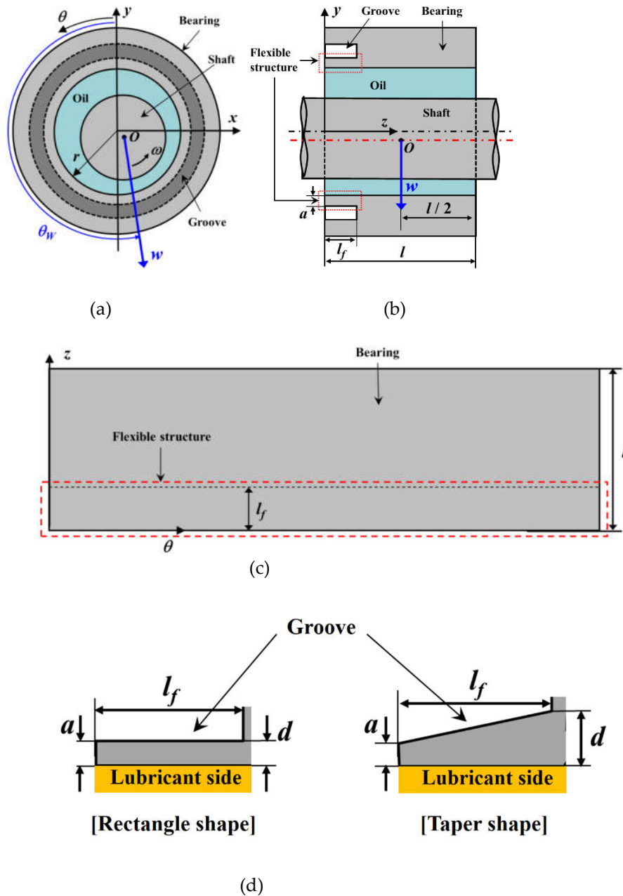
Figure 2. Schematic of journal bearing system (a) x-y plane; (b) y-z plane; (c) \theta - z plane; (d) shapes of the flexible structure.
