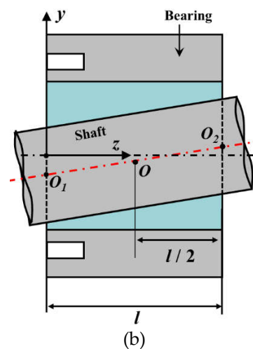
Figure 3. The shaft in bearing with eccentric and tilted motion (a) x-y plane; (b) y-z plane.
