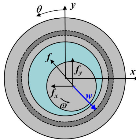
Figure 5. Oil-film force working on the shaft.
