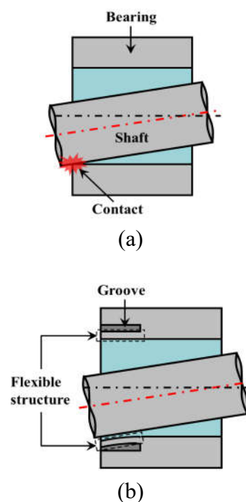
Figure 1. Application of the flexible structure to the misaligned journal bearing (a) without flexible structure; (b) with flexible structure.
