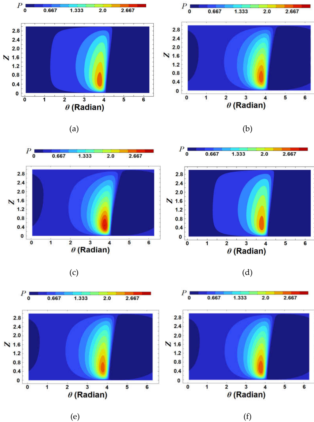
Figure 12. Distributions of the dimensionless oil pressure for \varepsilon' = 0.2 .
