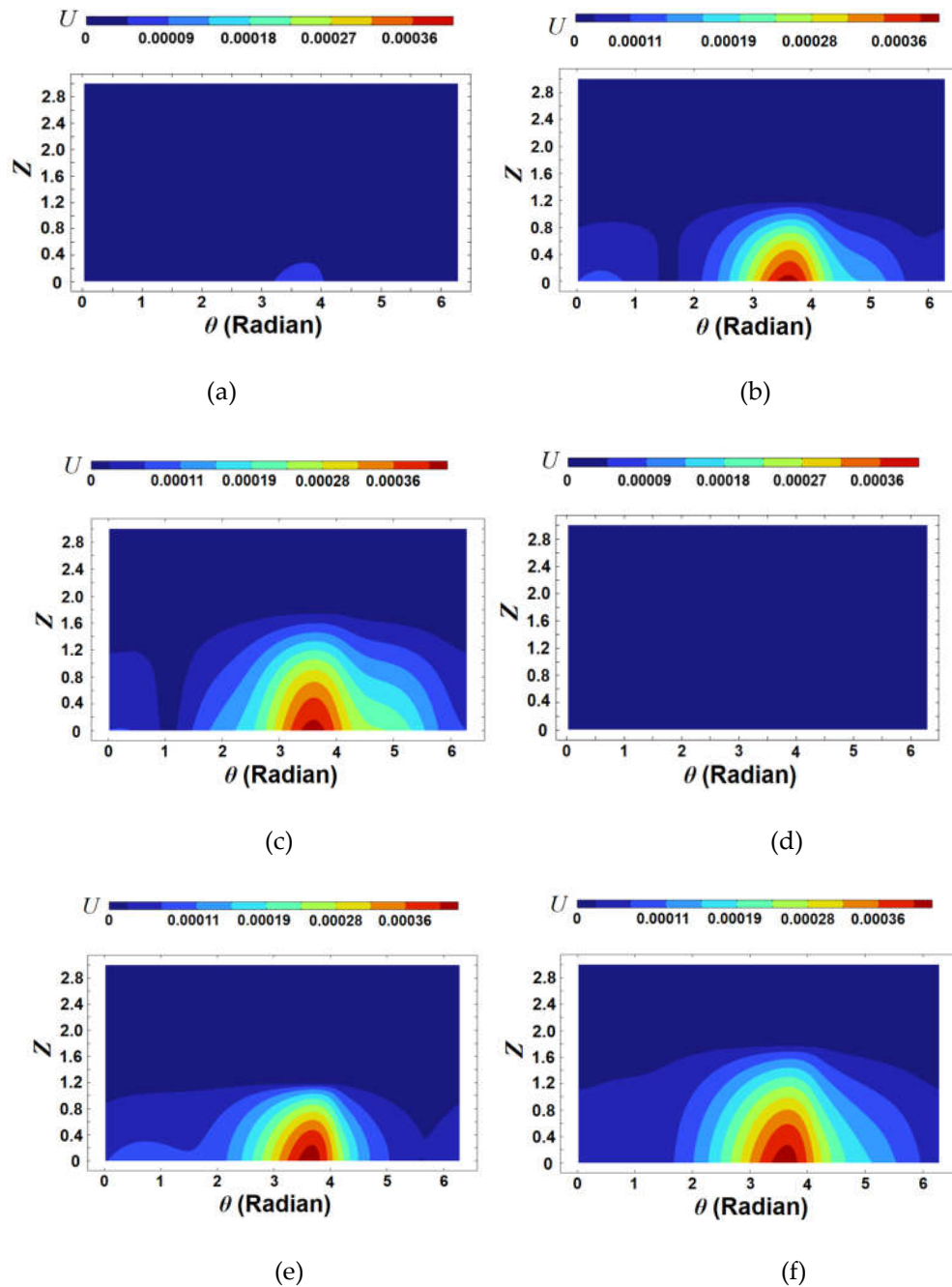
Figure 13. Distributions of the dimensionless deformation for \varepsilon' = 0.2 .
