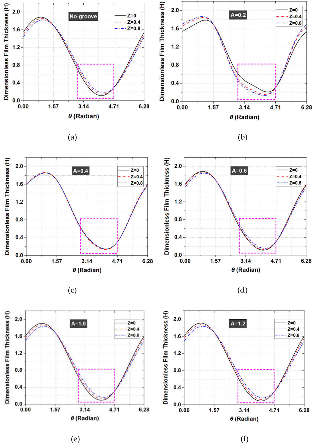
Figure 10. Circumferential distributions of the dimensionless film thickness for different A ( L = 3.0 , L_f = 1/3 , W = 4.4 , \gamma = 1.0 , \varepsilon' = 0.3 ).
