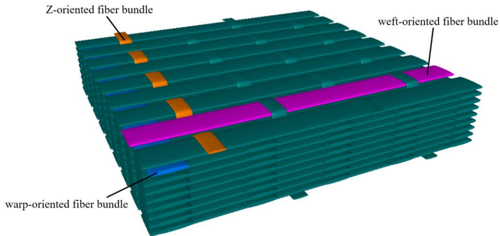
Figure 1. The structure diagram of 3D woven composites
