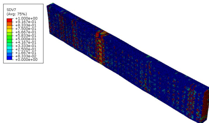
Figure 8. Final damage diagram of finite element model
