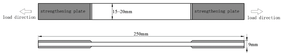
Figure 2. Uniaxial tensile specimen of 3D woven composites
