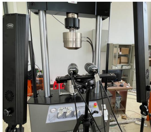
Figure 3. Setup of 3D DIC Technology
