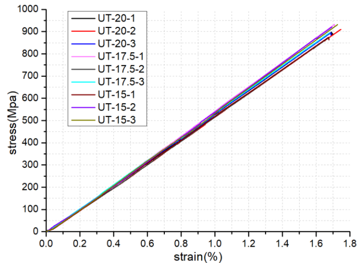
Figure 6. Stress-strain curves of specimens with different widths
