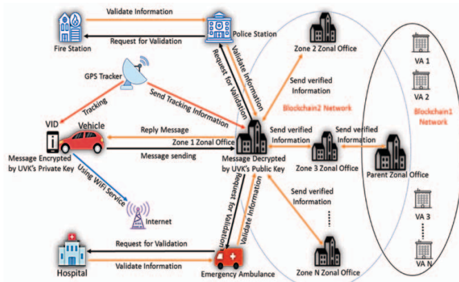
Fig. 3. The secure data communication process between different entities
