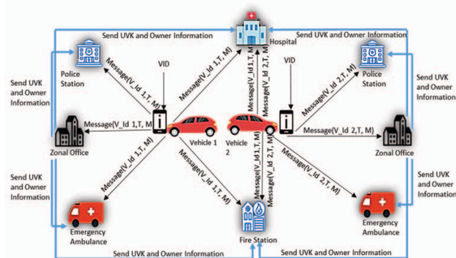
Fig. 2. Message propagation procedure within a zone
