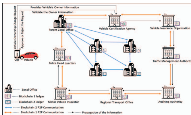
Fig. 1. An overview of the BSIoV framework
