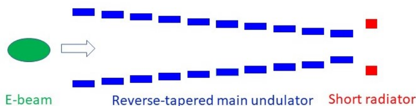
Figure 1. Conceptual scheme of ultrashort pulse production. A short electron bunch propagates in the reverse-tapered main undulator followed by a short radiator.
