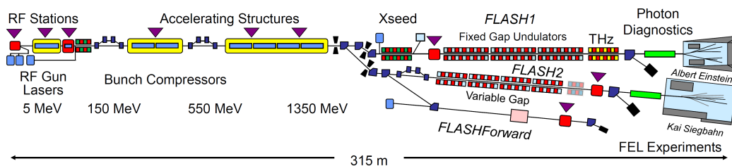
Figure 3. FLASH layout.
