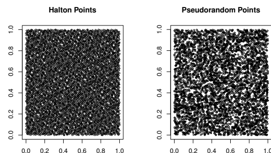
Figure 2. Two-dimensional projection of 5000 Halton and Pseudorandom points
