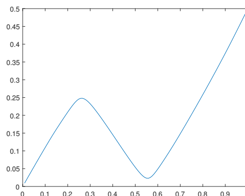
Figure 9. Solution u_0(x) for the example A.
