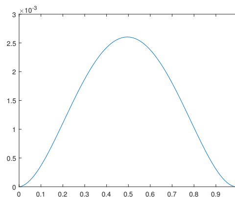
Figure 19. Solution u(x) for the example B.
