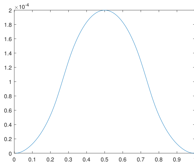
Figure 22. Optimal solution w(x) for a bi-clamped beam.
