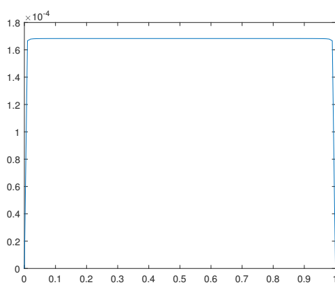
Figure 16. Solution \phi_v(x) for \omega = 1 .
