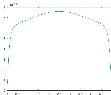
Figure 12. Solution \phi_S(x) for the \omega = 1.8 .
