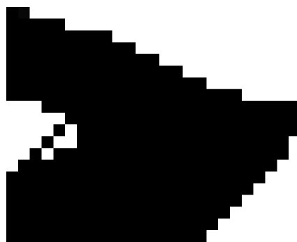
Figure 5. Density t(x, y) for the Case A.
