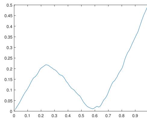
Figure 30. Optimal solution u_0(x) for the case f(x) = \cos(\pi x)/2 .
