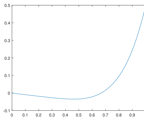
Figure 1. solution u_0(x) for the case f(x) = 0 .
