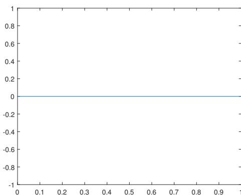
Figure 17. Solution \phi_u(x) for \omega = 15 .
