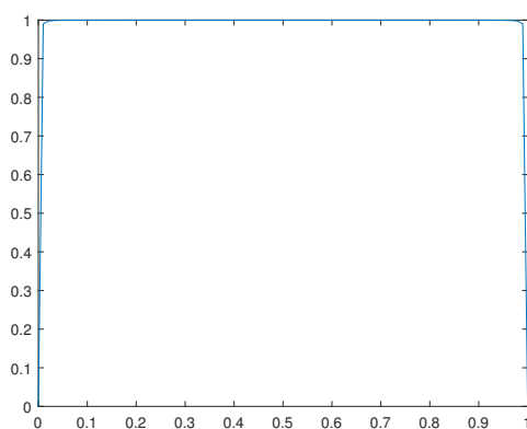
Figure 15. Solution \phi_u(x) for \omega = 1 .
