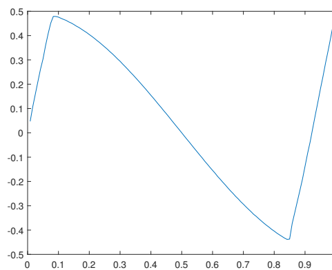
Figure 10. Solution u_0(x) for the example B.
