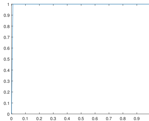
Figure 18. Solution \phi_v(x) for \omega = 15 .
