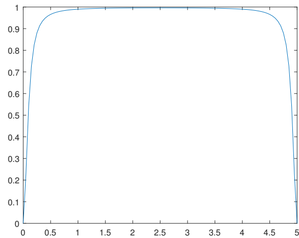
Figure 11. Solution \phi_N(x) for the \omega = 1.8 .
