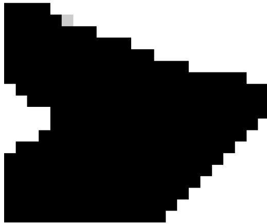
Figure 40. Optimal shape \lambda_1(x, y) for the beam of case A.
