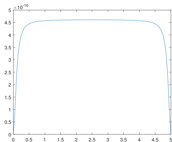
Figure 13. Solution \phi_N(x) for the \omega = 1.0 .
