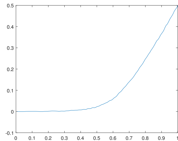
Figure 31. Optimal solution u_0(x) for the case f(x) = 0 .
