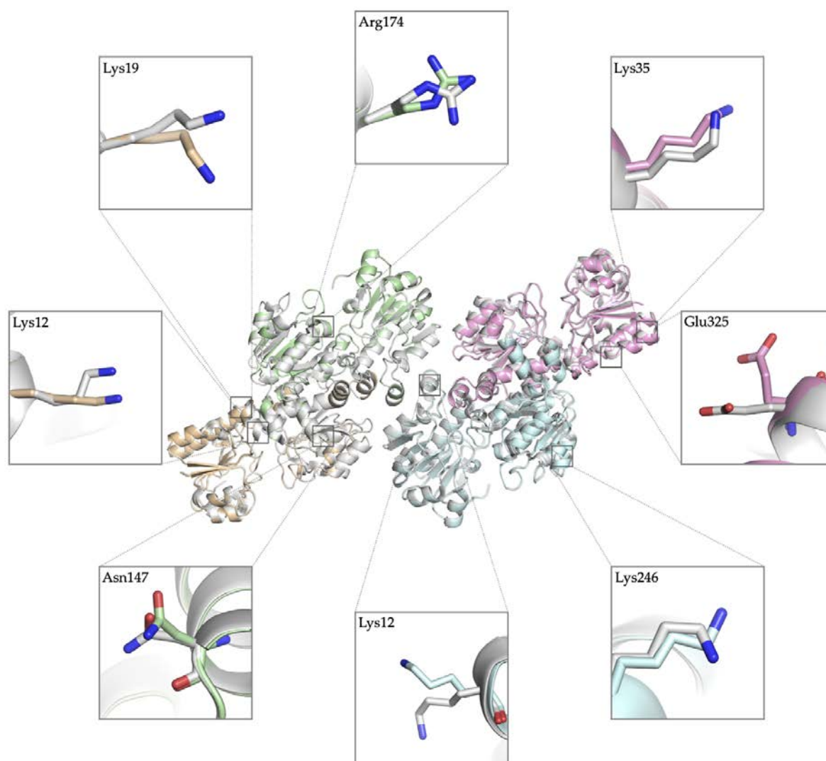
Figure 4. Superposition of two apo wild-type CbFDH structures. Our 1.4 Å structure is shown in four distinct colors indicating each chain; A: pale green, B: wheat, C: pink, D: pale cyan. 5DNA is colored gray. Conformational differences in side chains are shown in boxes in stick representation.
