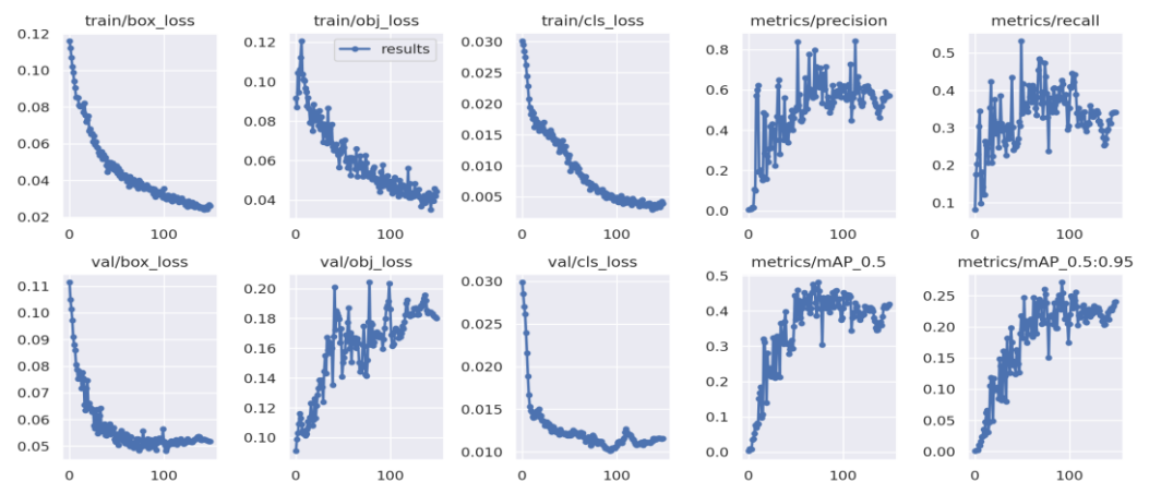
Figure 44. Setup output results using the YOLOv5s algorithm.
