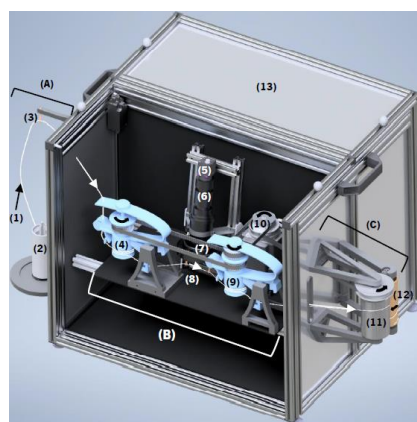
Figure 27. Mechatronic system developed.
