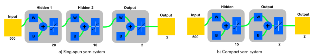
Figure 9. The tenacity and % elongation architectures of the neural network: a) Ring yarn system (left), b) Compact yarn system (right) (Adapted from [9]).
