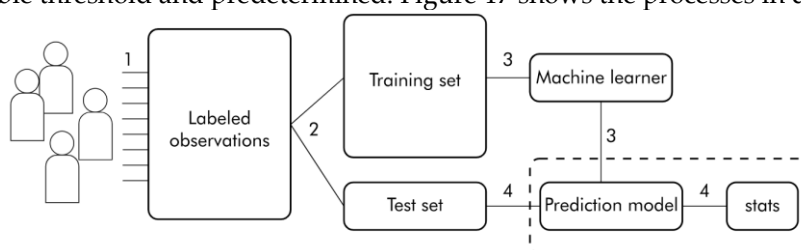
Figure 17. Supervised Learning. Steps: (1) made annotations in the dataset; (2) dataset separation; (3) algorithm training; (4) Dataset test for algorithm evaluation and performance (Adapted from [24]).
