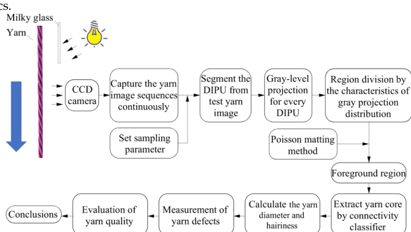
Figure 1. Flowchart of the method for detecting yarn parameters and evaluating yarn quality (Adapted from [3]).
