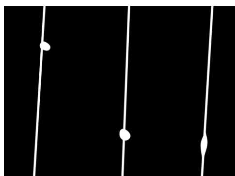
Figure 4. An example of a yarn image with a nep defect obtained using the image acquisition system (Adapted from [7]).
