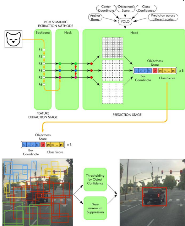
Figure 23. Yolo architecture and how it works (Adapted from [30,31]).
