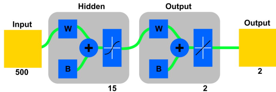
Figure 6. Cotton threads: the architecture of neural network traction properties (Adapted from [8]).
