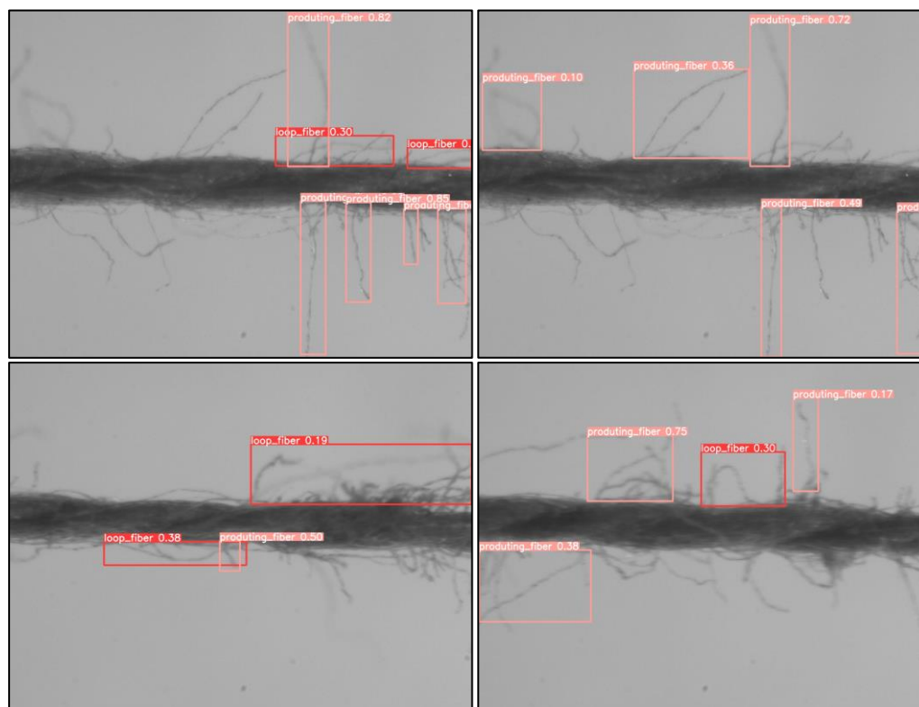
Figure 45. Classification results using the YOLOv5s algorithm.
