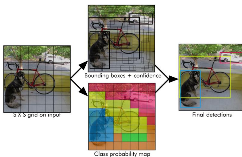
Figure 22. YOLO models the detection as a regression problem. It splits the image into an S \times S grid and for each cell of the grid predicts bounding boxes B , confidence for those boxes (thicker lines, higher confidence) and class C probabilities. These predictions are encoded as a tensor S \times S \times (B * 5 + C) (Adapted from [28,29]).
