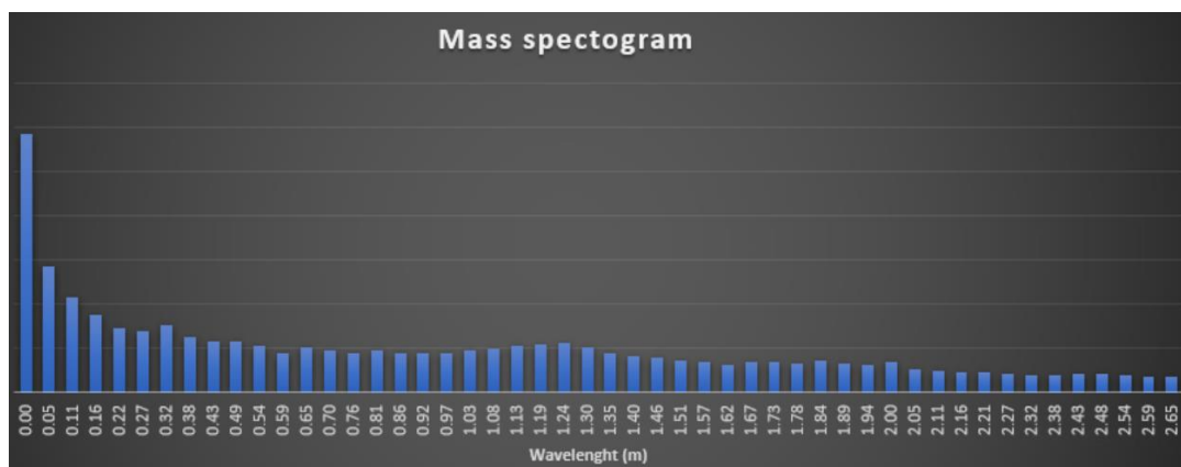
Figure 38. Mass spectrogram.
