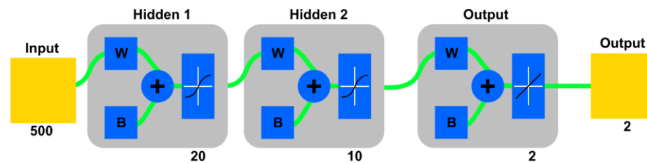
Figure 7. Mixed yarns: the structure of neural network traction properties (Adapted from [8]).
