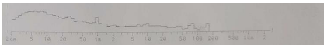
Figure 39. Mass spectrogram graphic obtained by the USTER Tester 3.
