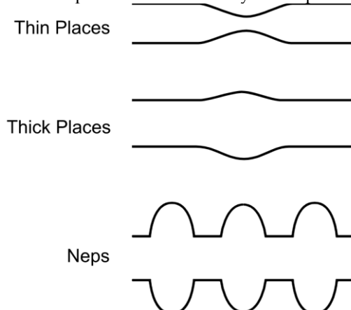
Figure 14. Types of dimensional imperfections (Adapted from [16]).
