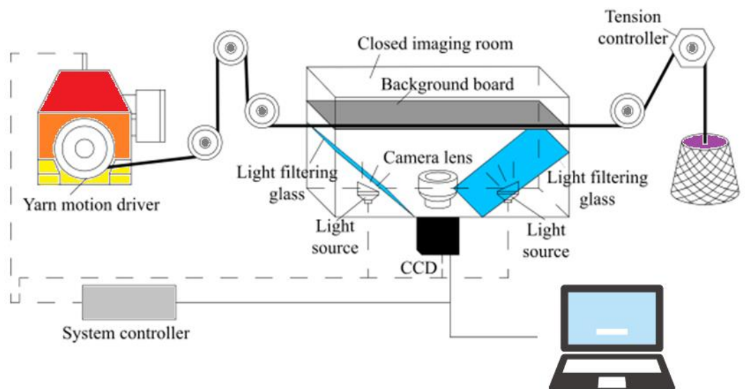
Figure 2. System device to detect yarn parameters (Adapted from [3]).
