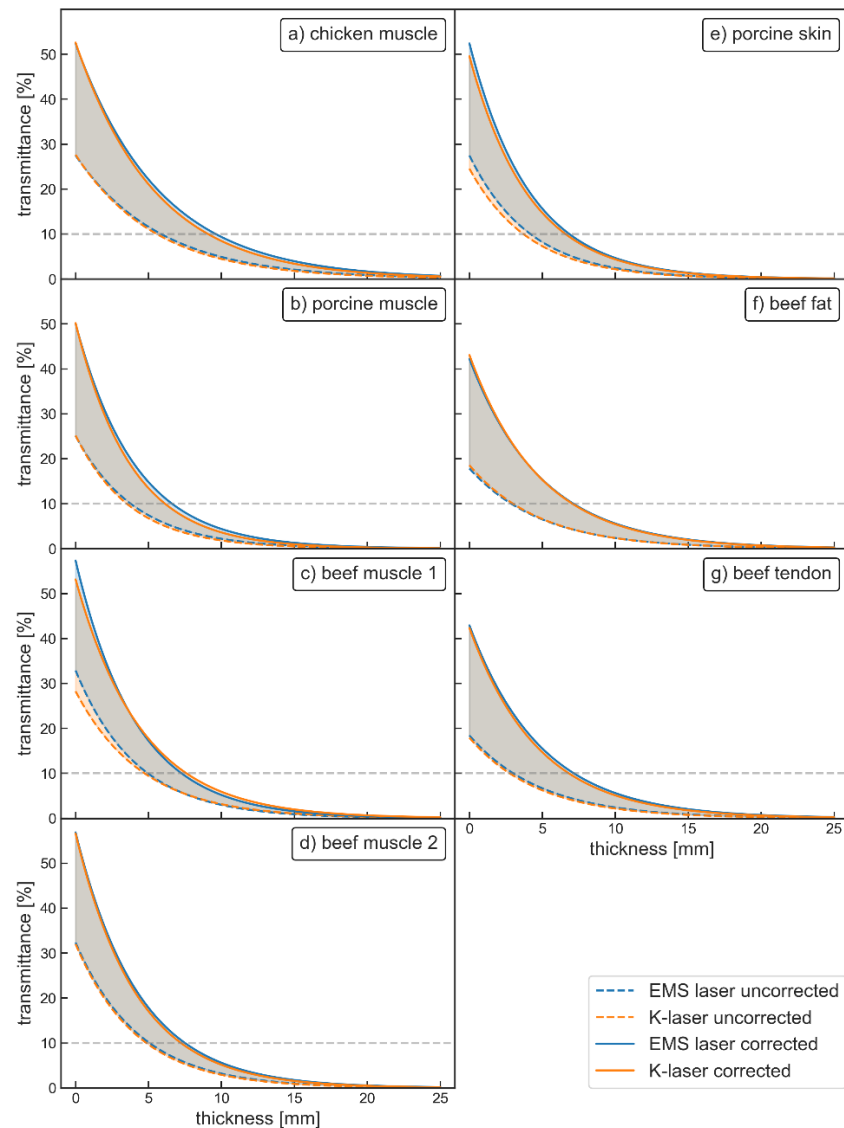
Figure 5. Transmittance curves before and after correction. The transmittance in percent is plotted against the tissue thickness in millimeters. While the uncorrected curves are the same as in Figure 4, the corrected curves were here added as solid lines. The areas between the uncorrected and corrected curves are filled with the according color of the laser therapy device. This area gives the range of what are most likely the true transmittance values. Dotted gray lines represent the 10% penetration depths.
