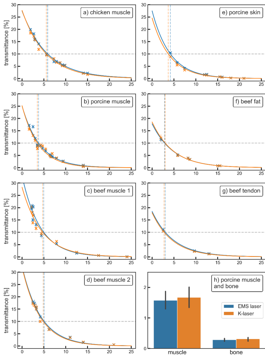
Figure 4. Results of penetration depth measurements. Transmittance in percent is plotted against the tissue thickness in millimeters for the EMS laser (blue dots and blue lines) and the K-laser (orange dots and orange lines) (a-g). In addition, bone tissue and muscle tissue were compared for a fixed thickness of 15 mm (h). Measurements were performed with muscle tissue specimens (a-d) and with non-muscular tissue specimens (e-g) from different animal species. Each point represents the average of seven measurements; the according standard deviations are indicated by vertical lines. Solid lines represent best fitting transmittance curves. The 10% penetration depth is illustrated by dashed vertical lines in the color of the according laser therapy device.
