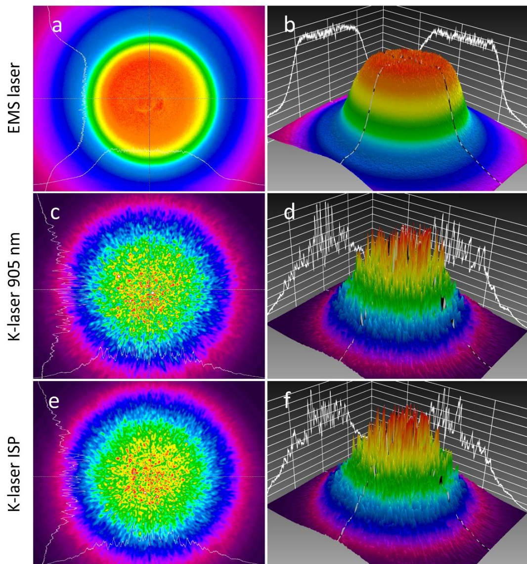
Figure 2. Power density maps recorded with a beam profiling camera for the EMS laser ( a, b ), the K-laser using 905 nm wavelength ( c, d ), and the K-laser operated in ISP mode ( e, f ). Two-dimensional power density maps ( a, c, e ) are shown as well as three-dimensional representations ( b, d, f ). White lines in both representations are beam profiles along the x- and y-axis. Maps were normalized to the maximum intensity of each recording.
