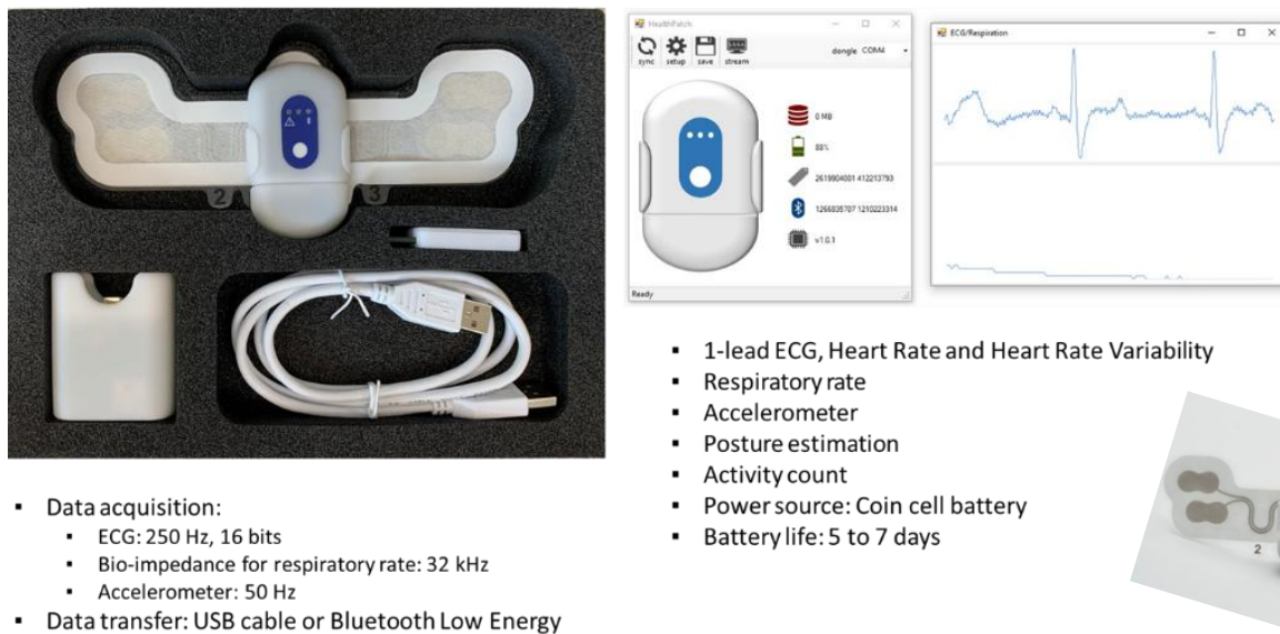
Figure 1: Photo of the Portable 3-in-1 Sensor Patch. Source: TNO Holst Centre, Eindhoven, The Netherlands
