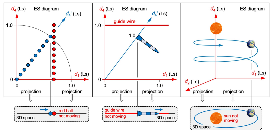
Fig. 4 Solving three instructive problems. Each snapshot shows one instant in cosmic time. Only the left ES diagram shows ten snapshots at once. Left: The blue ball is hit toward the red ball. In the projection, the two balls collide after one second even if their d_4 values do not match. Center: Some rocket moves along a guide wire. In the projection, the wire does not escape from the rocket. Right: Earth orbits the sun. In the projection, the sun does not escape from the orbital plane
