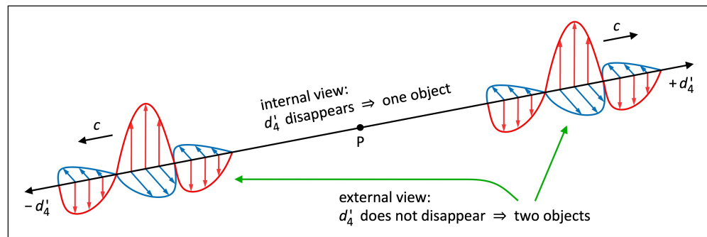
Fig. 8 Solving non-locality in ER. For an observer moving in any direction other than \pm d'_4 (external view), the wavematters moving in \pm d'_4 are two distinct objects. For each wavematter (internal view), the \pm d'_4 axis disappears. They are one object that has never been separated
