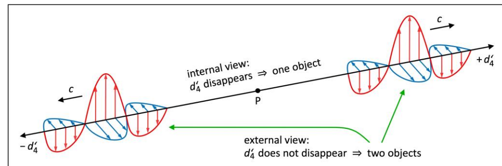
Fig. 7 Solving non-locality in ER. For an observer moving in any direction other than \pm d'_4 (external view), the displayed wavematters moving in \pm d'_4 are two distinct objects. For each wavematter (internal view), the \pm d'_4 axis disappears. They are one object that has never been separated
