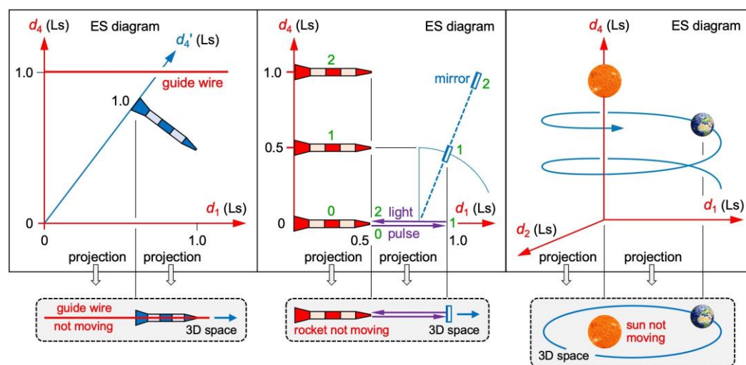
Fig. 4 Graphical solutions to three geometric paradoxes. Left: A rocket moves along a guide wire. In 3D space, the guide wire remains within the rocket. Center: An observer in a rocket tip tries to detect the reflection of a light pulse. Between two snapshots (0–1 or 1–2), rocket, mirror, and light pulse move 0.5 Ls in ES. In 3D space, the light pulse is reflected back to the observer. Right: Earth revolves around the sun. In 3D space, the sun remains in the orbital plane of Earth
