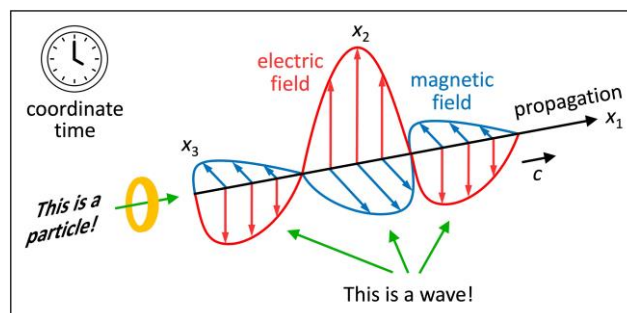
Fig. 6 Artwork illustrating the concept "wavematter". If I observe a wavematter (external view), it may appear as a wave packet or as a particle. As a wave, it propagates and oscillates as a function of coordinate time. In its own reality (internal view), the axis of the wavematter's 4D motion disappears because of length contraction at the speed c . It deems itself particle at rest
