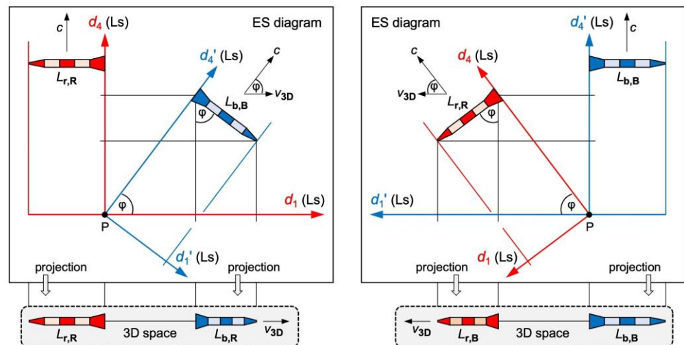
Fig. 2 ES diagrams and 3D projections for two rockets "r" (red) and "b" (blue). Top left and top right: Both rockets move at the speed c but in different directions. Bottom left: Projection to the 3D space of observer R. Rocket "b" moves at the speed v_{3D} and contracts to L_{b,R} . Bottom right: Projection to the 3D space of observer B. Rocket "r" moves at the speed v_{3D} and contracts to L_{r,B}
