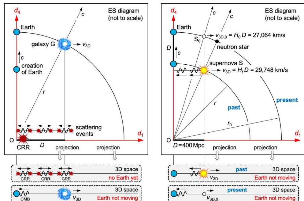
Fig. 5 ES diagrams and 3D projections for solving the mysteries 5.6, 5.7, 5.10, 5.11. The circular arcs are part of an expanding 3D hypersurface. Left: The CMB is CRR that has been scattered in the past. Galaxy G recedes from Earth at the speed v_{3D} . Right: The supernova of star S occurred at a distance D from Earth. If star S_0 is at the same distance D today, it recedes more slowly from Earth than S
