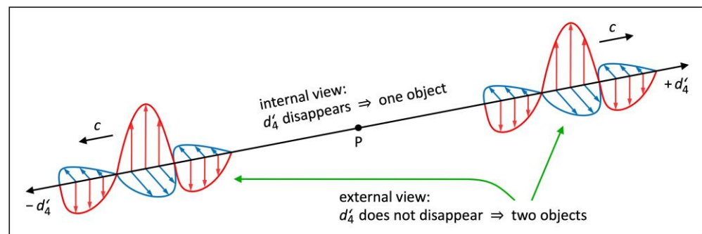
Fig. 8 Solving non-locality in ER. For an observer moving in any direction other than \pm d'_4 (external view), the displayed wavematters moving in \pm d'_4 are two distinct objects. For each wavematter (internal view), the \pm d'_4 axis disappears. They are one object that has never been separated
