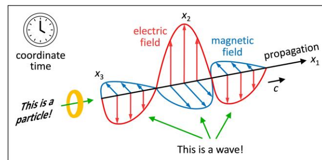
Fig. 7 Artwork illustrating the concept “wavematter”. If I observe a wavematter (external view), it may appear as a wave packet or as a particle. As a wave, it propagates and oscillates as a function of coordinate time. In its own reality (internal view), the axis of the wavematter’s 4D motion disappears because of length contraction at the speed c . It deems itself particle at rest
