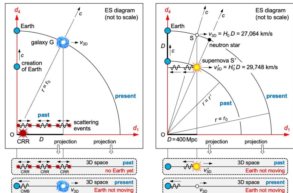
Fig. 5 ES diagrams and 3D projections for solving the mysteries 5.6, 5.7, 5.10, and 5.11. The circular arcs are part of an expanding 3D hypersurface. Left: The CMB is CRR that has been scattered in the past. Galaxy G recedes from Earth at the speed v_{3D} . Right: Supernova S' occurred in the past at the distance D . If a supernova S occurs today at the same distance, it recedes more slowly than S'
