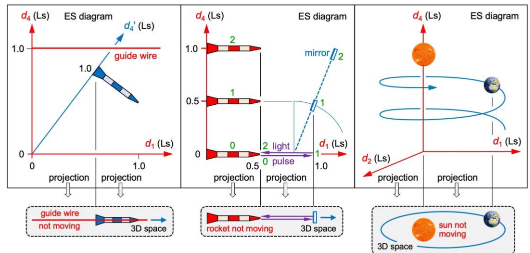
Fig. 4 Graphical solutions to three geometric paradoxes. Left: A rocket moves along a guide wire. In 3D space, the guide wire remains within the rocket. Center: An observer in a rocket tip tries to detect the reflection of a light pulse. Between two snapshots (0-1 or 1-2), rocket, mirror, and light pulse move 0.5 Ls in ES. In 3D space, the light pulse is reflected back to the observer. Right: Earth revolves around the sun. In 3D space, the sun remains in the orbital plane of Earth
