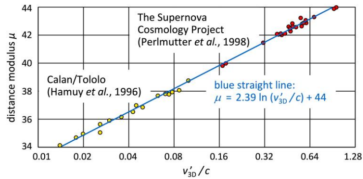
Fig. 6 Hubble diagram for 40 Type Ia supernovae. The horizontal axis displays adjusted speeds. All the data, including their uncertainties, are listed in the Appendix A
