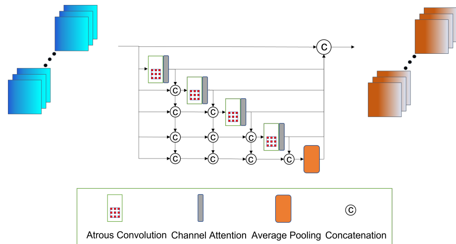
Figure 3. Channel-attention based densely connected Atrous spatial pyramid pooling (CADenseASPP). The Atrous convolution layers and a average pooling layer are densely connected, where a channel attention module is added just after each Atrous convolution layer.
