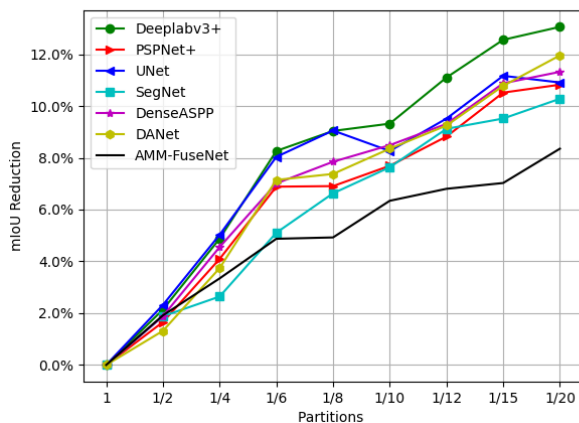
Figure 10. mIoU reduction on different partitions of the Potsdam data for each network
