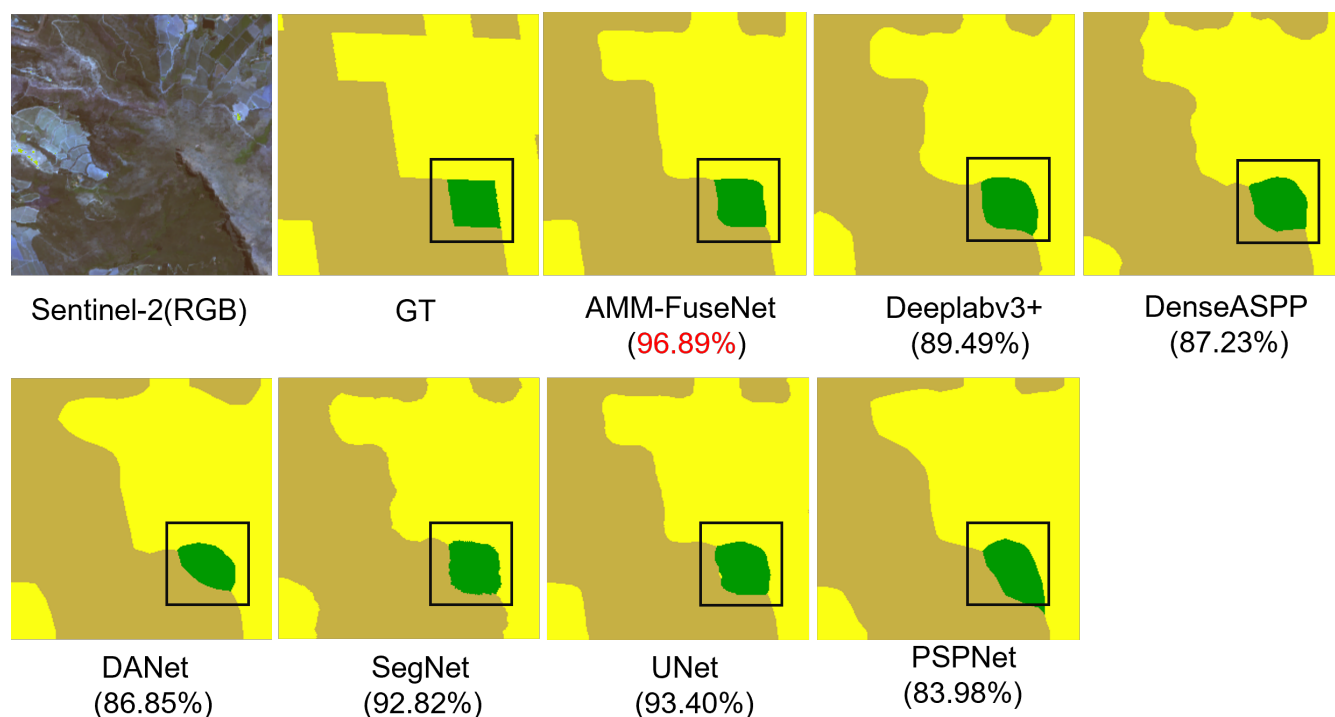
Figure 8. Results on DFC2020 dataset. Values between parentheses refer to mIoU in percentages for the example image for each model, where the best model is shown in a different colour.
