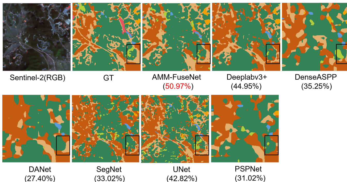
Figure 6. Results on Hunan dataset (Sentinel-2 & Sentinel-1). Values between parentheses refer to mIoU in percentages for the example image for each model, where the best model is in different colour.
