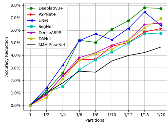
Figure 11. Accuracy reduction on different partitions of the Potsdam data for each network
