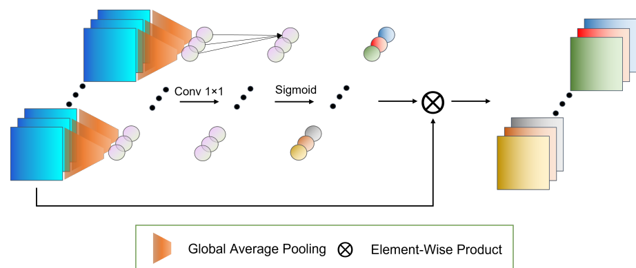
Figure 2. Visual representation of channel attention module (CA-Module). Aggregated features is processed by average pool to acquire element for each channel. Channel weights are obtain after 1-D convolution and Sigmoid function. Those channel weights and feature channels are matched in the figure by relevant colors.
