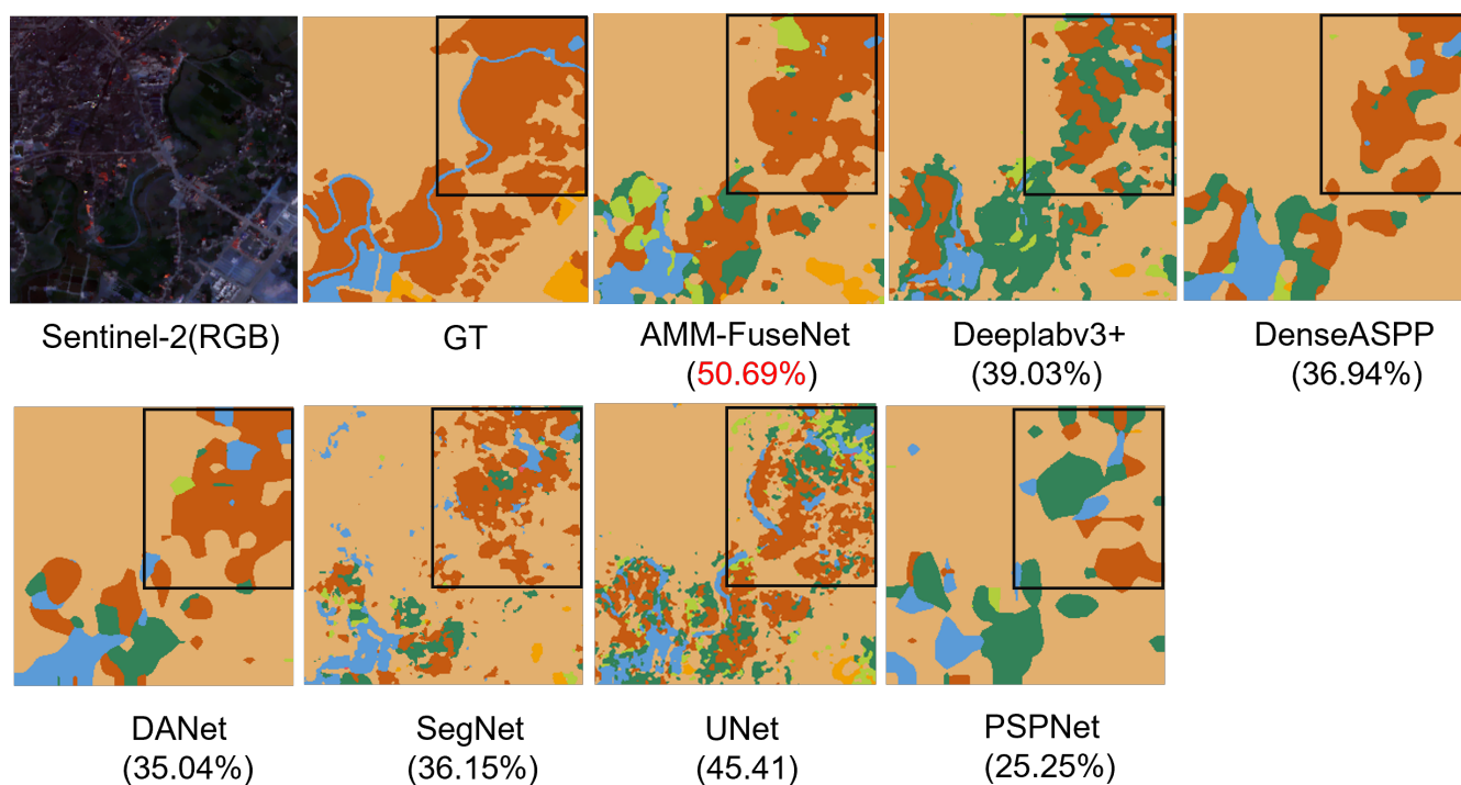
Figure 7. Results on Hunan dataset (Sentinel-2 & DEM) Values between parentheses refer to mIoU in percentages for the example image for each model, where the best model is in different colour.
