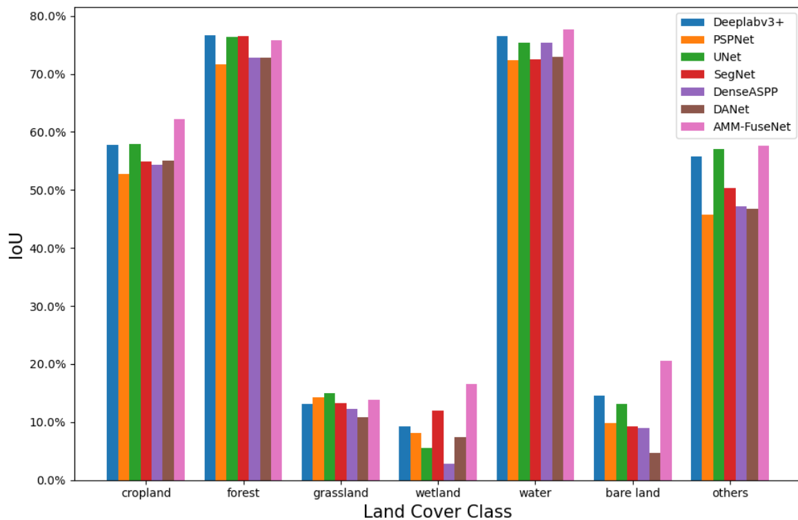
Figure 5. IoU of each land cover class on Hunan dataset (Sentinel-2 & Sentinel-1)
