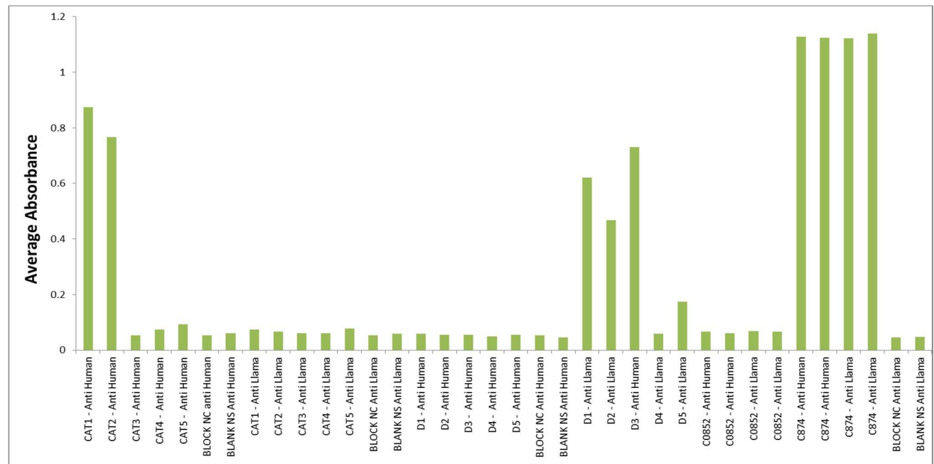
Figure 3: Bar graph showing positive cat, dogs and camel Sera detected either with Secondary second step anti-human IgG HRP or anti-Llama IgG HRP conjugated antibodies. The selected anti-human IgG conjugated with HRP can discriminate between positive sera (CAT1 & 2) and negative cat sera (CAT3, 4 & 5) samples, while anti-Llama IgG-conjugated HRP cannot discriminate between positives and negatives cats sera (D1, 2, 3 & 5). Anti-human IgG conjugated HRP does not detect Camel sera therefore doesn't distinguish between positive and negatives (C0852-Antihuman IgG HRP, C874 anti-Human) while anti-Llama IgG HRP does detect camel sera and can discriminate between a SARS CoV-2 positive sera (C874 –Anti-Llama IgG-HRP) from the negative sera (C0852-Anti-Llama IgG HRP)
