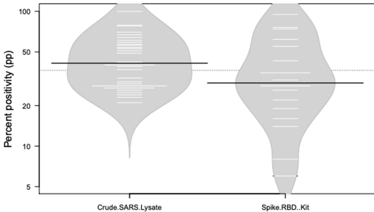
Figure 10: A comparison of the distribution of SARS CoV-2 like antibodies in camel sera determined both by a commercial kit (n=18) and by the crude lysate ELISA (n=32), and expressed as a percentage of the positive control serum (percent positivity). Black lines show the means; white lines represent individual data points; polygons represent the density of the data. The plot was generated using the R package beanplot (Kampastra 2009).
