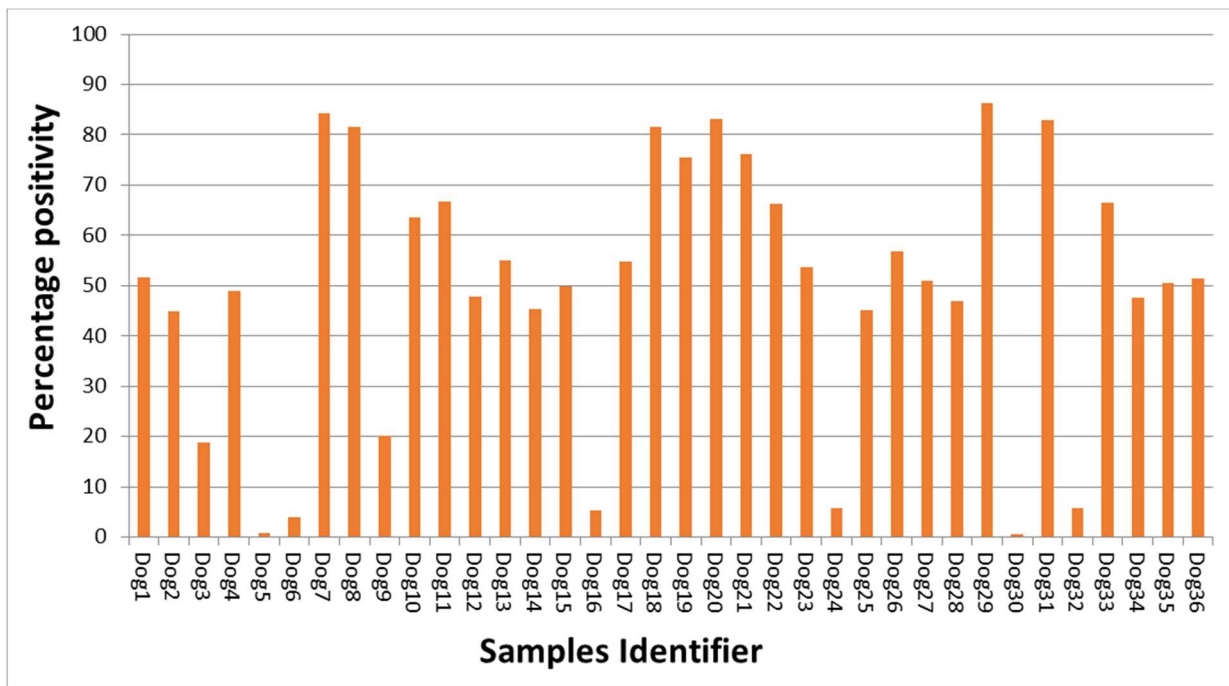
Figure 8: Screening of randomly selected Dogs Sera for the detection of SARS-CoV – 2 like antibodies. Sera dilution 1/50, (antigen at 5 \times 10^{-6} ). 15% PP cutoff: 83% exposure; 20%, cutoff point: 81% exposure to COVID-like antibodies
