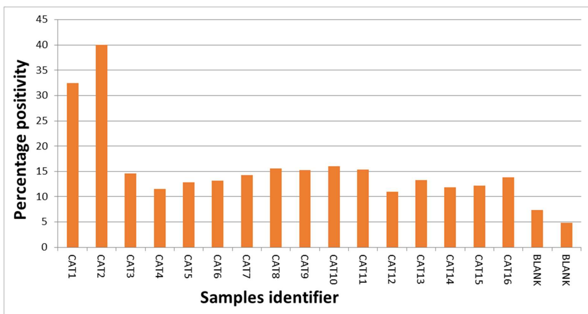
Figure 7: Screening of randomly selected Cats Sera for the Detection of SARS-CoV – 2 like antibodies. 1/50 sera dilution
