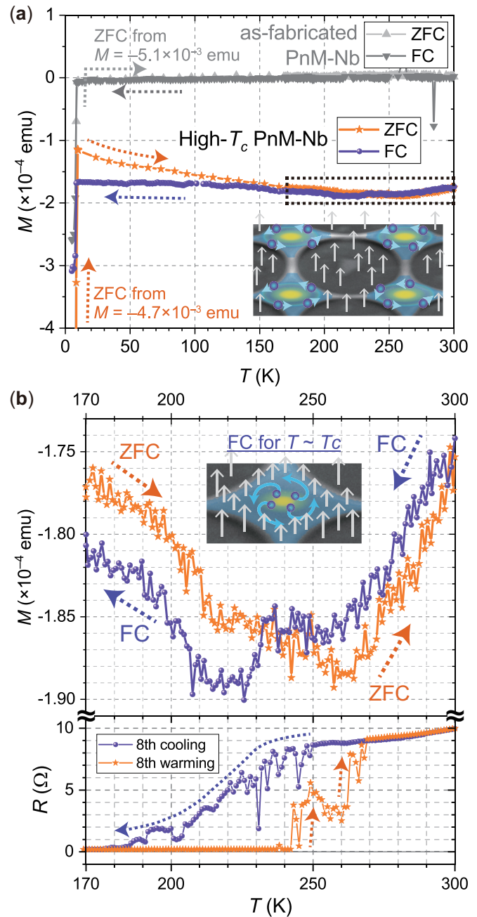
FIG. 5: Magnetic flux expulsion. (a) Magnetization versus temperature of an as-fabricated PnM-Nb sample (gray colors) and that of the PnM-Nb sample that exhibited high T_c 's in the preceding R - T measurement (orange and purple colors). Applied magnetic field for both the M - T measurements was 1000 Oe, perpendicular to the sample surface. (Inset) Schematic illustration of the PnM-Nb sample during the ZFC process for T < T_c using a false-color SEM. Out-of-plane gray arrows, applied magnetic flux. In-plane cyan arrows, circulating negative charge particles in the counterclockwise direction in such a way as to shield the interior of superconducting "islands" from the applied magnetic flux. (b) Enlarged M - T result in the temperature range of 170–300 K, surrounded by the black dotted square in (a). (Inset) Schematic illustration of the magnetic flux expulsion during the FC process, the Meissner effect. (Bottom panel) Duplicated R - T result of the eighth cycle in Fig. 4b, which was performed just before this M - T measurement.
