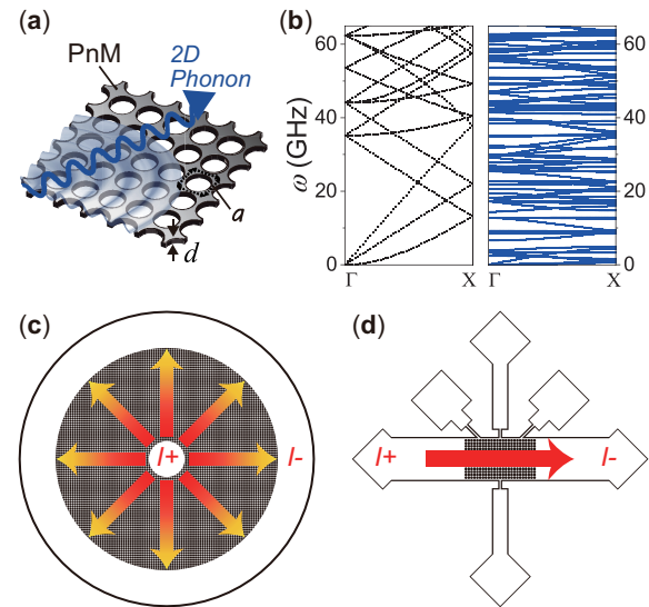
FIG. 1: Phonon engineered metallic system (PnM). (a) Schematic representation of a 2D PnM. The thickness and lattice constant is indicated by d and a , respectively. (b) Phonon dispersions of an Nb sheet with d of 150 nm. (Left) Without perforation. (Right) With periodic perforation designed as the PnM with a of 20 \mu\text{m} . (c) and (d) Bird's-eye view of the sample, respectively, used for the previous study 8 and for this study.
