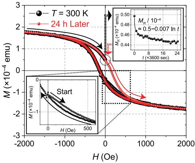
FIG. 6: Flux trapping at 300 K. Magnetic field dependence of magnetization of the PnM-Nb sample (black color) and that measured again 24 hours later (red color). Both were measured at 300 K.
