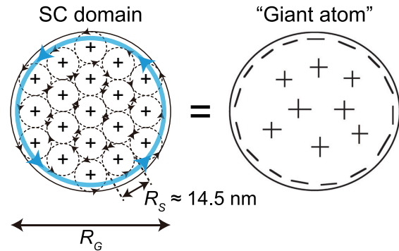
FIG. 8: Schematic superconducting (SC) domain with a diameter R_G , filled with Slater's atoms with the diameter R_S . Right panel, its superpositioned equivalent. "+" and "-" indicates a positive and negative charge, respectively. Cyan arrow, a screening current. The right panel is reprinted from ref. 22 , with the permission of AIP Publishing.
