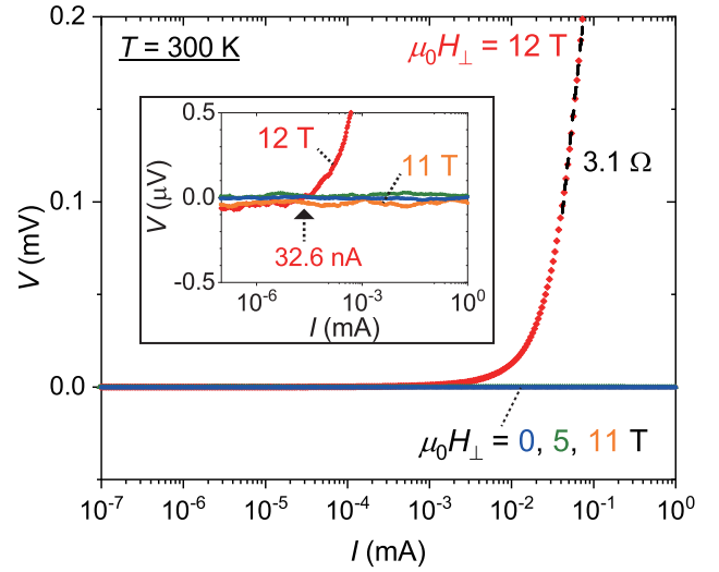
FIG. 7: Critical field at 300 K. Output voltage versus applied current under various magnitudes of perpendicular magnetic field, measured at 300 K. Inset, zoomed-in plot.
