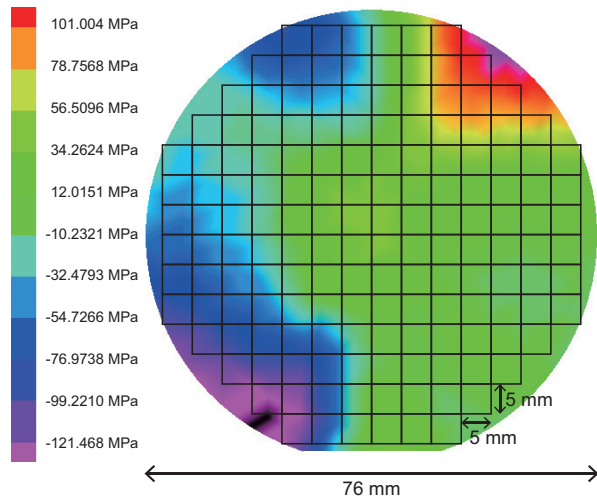
FIG. 9: In-plane stress of the Nb layer sputtered on the \text{SiO}_2/\text{Si} wafer with the diameter of 76 mm. The size of a sample chip ( 5 \times 5 \text{ mm}^2 ) is also indicated. The in-plane stress was measured using FSM 128NT (Frontier Semiconductor).
