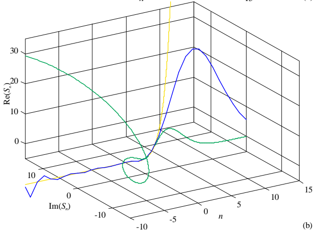
Fig. 7: Graphs of volumes (a, pink) and surface areas (b, blue) of n -balls of radius 1, along with volumes and surface areas of n -cubes circumscribed about (yellow) and inscribed in (green) these n -balls. In negative dimensions the latter are complex.
