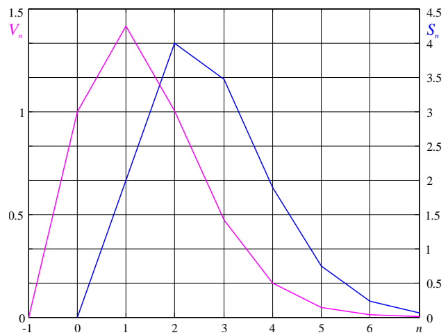
Fig. 6: Graphs of volumes ( V ) and surface areas ( S ) of n -orthoptices of unit edge length for n = -1, \dots, 7 .
