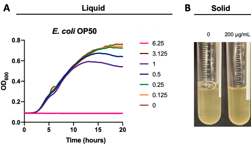
Supplemental Figure 2. The effect of gentamicin on E. coli OP50. A) Gentamicin dose-response in a plate dilution assay. Data represent three independent experiments, each in triplicates. B) Overnight cultures inoculated from bacteria plated on 0 and 200 µg/mL gentamicin.
