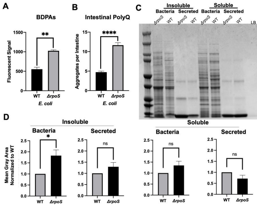
Figure 3. E. coli \Delta rpoS has increased levels of BDPAs and its colonization of the C. elegans intestine induces polyQ aggregation. A) ProteoStat assay quantification of total protein aggregates produced by E. coli wild-type (WT) and rpoS deletion ( \Delta rpoS ). Data are represented as the average ProteoStat fluorescent signal per bacterial strain. Each data point is an average of two independent experiments with three internal replicates per run. B) The effect of E. coli wild-type (WT) and rpoS deletion ( \Delta rpoS ) colonization of the C. elegans intestine on polyQ aggregation. Data are represented as the average number of polyQ aggregates per C. elegans intestine. C) An SDS-polyacrylamide gel electrophoresis of insoluble and soluble fractions from whole-cell lysate (Bacteria) and supernatant (Secreted) proteins. Image is representative of the results obtained from three independent experiments. Each data point is an average of three independent experiments with a minimum of 84 worms. The empty lane contains Lennox broth medium only (LB). D) Image-J (FIJI) quantification of proteins from (C). Data are representative of three independent experiments. A, B, D) Error bars represent SEM. Statistical significance was calculated using Student's t-test (* p < 0.05 , ** p < 0.01 , **** p < 0.0001 ).
