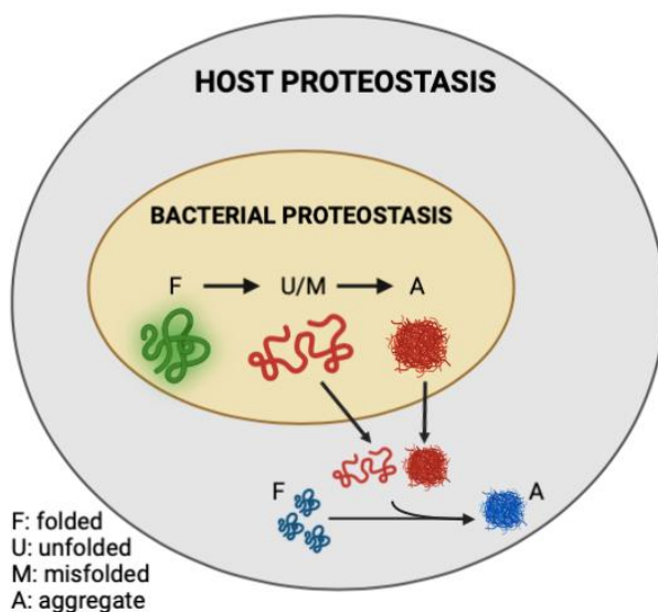
Figure 6. Model figure demonstrating the contribution of misfolded and aggregation-prone bacterial proteins to the disruption of host proteostasis.
