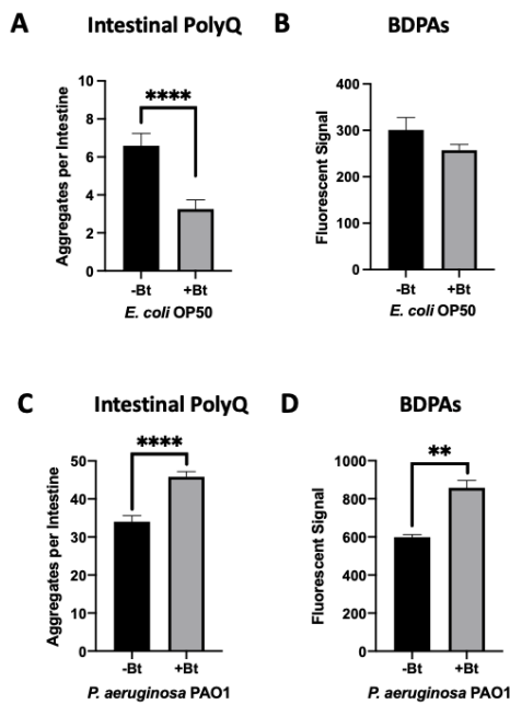
Figure 2. Low-concentration butyrate increases the abundance of P. aeruginosa BDPAs, which contributes to polyQ aggregation in C. elegans . The effect of A) E. coli OP50 and C) P. aeruginosa PAO1 colonization of the C. elegans intestine on polyQ aggregation in the absence (-Bt) and presence (+Bt) of 12.5 mM butyrate. Data are represented as the average number of polyQ aggregates per C. elegans intestine. Each data point is an average of three independent experiments with a total of 60 worms. ProteoStat assay quantification of total protein aggregates produced by B) E. coli OP50 and D) P. aeruginosa PAO1 in the absence (-Bt) and presence (+Bt) of butyrate. Data are represented as the average ProteoStat fluorescent signal per bacterial strain per treatment. Each data point is an average of two independent experiments with three replicates per run. A-D) Error bars represent SEM. Statistical significance was calculated using Student's t-test (** p < 0.01 , **** p < 0.0001 ).
