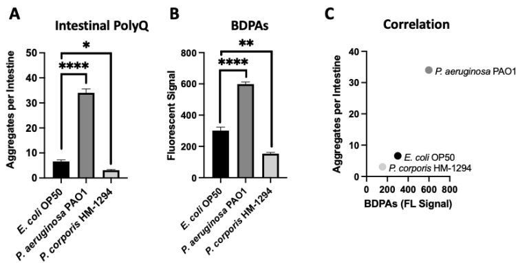
Figure 1. The extent of polyQ aggregation in the C. elegans gut upon bacterial colonization correlates with the relative abundance of BDPAs. A) The effect of P. aeruginosa PAO1 and P. corporis HM-1294 colonization of the C. elegans intestine on polyQ aggregation. Data are represented as the average number of polyQ aggregates per C. elegans intestine. Each data point is an average of three independent experiments with a total of 60 worms. B) ProteoStat assay quantification of total protein aggregates produced by E. coli OP50, P. aeruginosa PAO1, and P. corporis HM-1294. Data are represented as the average fluorescent signal per bacterial strain stained with ProteoStat. Each data point is an average of two independent experiments with three internal replicates per run. C) A positive correlation between the average number of polyQ aggregates and BDPAs. Error bars represent standard error of the mean (SEM). Statistical significance was calculated using one-way analysis of variance (ANOVA) followed by multiple comparison Dunnett's post-hoc test (* p < 0.05 , ** p < 0.01 , **** p < 0.0001 ).
