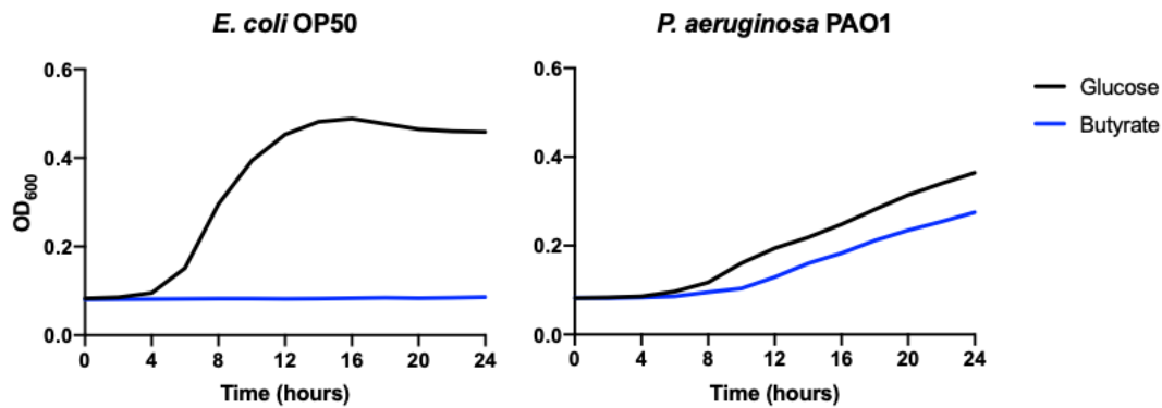
Supplemental Figure 1. Bacterial utilization of butyrate as energy source. Representative bacterial growth curves in M9 minimal medium supplemented with 0.2% glucose or butyrate as the sole carbon source. Data are representative of the average of two replicates. The experiment was performed three independent times.
