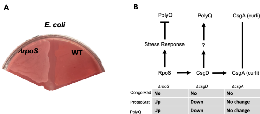
Figure 4. E. coli strain lacking RpoS induces polyQ aggregation through a mechanism independent of amyloid production. A) Congo Red staining of amyloids in E. coli lacking RpoS ( \Delta rpoS ) and wild-type (WT). B) A summary of the results indicating the absence of amyloids as assessed by the absence of Congo Red staining (No), change in the BDPAs assessed by the ProteoStat dye, and the effect on polyQ aggregation upon colonization of the C. elegans intestine. We previously showed that unknown product(s) (?) regulated by CsgD contributes to polyQ aggregation and that CsgA (major structural subunit of curli) had no effect on polyQ [12].
