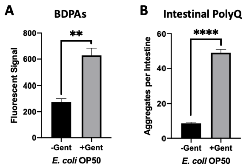
Figure 5. Gentamicin-induced disruption of bacterial proteostasis increases polyQ aggregation in the C. elegans intestine. A) ProteoStat assay quantification of total protein aggregates produced by E. coli OP50 in liquid culture in the absence (-Gent) or presence (+Gent) of 1 \mu\text{g}/\text{mL} gentamicin, a non-effective concentration (SFig 2A). Data are represented as the average ProteoStat fluorescent signal per bacterial strain per treatment. Each data point is an average of two independent experiments with three internal replicates per run. B) Intestinal polyQ aggregation in C. elegans colonized with E. coli OP50 in the absence (-Gent) or presence (+Gent) of 200 \mu\text{g}/\text{mL} , a sub-lethal concentration (SFig 2B). Data are represented as the average number of polyQ aggregates per C. elegans intestine. Each data point is an average of three independent experiments with a minimum of 90 worms. A-B) Error bars represent SEM. Statistical significance was calculated using Student's t-test (** p < 0.01 , **** p < 0.0001 ).
