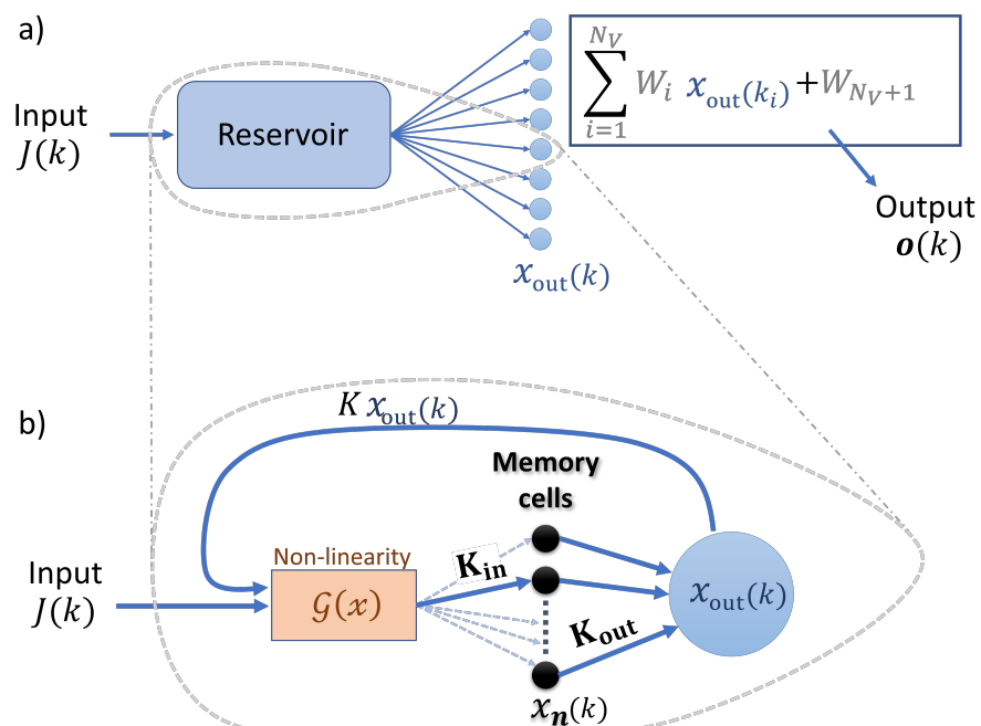
Figure 1. (a) Sketch of the reservoir computing concept. (b) Sketch of the memory cell reservoir described in Section 2.2.
