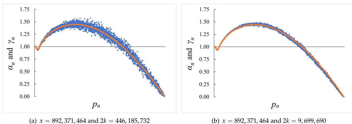
Figure 3. \alpha_n = \frac{|\mathcal{A}^{p_n}|}{|\mathcal{A}^{p_n}|} \cdot p_n (red) and \gamma_n = \begin{cases} \frac{1}{1} \cdot \frac{|\mathcal{C}^{p_n}|}{|\mathcal{C}^{p_n}|} \cdot p_n & \text{if } p_n \mid 2k, \\ \frac{1}{2} \cdot \frac{|\mathcal{C}^{p_n}|}{|\mathcal{C}^{p_n}|} \cdot p_n & \text{if } p_n \nmid 2k, \end{cases} (blue).
