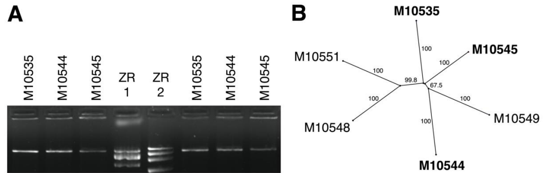
Figure 2. Characterisation of dsRNA extracted from Cryphonectria naterciae . (A) Agarose gel electrophoresis of dsRNA used for RNA-seq before (left) and after (right) DNase and S1 nuclease treatment. ZR1: 10, 5, 3kb; ZR2: 20, 7, 4, 2.5kb, Thermo Scientific ZipRuler Express DNA Ladder Set (SM1373). (B) Unrooted Neighbor Joining tree of a 958nt alignment including concatenated sequences of ORF1 and ORF2. Bold labels highlight strains associated with C. naterciae from Quercus suber , the others from Castanea sativa . Numbers represent bootstrapping rate of 1,000 replicates.
