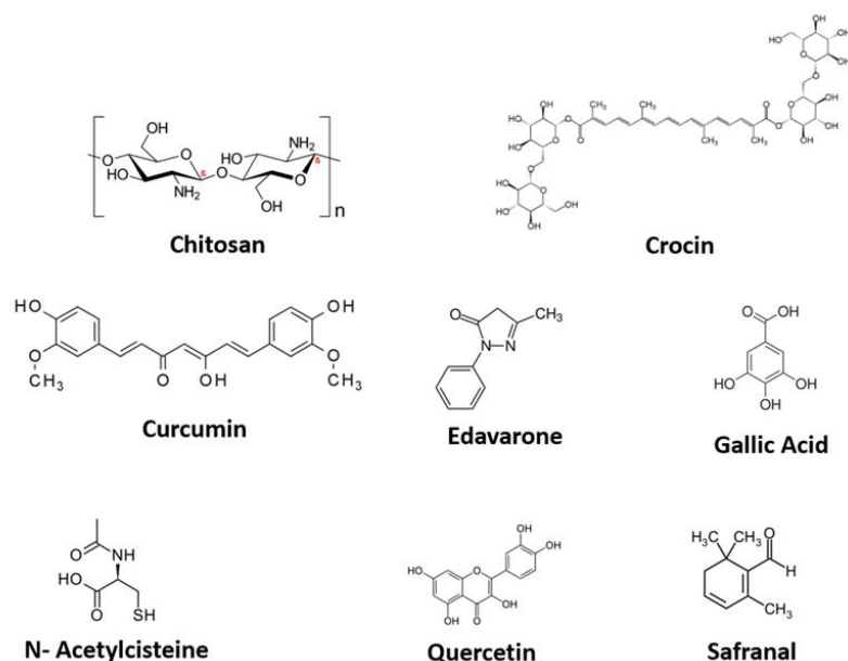
Figure 2. Chemical formula of the antioxidant substances.
