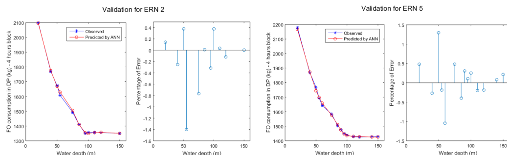
Figure 2. Comparison plot for observed and ANN predicted FO consumption values in DP assisted station keeping.
