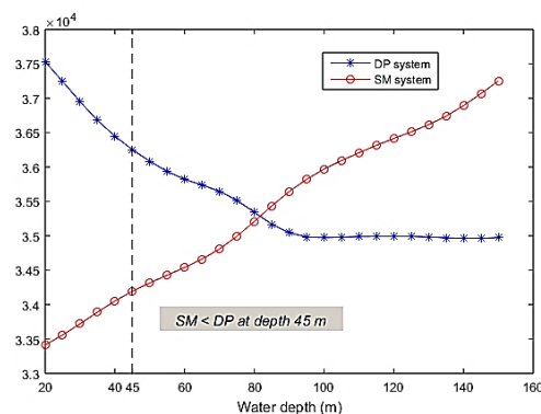
Figure 12. Decision making by ANNs based on total operational cost for the project specified in Table 11.
