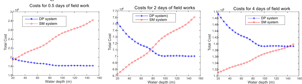
Figure 10. Cost comparison for different days of fieldwork in ERN 0 condition.
