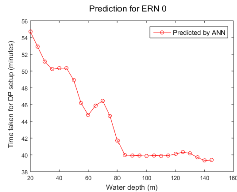
Figure 5. ANN-predicted DP setup time at ERN 0.
