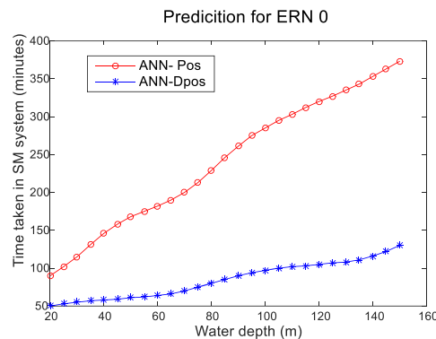
Figure 9. ANN-predicted SM set up and removal time at ERN 0.
