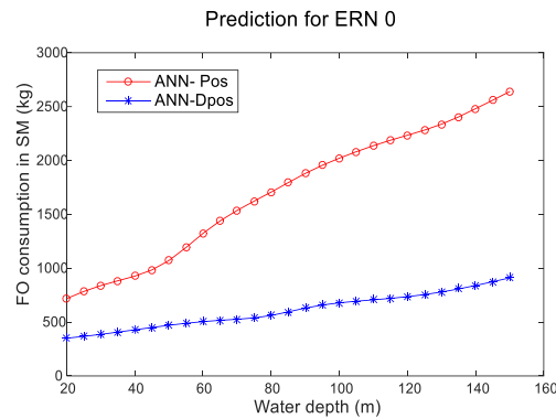
Figure 5. ANN-predicted FO consumption for the SM system.
