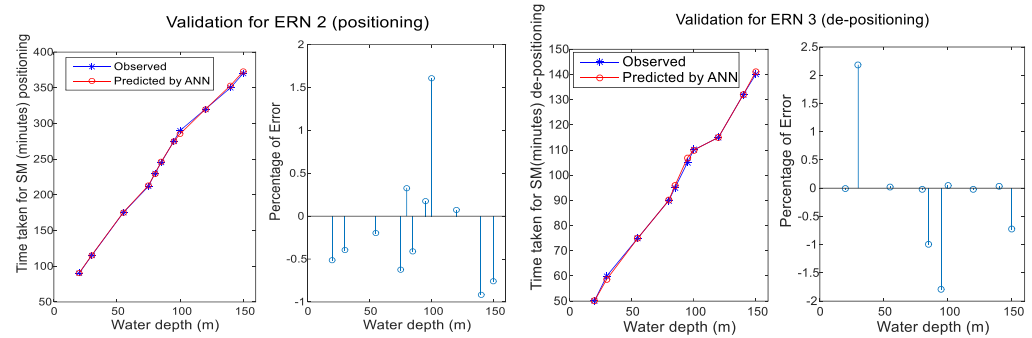
Figure 8. Comparison plot for observed and ANN predicted values (FO consumption for SM setup).
