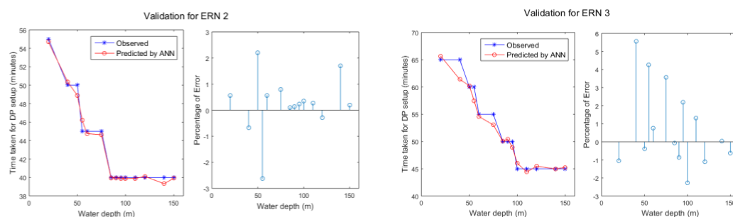
Figure 4. Comparison plot for observed and ANN predicted values (Time for DP setup).
