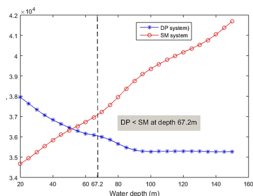
Figure 13. Decision making by ANNs based on total operational cost for the project specified in Table 12.
