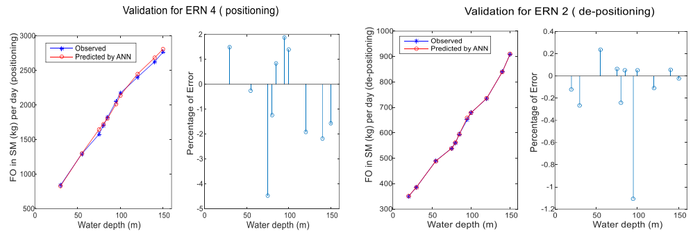
Figure 6. Comparison plot for observed and ANN predicted values (FO consumption for SM setup).
