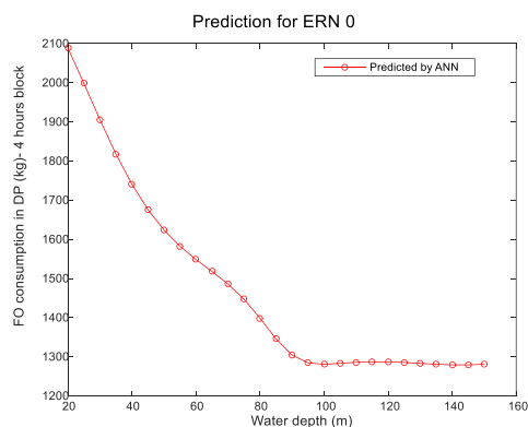
Figure 3. ANN-predicted FO consumption for ERN 0.
