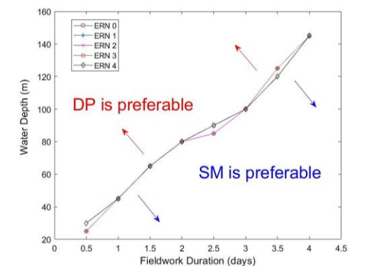
Figure 11. Decision-making plot for the geotechnical vessel with various ERNs.
