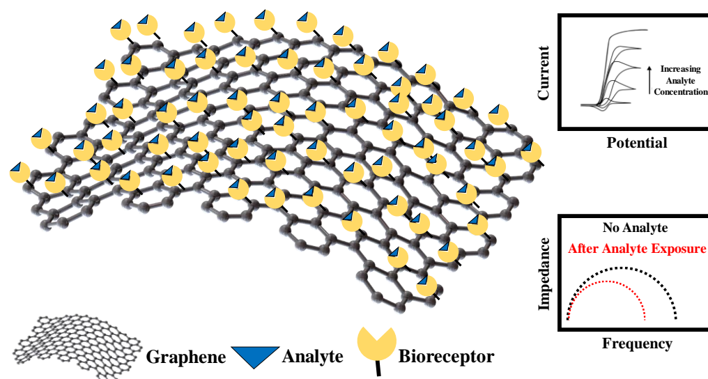
Fig. 6: Schematic showing analyte capture by appropriately functionalized graphene monolayer. The capture can be electrically measured by recording the impedance properties of the graphene layer, before and after analyte capture. Additionally, cyclic voltammetry measurements of the graphene layers display a change in I-V plots as a function of analyte concentration.
